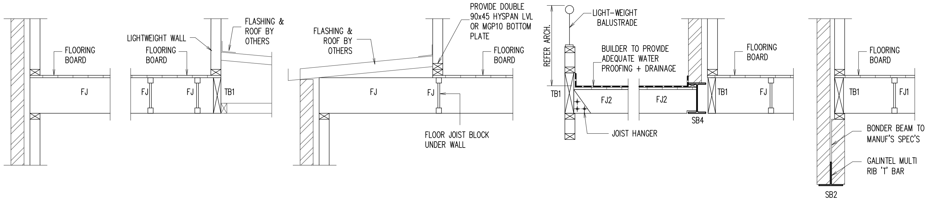
SECTION 1 SCALE 1:20
