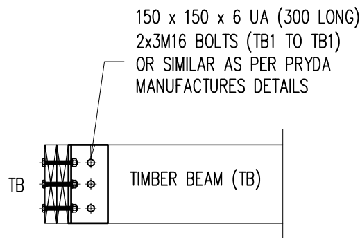
TYPICAL TIMBER BEAM (TB) TO TB DETAIL
