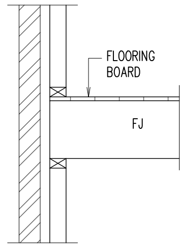
SECTION 1 SCALE 1:20
