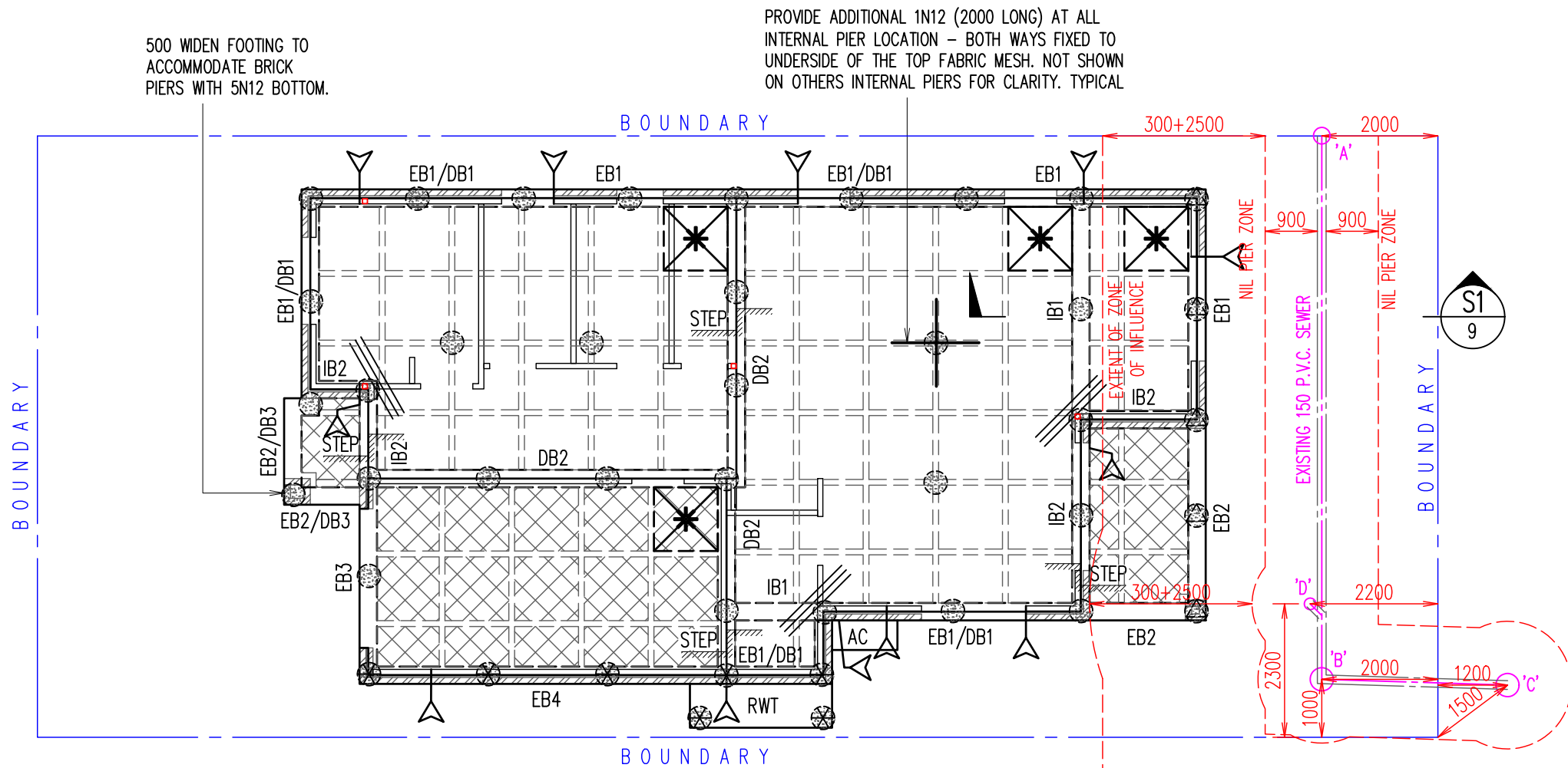
GROUND FLOOR WAFFLE SLAB LAYOUT PLAN SCALE 1:100
