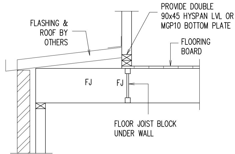
SECTION 3 SCALE 1:20
