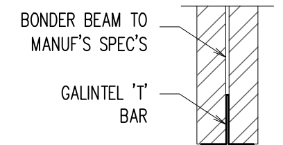
DETAIL -- A SCALE 1:20
