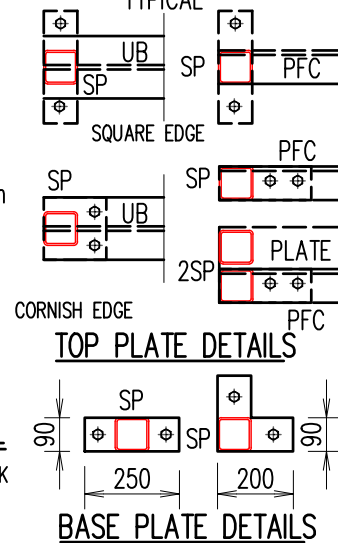
TYPICAL POST TO SLAB DETAIL
