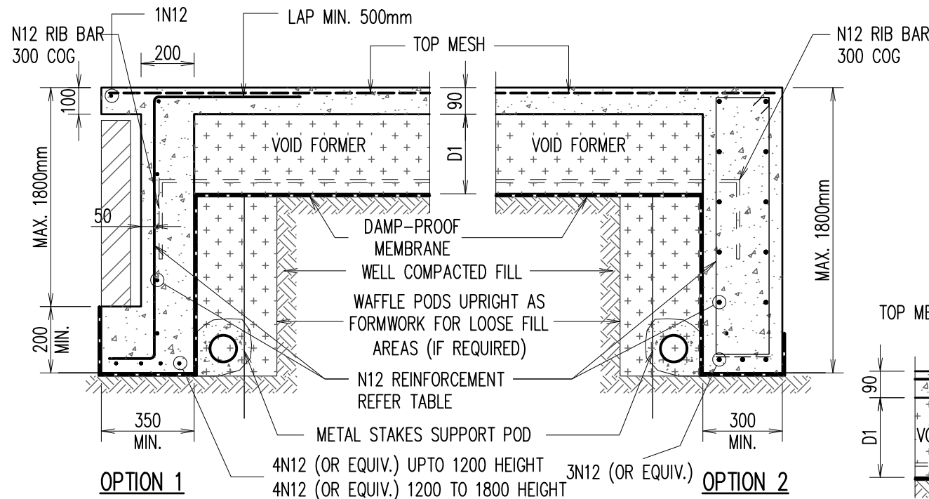
'EXTERNAL' DROP BEAM - 'DB3'
