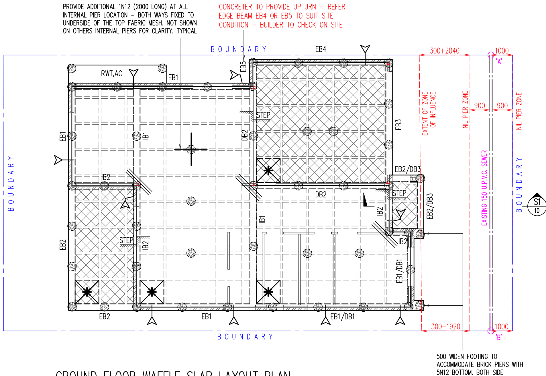
GROUND FLOOR WAFFLE SLAB LAYOUT PLAN SCALE 1:100
