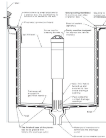
FIGURE 2.17 TYPICAL PLANTER BOX CONSTRUCTION
