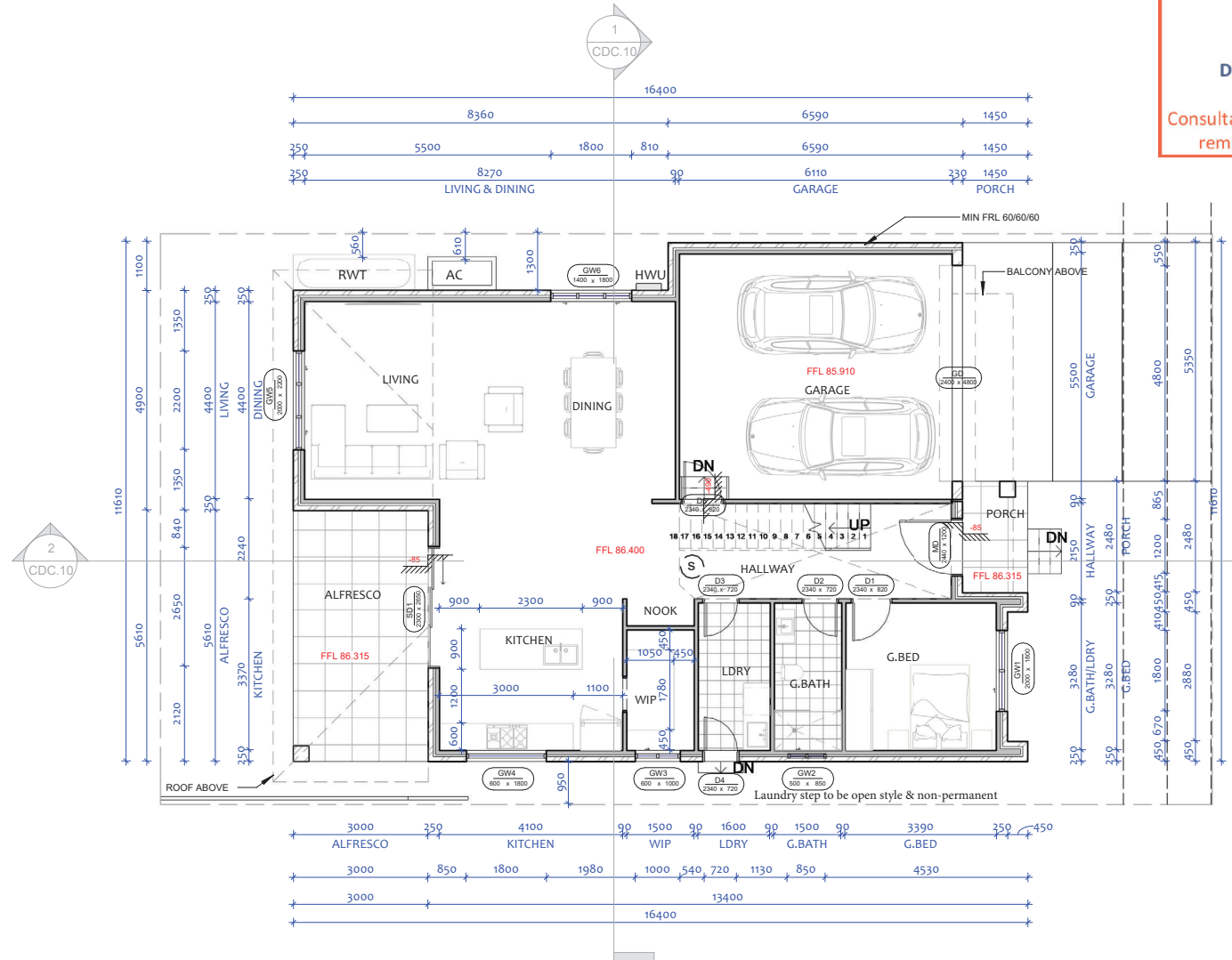
1 Ground Floor 1 : 100
