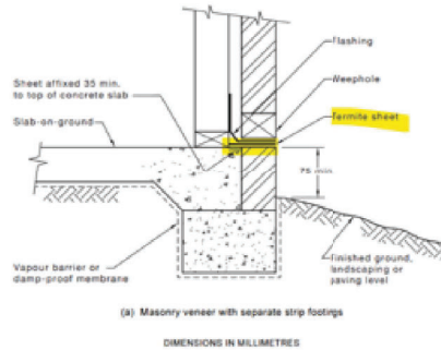
FIGURE 5.5 (in part) TYPICAL SHEET INSTALLATION TO EXTERNAL WALL WITH CONCRETE FLOOR SLAB
