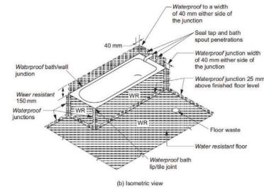
Figure 10.2.4b: Areas adjacent to baths and spas without showers for timber floors including particle-board, plywood and other floor materials
