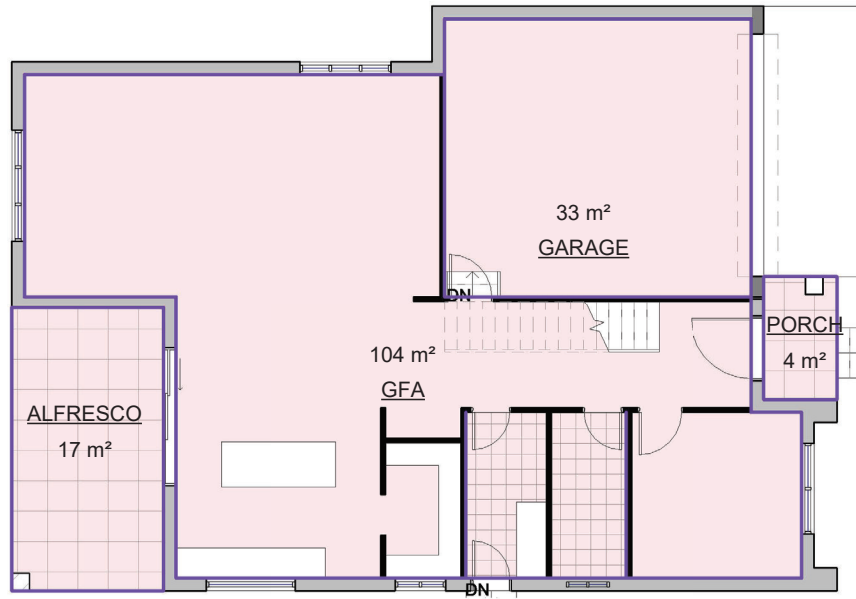
1 Ground Floor 1 : 100
