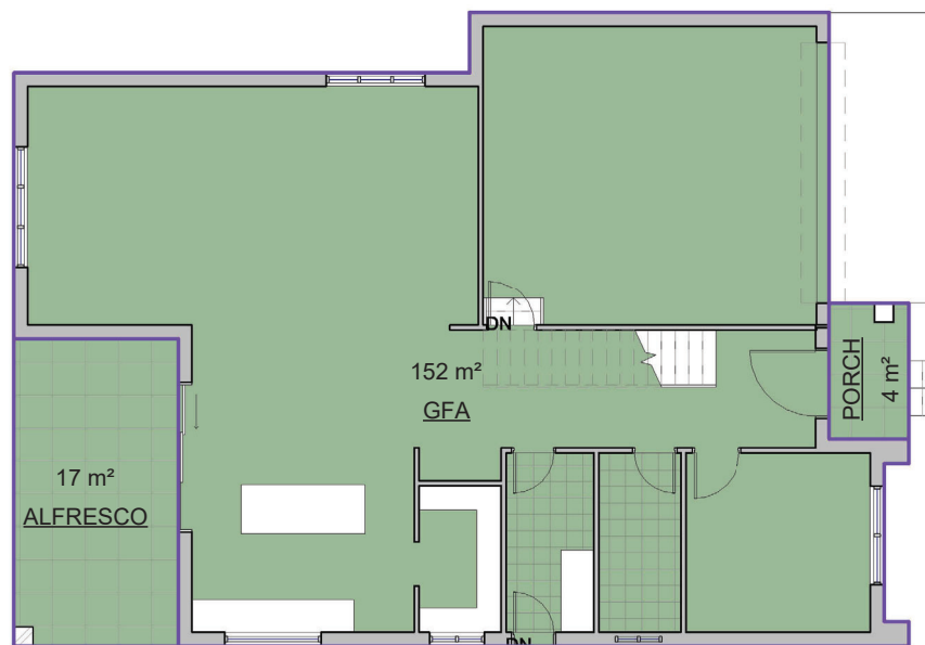
1 Ground Floor 1 : 100
