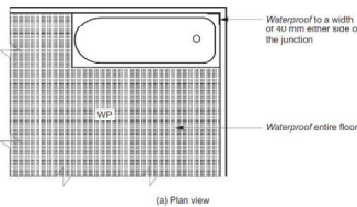
Figure 10.2.4b: Areas adjacent to baths and spas without showers for timber floors including particle-board, plywood and other floor materials
