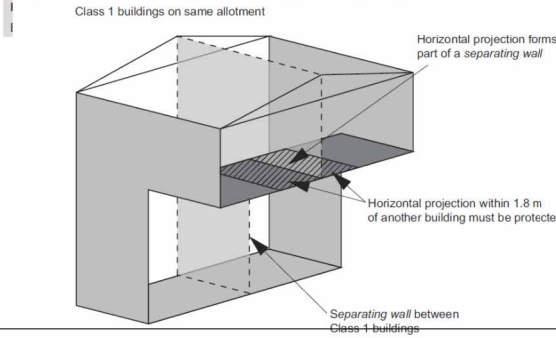
Figure 9.3.4: Horizontal projection forming part of a separating wall
