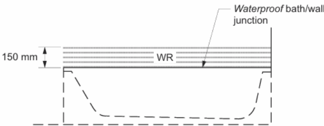
(b) Wall/bath junction
