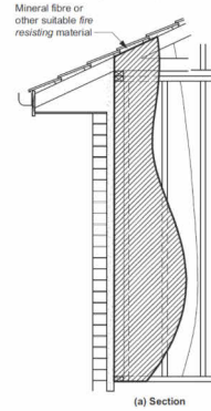
Figure 10.7.2a: Sound insulation between buildings — Stud wall junctions
