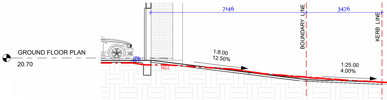
DRIVEWAY SECTION
