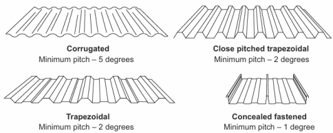
Minimum pitch requirements for metal roofing profiles
