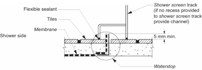
Figure 10.2.17: Typical hobless construction
