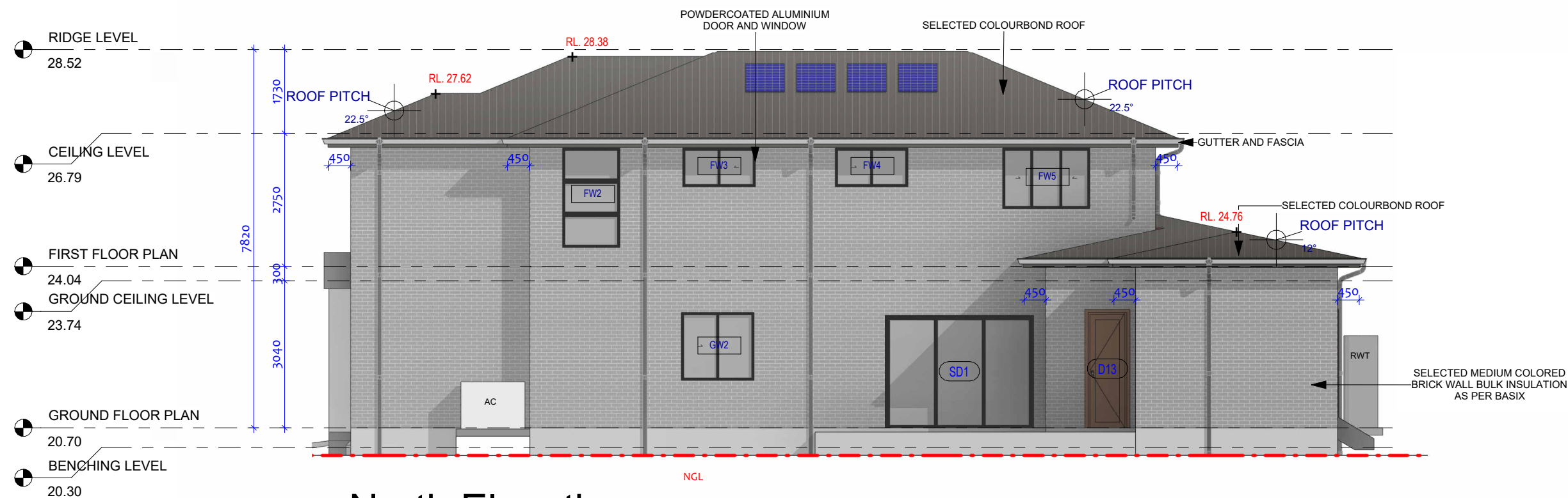
2 North Elevation 1 : 100
