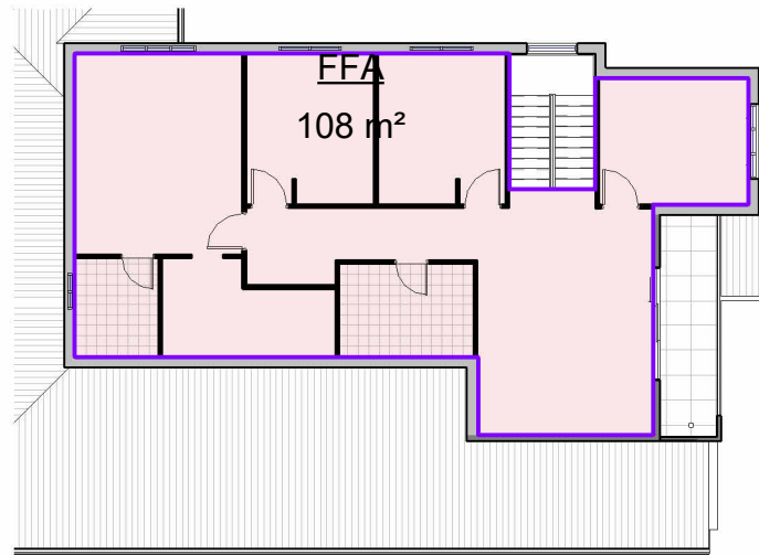
2 FIRST FLOOR PLAN 1 : 200
