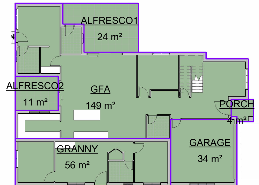
3 GROUND FLOOR PLAN 1 : 200
