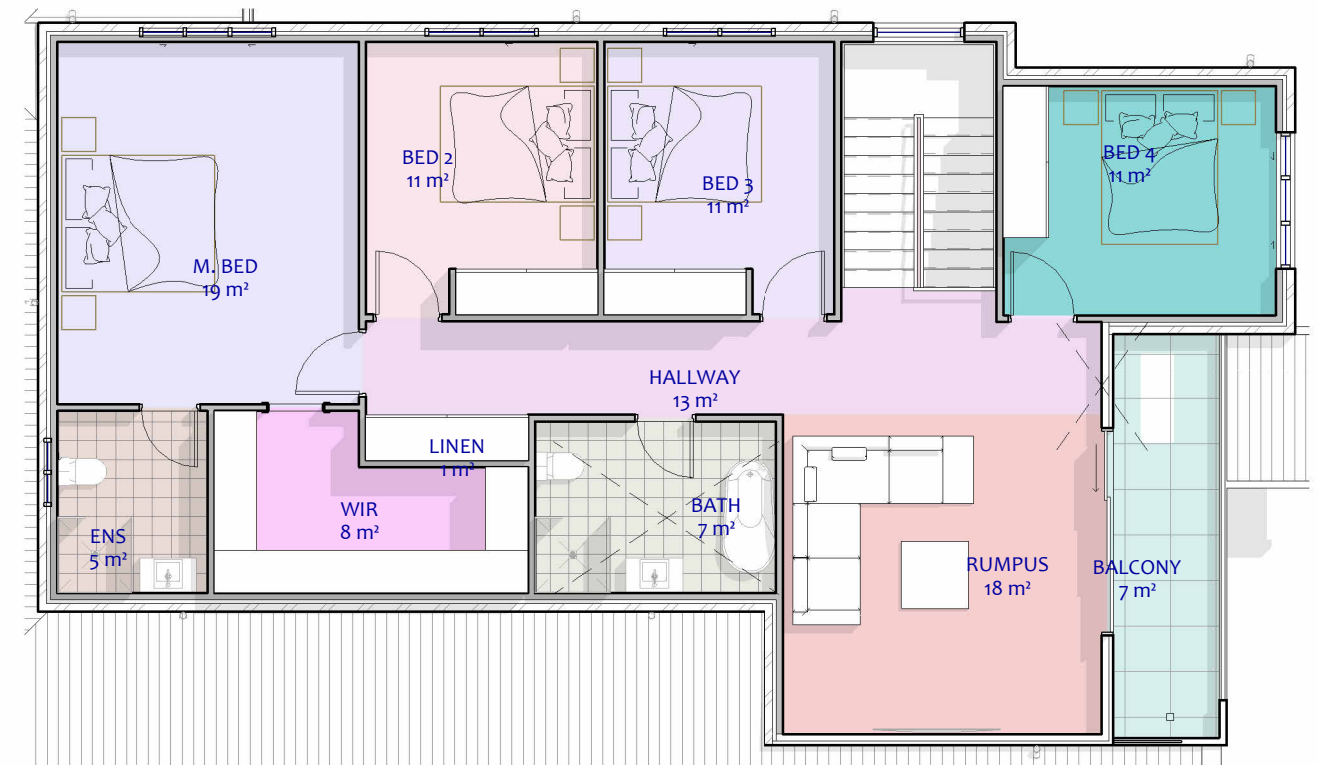
2 FIRST FLOOR ROOM AREA PLAN 1 : 100
