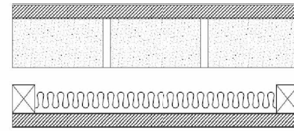
Figure 10.7.5c: Single leaf of 110 mm clay brick masonry
