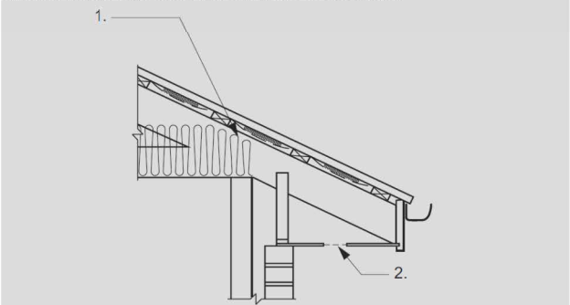
Figure 10.8.3 (explanatory): Example of roof space with low level ventilation
