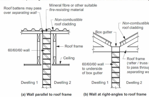
Figure 9.3.1c: Separating wall construction — Underside of non-combustible roof cladding (diagram 2)
