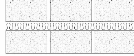
Figure 10.7.5b: Two leaves of 110 mm clay brick masonry (method 2)
