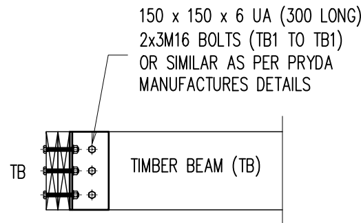
TYPICAL TIMBER BEAM (TB) TO TB DETAIL
