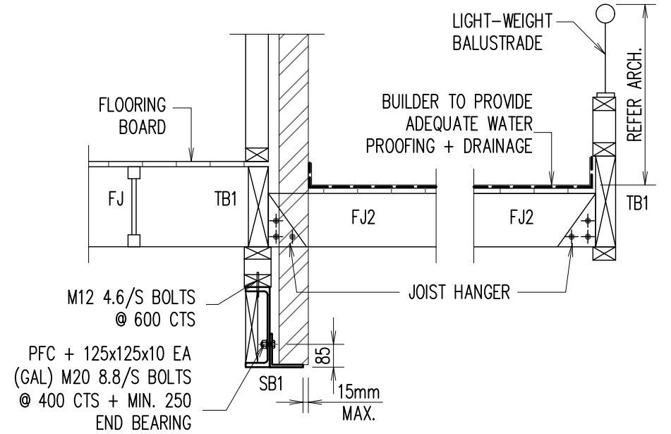
SECTION 4 SCALE 1:20
