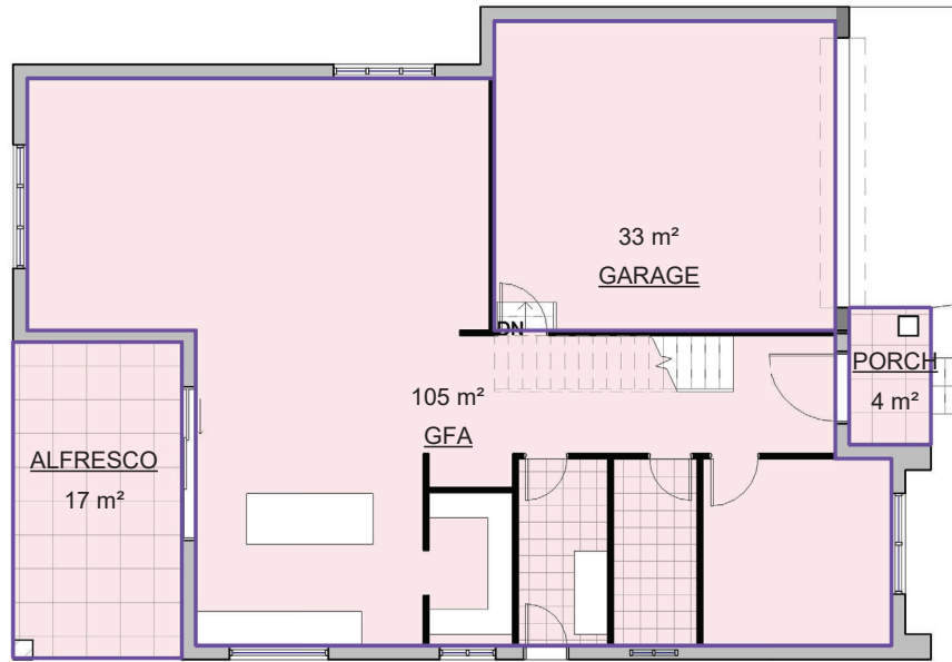
1 Ground Floor 1 : 100
