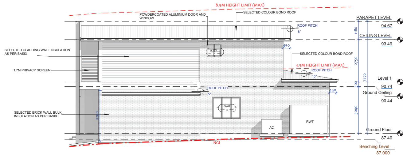
2 NORTH-EAST ELEVATION 1 : 100
