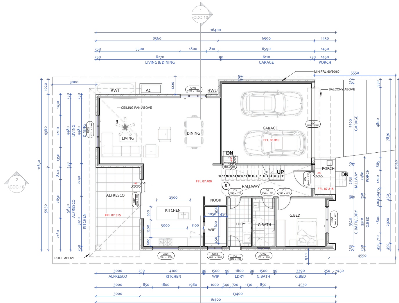
1 Ground Floor 1 : 100
