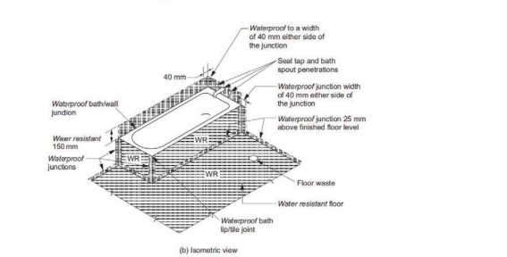
Figure 10.2.4b: Areas adjacent to baths and spas without showers for timber floors including particle-board, plywood and other floor materials
