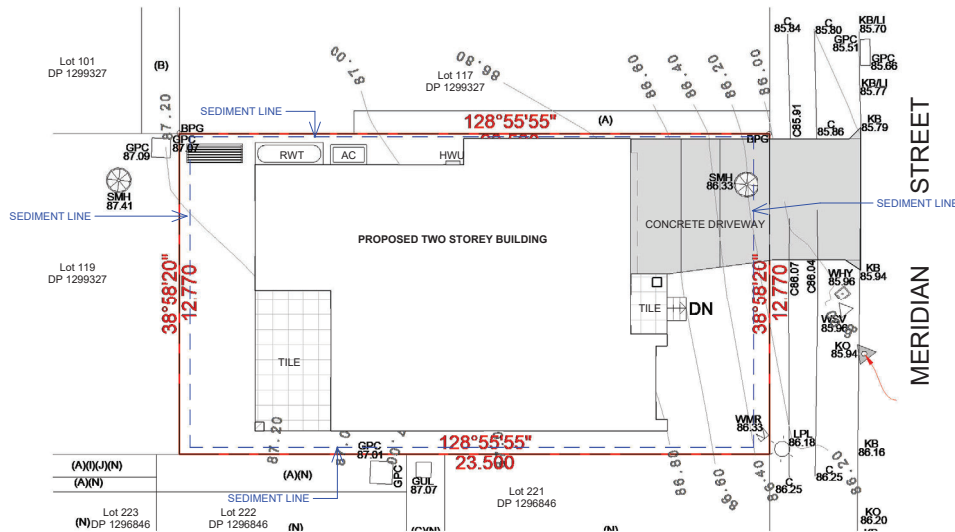
1 CDC - SITE ANALYSIS AND SEDIMENT CONTROL 1 : 200
