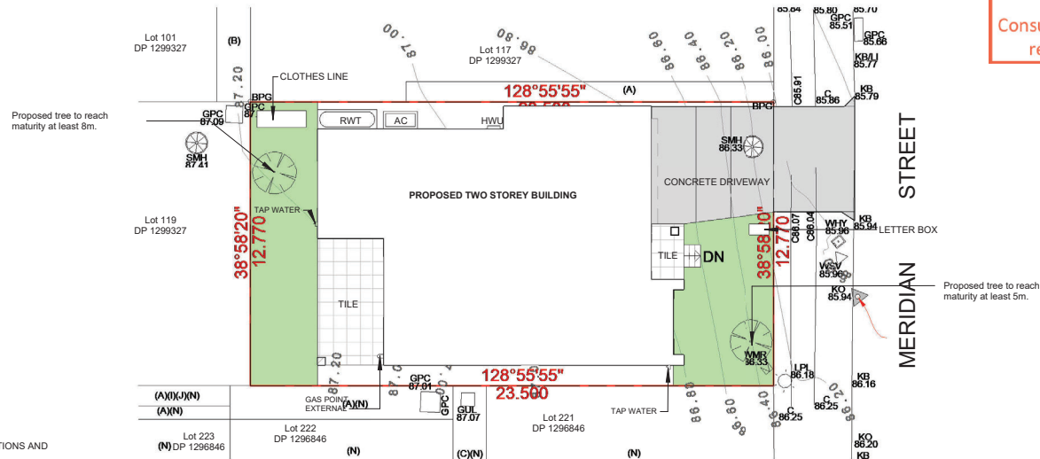
CDC - LANDSCAPE PLAN
