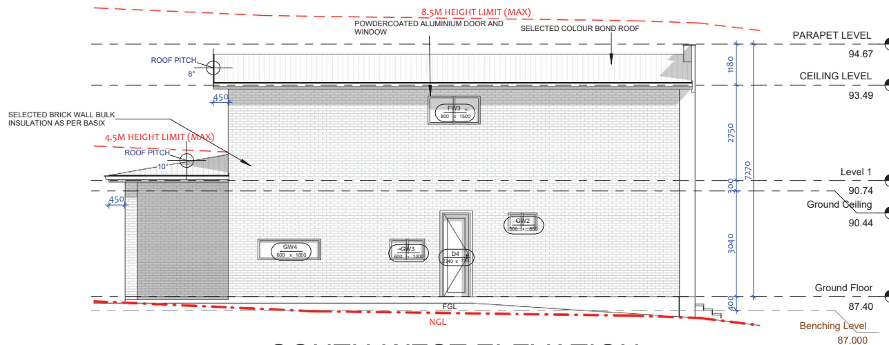
1 SOUTH-WEST ELEVATION 1 : 100
