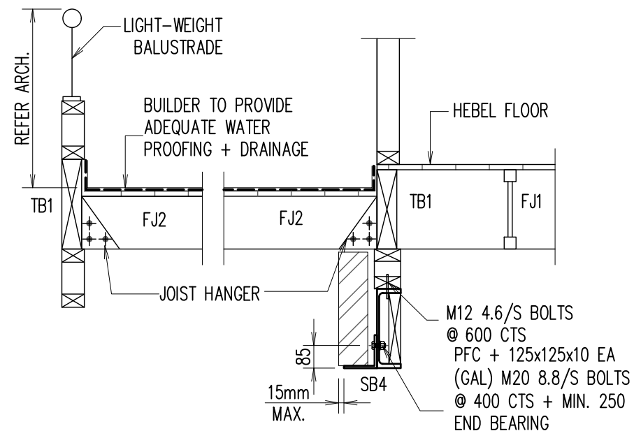
SECTION 4 SCALE 1:20
