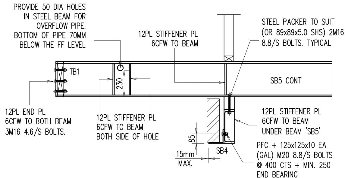
DETAIL – C SCALE 1:20
