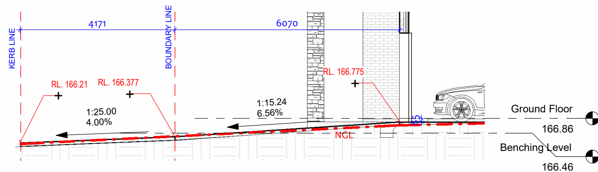
2 DRIVEWAY SECTION 1 : 100
