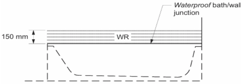
(b) Wall/bath junction
