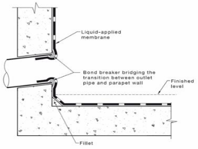
(a) Overflow through parapet
