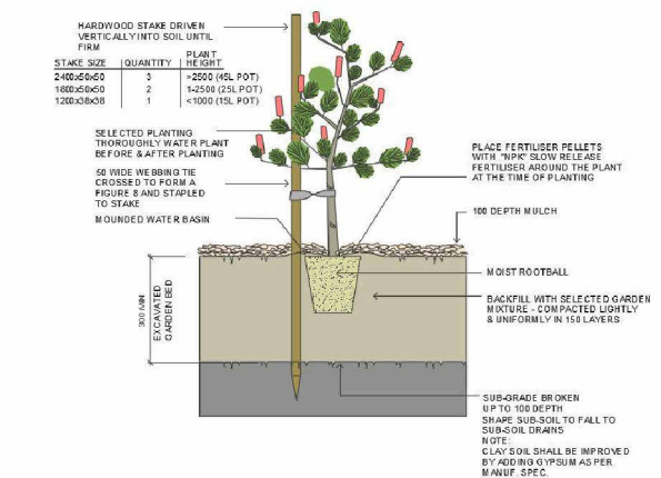
2. TREE & SHRUB PLANTING IN GARDEN BED
