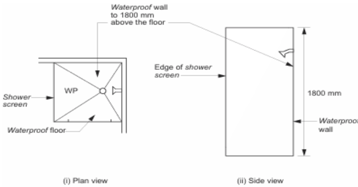
(a) Enclosed shower
