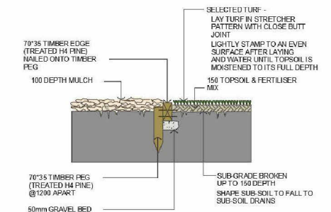
1. TURF & GARDEN EDGE DETAIL
