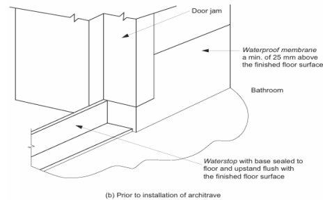
(b) Prior to installation of architrave
