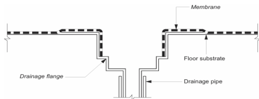
Figure 10.2.29: Typical membrane termination at drainage outlet
