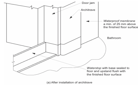
(a) After installation of architrave
