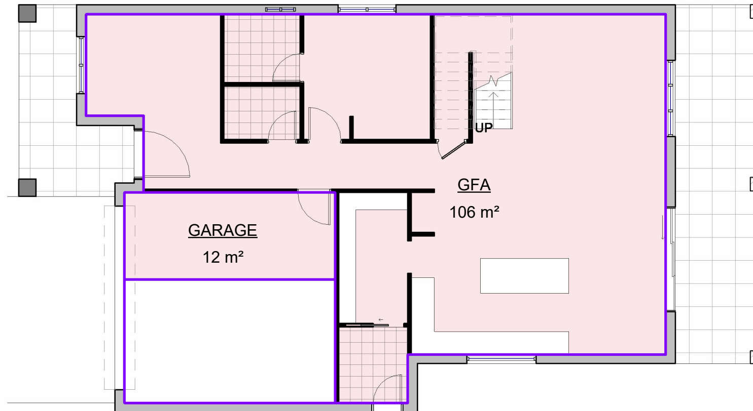
1 Ground Floor 1 : 100
