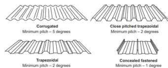
Figure 7.2.3: Minimum pitch requirements for metal roofing profiles
