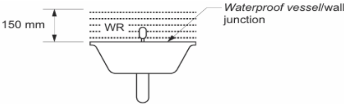
(a) Vessel abutting wall
