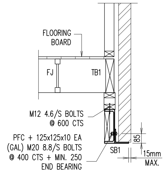
SECTION 4 SCALE 1:20
