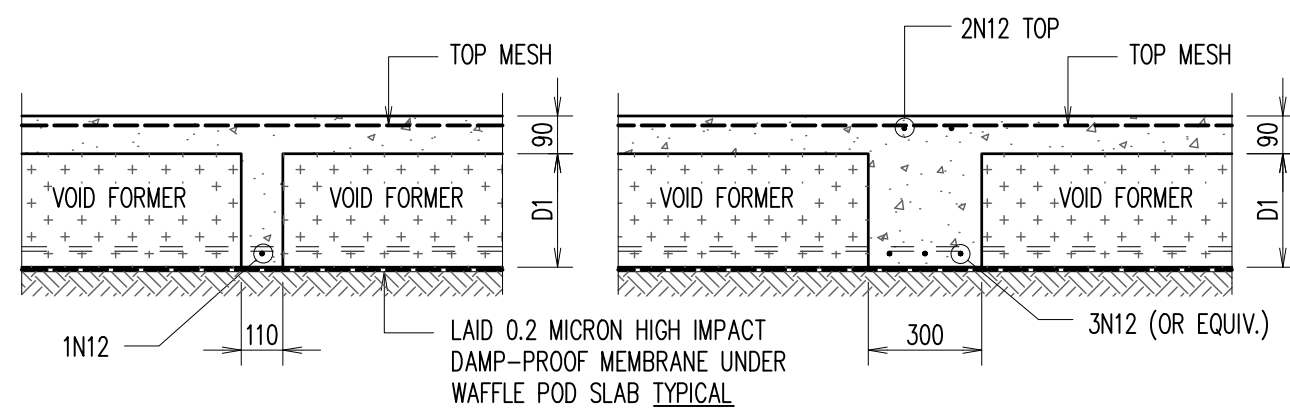
INTERNAL RIB
