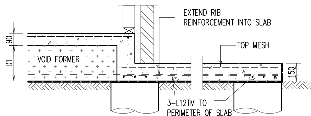
TYPICAL ATTACHED TANK/AC SLAB DETAIL
