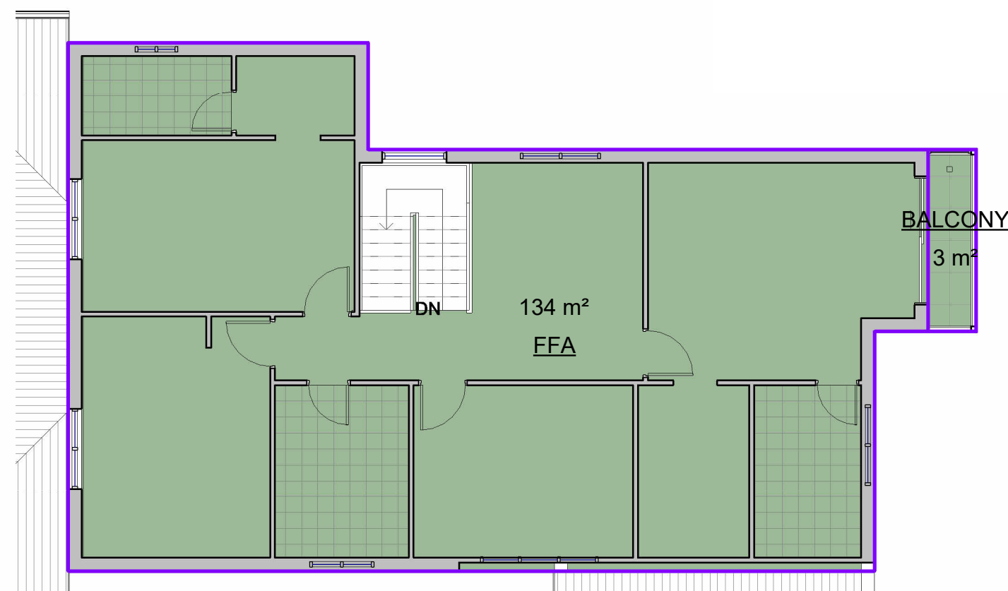
Level 1
