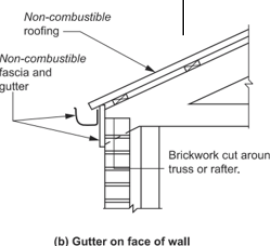
(b) Gutter on face of wall
