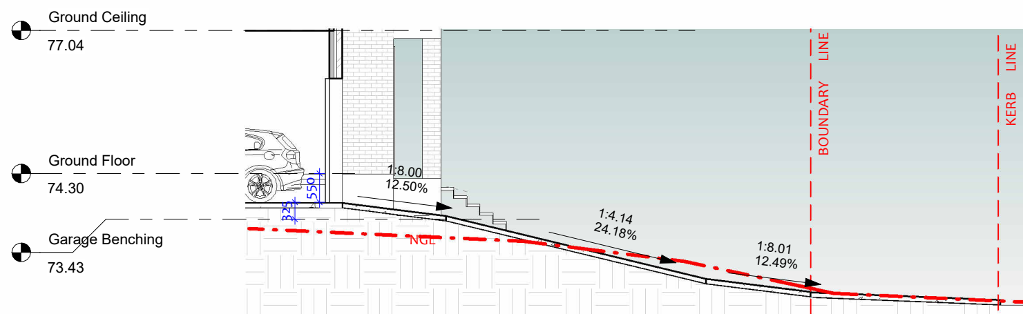
DRIVEWAY SECTION
