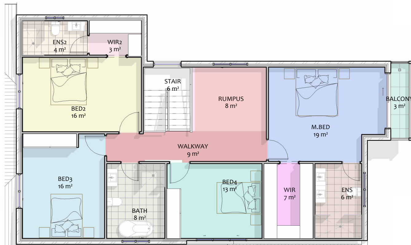
Level 1 Room Area Plan
