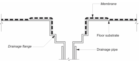
Figure 10.2.29: Typical membrane termination at drainage outlet
