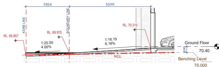
2 DRIVEWAY SECTION 1 : 100
