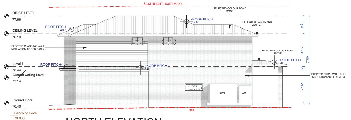
2 NORTH ELEVATION 1 : 100
