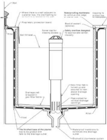
FIGURE 2.17 TYPICAL PLANTER BOX CONSTRUCTION
