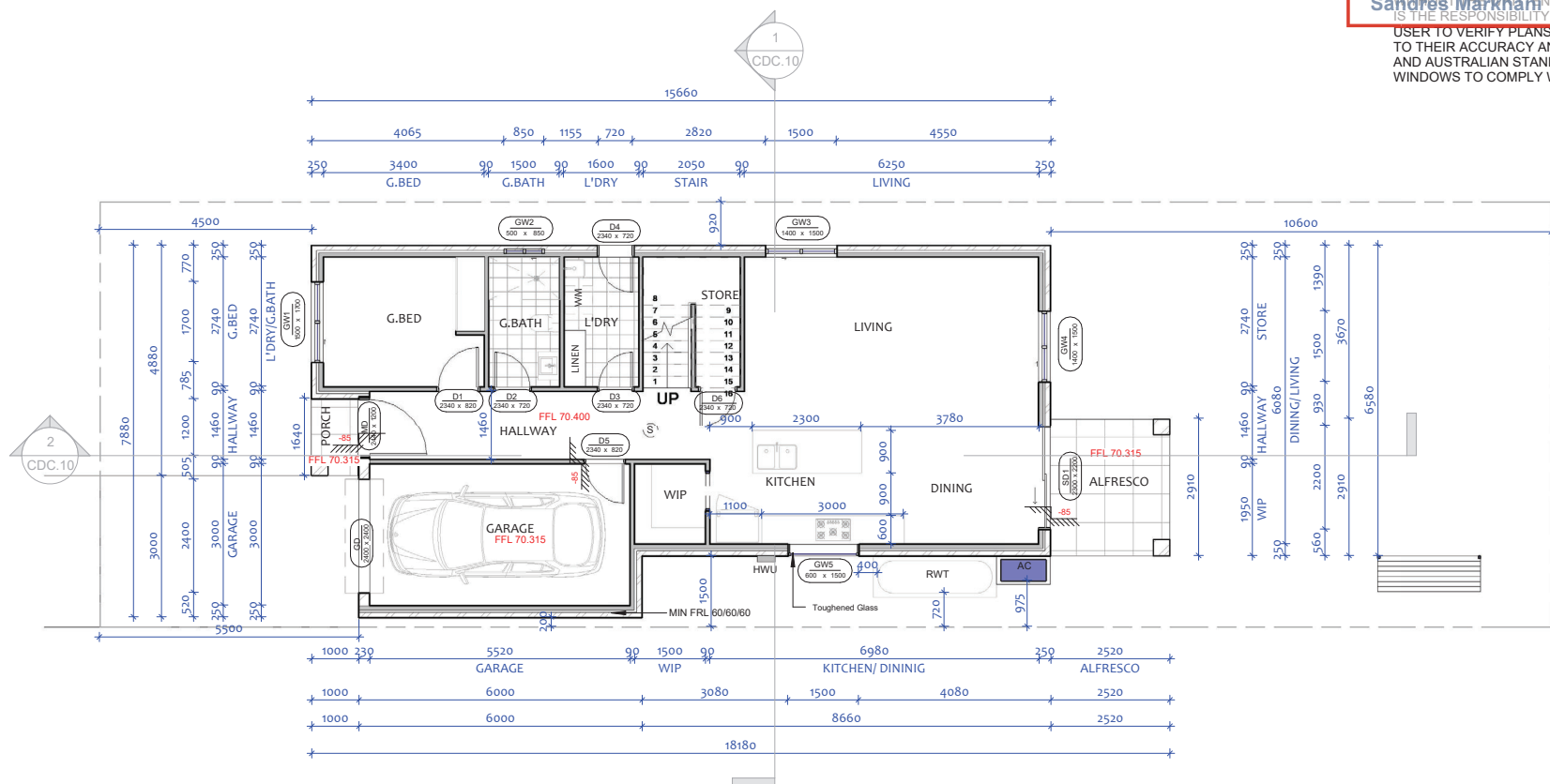
1 Ground Floor 1 : 100
