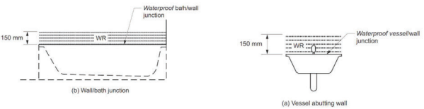
Figure 10.2.5: Bath and vessel abutting wall - areas to be protected
