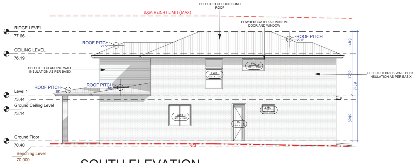
1 SOUTH ELEVATION 1 : 100
