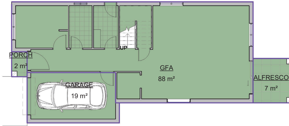
1 Ground Floor 1 : 100
