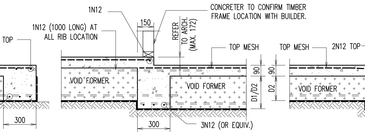
INTERNAL STEPDOWN BEAM – 'IB3'
