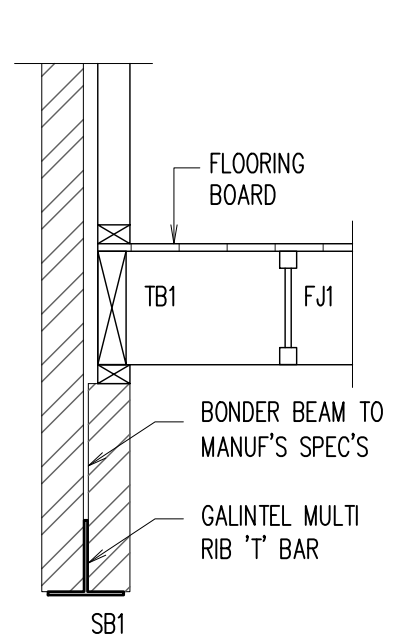
SECTION 5 SCALE 1:20
