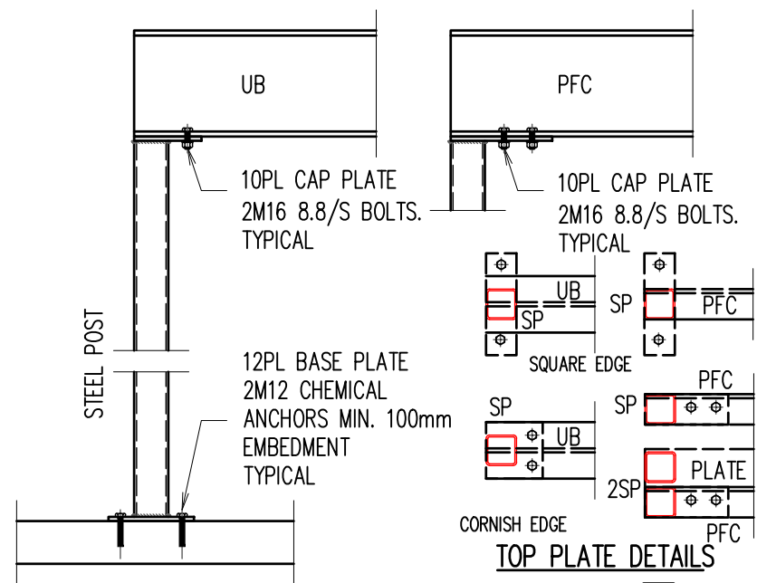
TYPICAL POST TO SLAB DETAIL NOTE: POSTS TO BE SECURELY BRACED TO STUD FRAMEWORK
