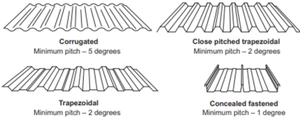
Figure 7.2.3: Minimum pitch requirements for metal roofing profiles
