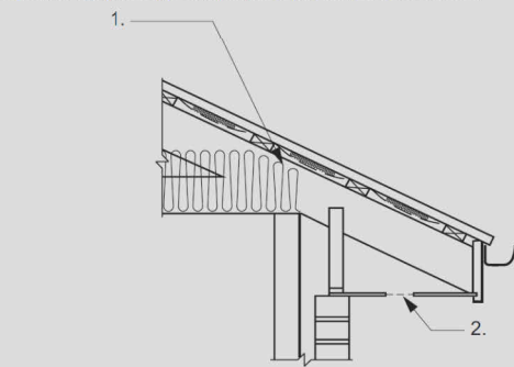
Figure 10.8.3 (explanatory): Example of roof space with low level ventilation
