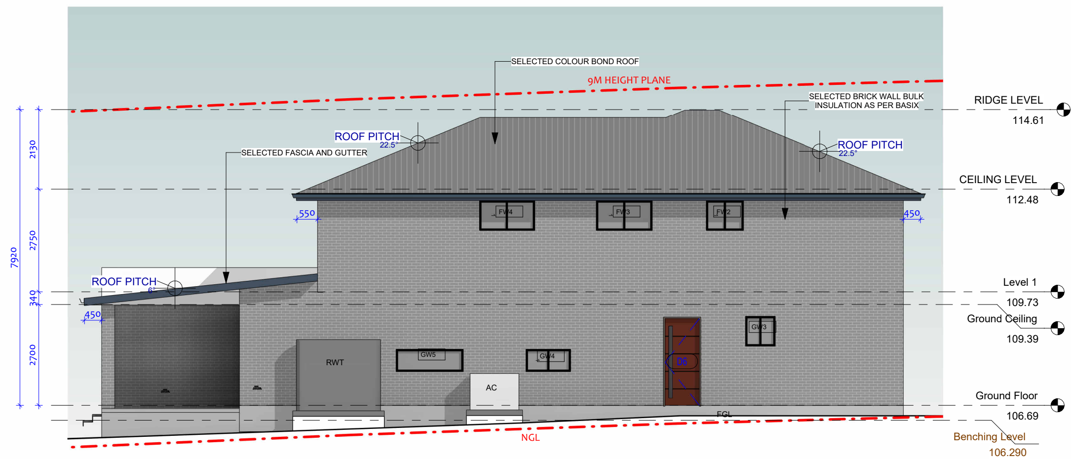
2 South- West Elevation 1 : 100
