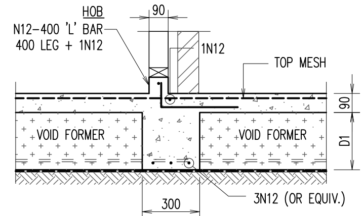
INTERNAL BEAM – 'IB4'
