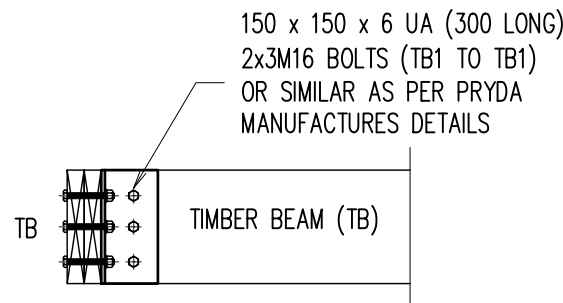
TYPICAL TIMBER BEAM (TB) TO TB DETAIL
