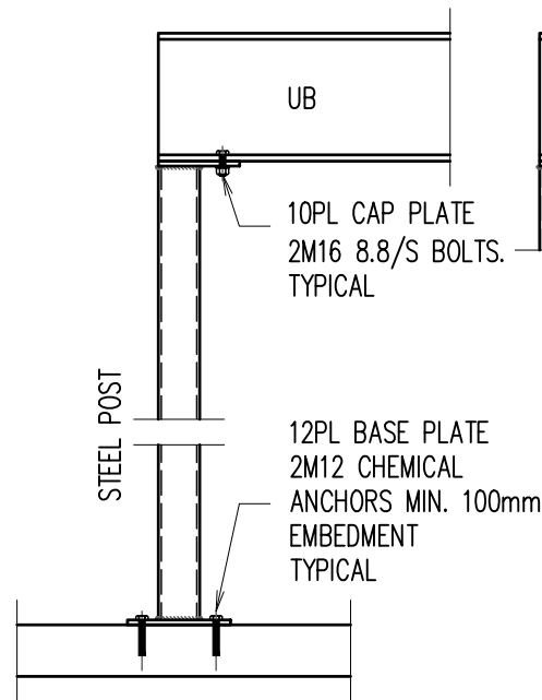
TYPICAL POST TO SLAB DETAIL
