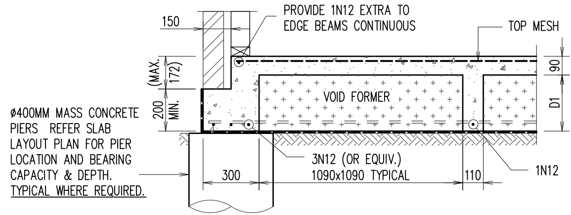
TYPICAL EDGE BEAM – 'EB1' ALTERNATIVELY REFER TO 'DB1' FOR DETAILS
