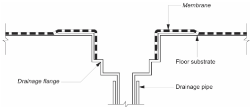
Figure 10.2.29: Typical membrane termination at drainage outlet
