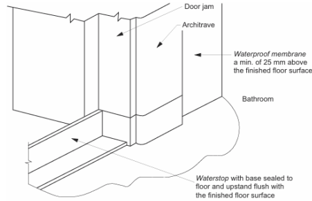
(a) After installation of architrave
