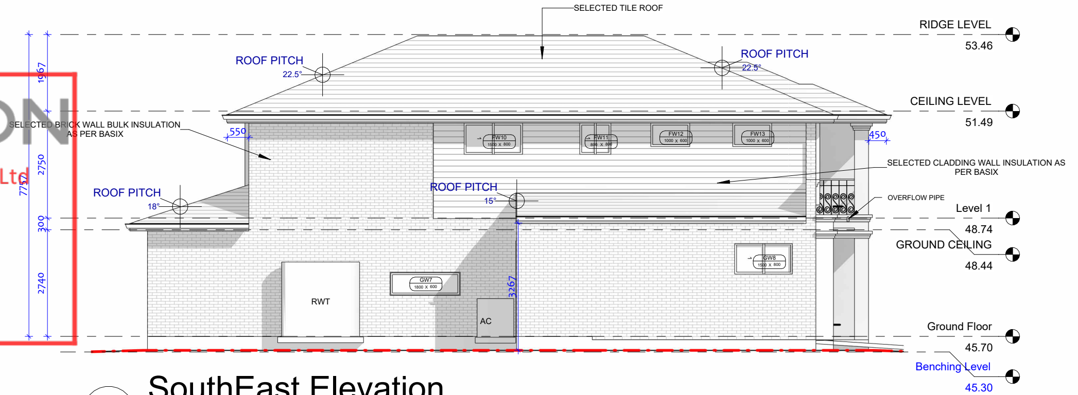
1 SouthEast Elevation 1 : 100
