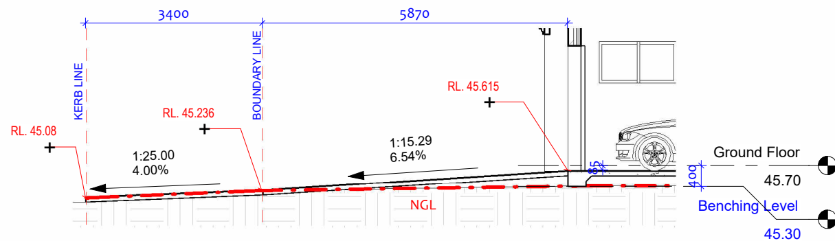
2 DRIVEWAY SECTION 1 : 100
