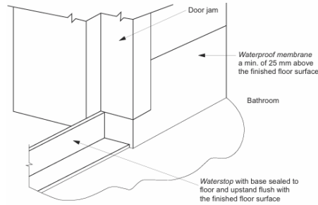
(b) Prior to installation of architrave
