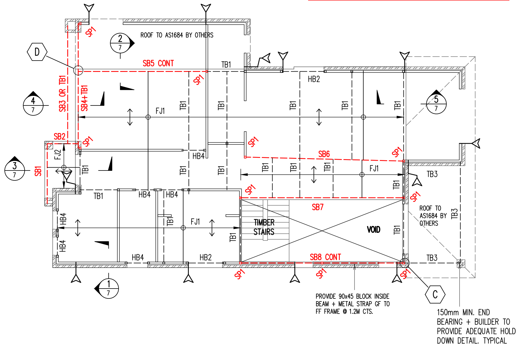
FIRST FLOOR – STEEL BEAM AND FLOOR JOIST LAYOUT PLAN
