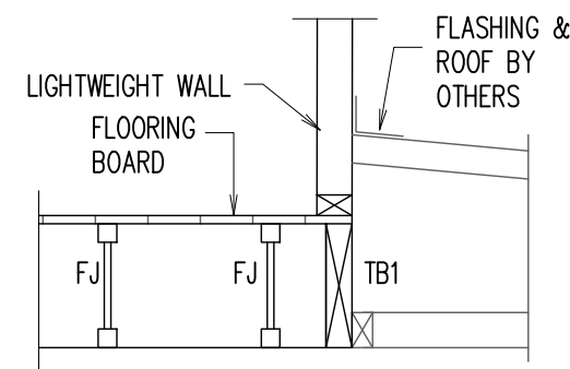
SECTION 5 SCALE 1:20
