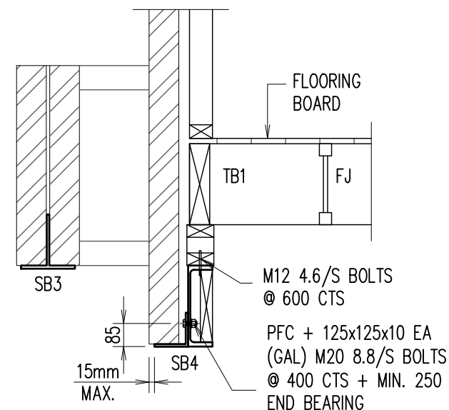
SECTION 4 SCALE 1:20
