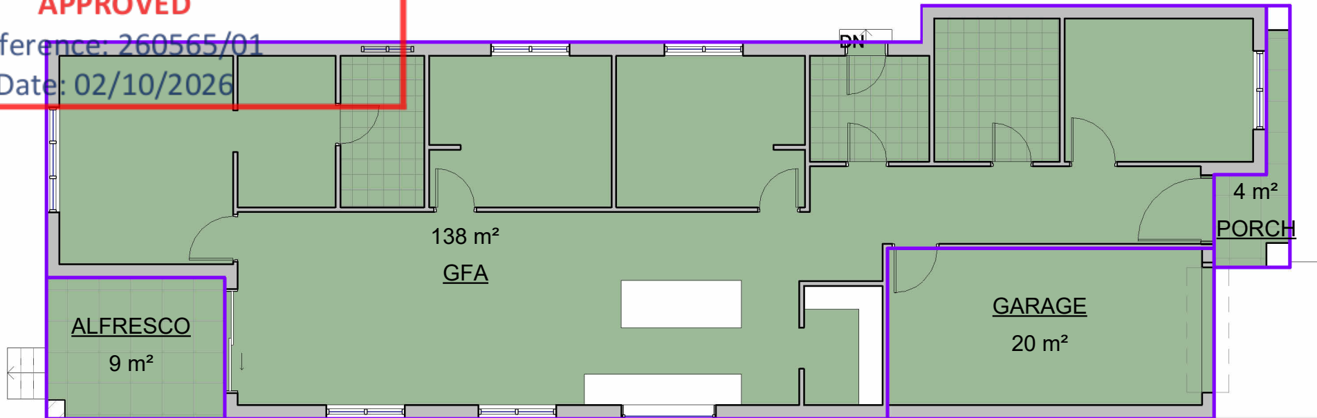
1 Ground Floor 1 : 100
