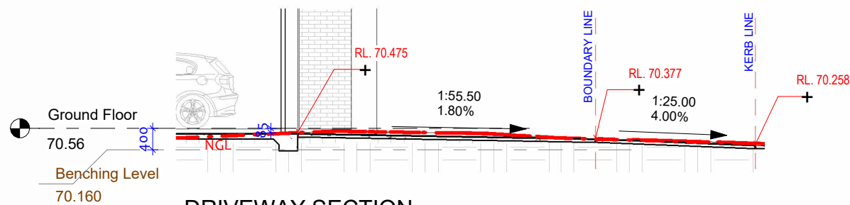
DRIVEWAY SECTION
