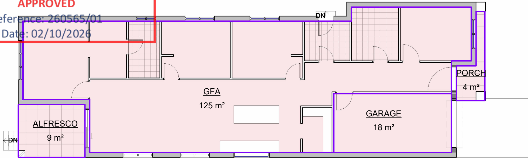
1 Ground Floor 1 : 100
