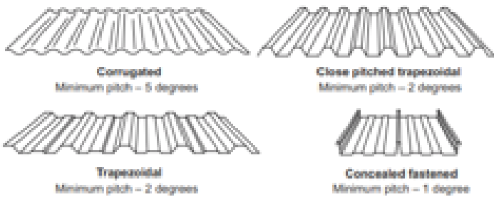
Figure 7.2.3: Minimum pitch requirements for metal roofing profiles
