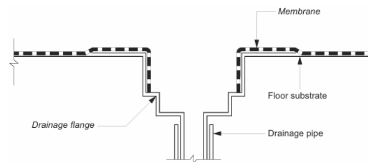
Figure 10.2.29: Typical membrane termination at drainage outlet
