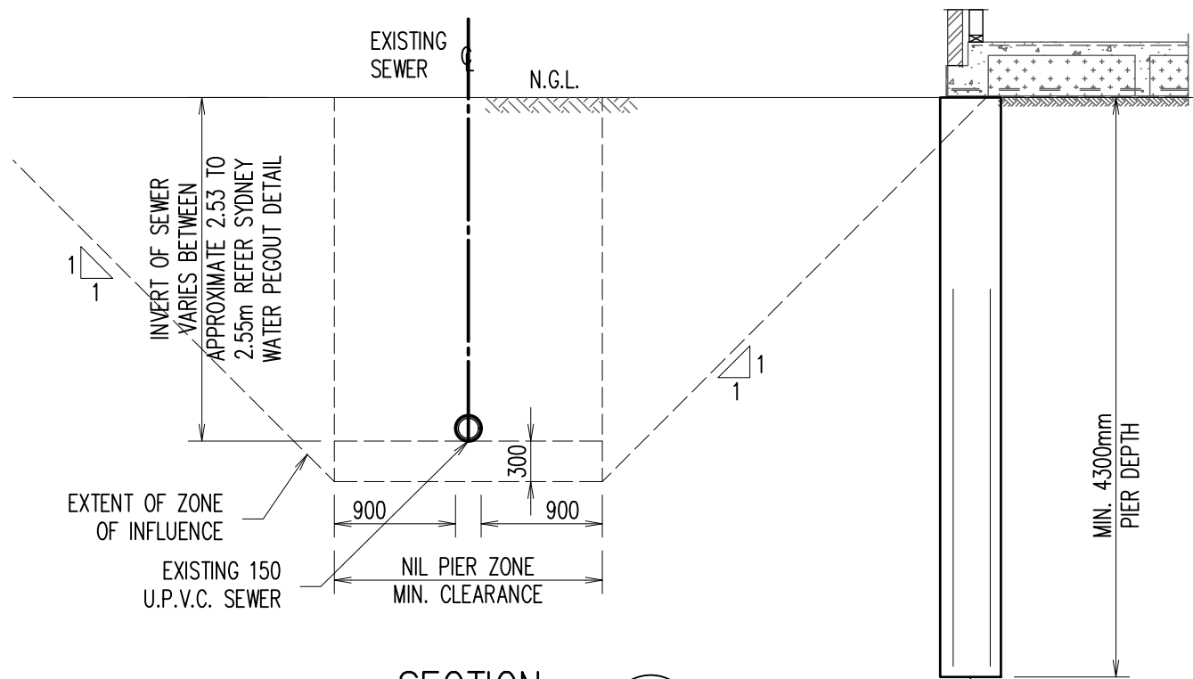
SECTION S1 SCALE 1:50
