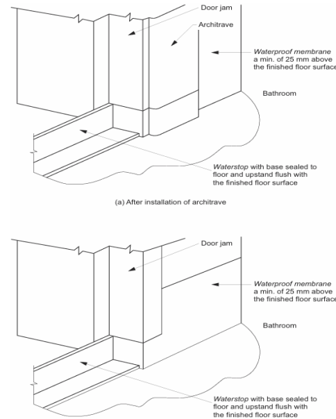
Figure 10.2.24: Typical bathroom door details for whole bathroom waterproofing
