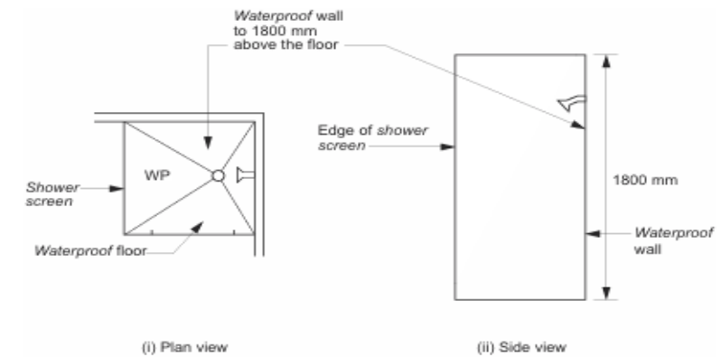
(a) Enclosed shower
