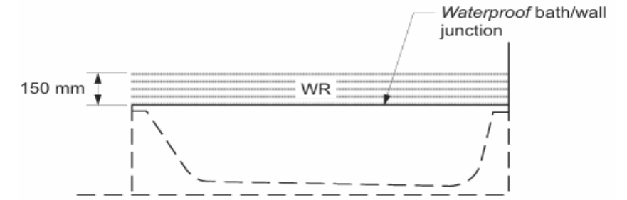
(b) Wall/bath junction
