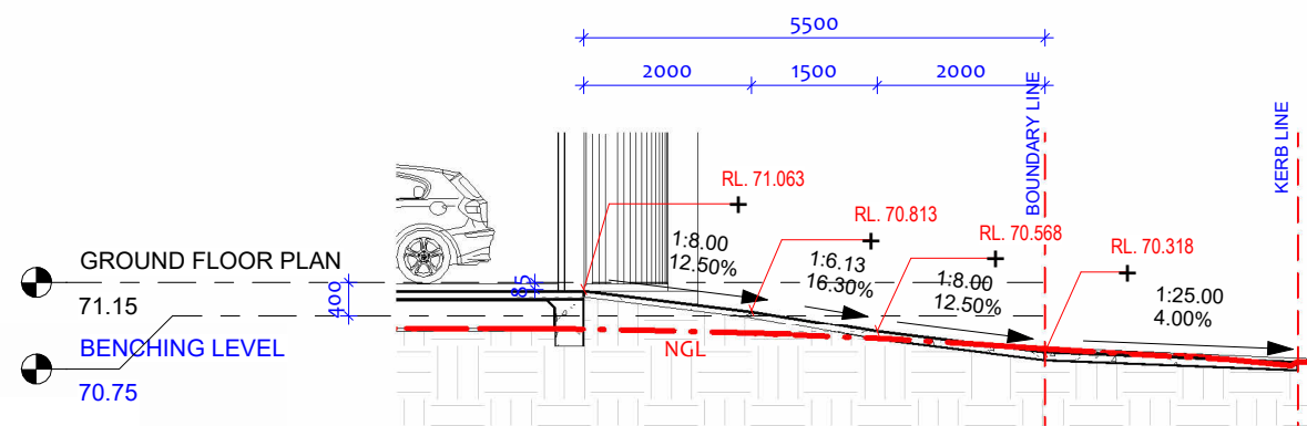
DRIVEWAY SECTION
