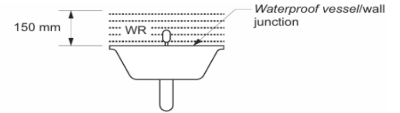
(a) Vessel abutting wall
