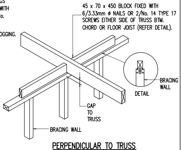
TIMBER BRACING WALL TOP CONNECTION DETAIL
