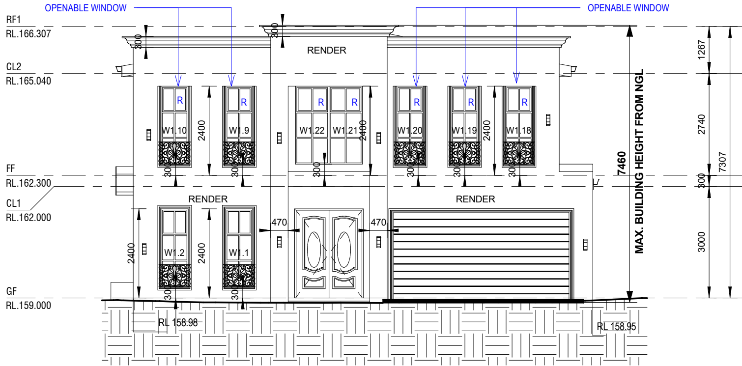
1 NORTH WEST ELEVATION A03 1 : 100
