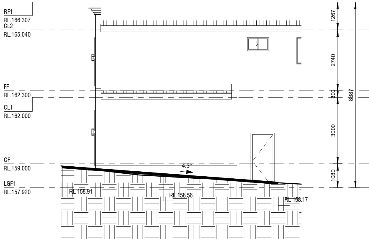
1 A05 SECTION - DW1 ENTRY TO LAUNDRY RAMP 1 : 100
