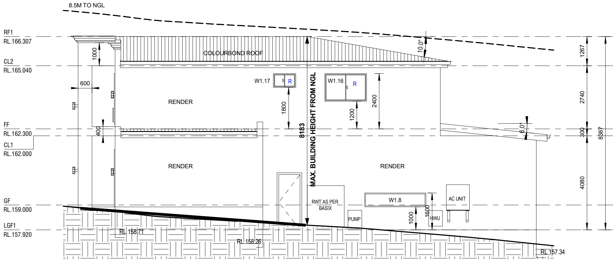
1 SOUTH WEST ELEVATION A04 1 : 100
