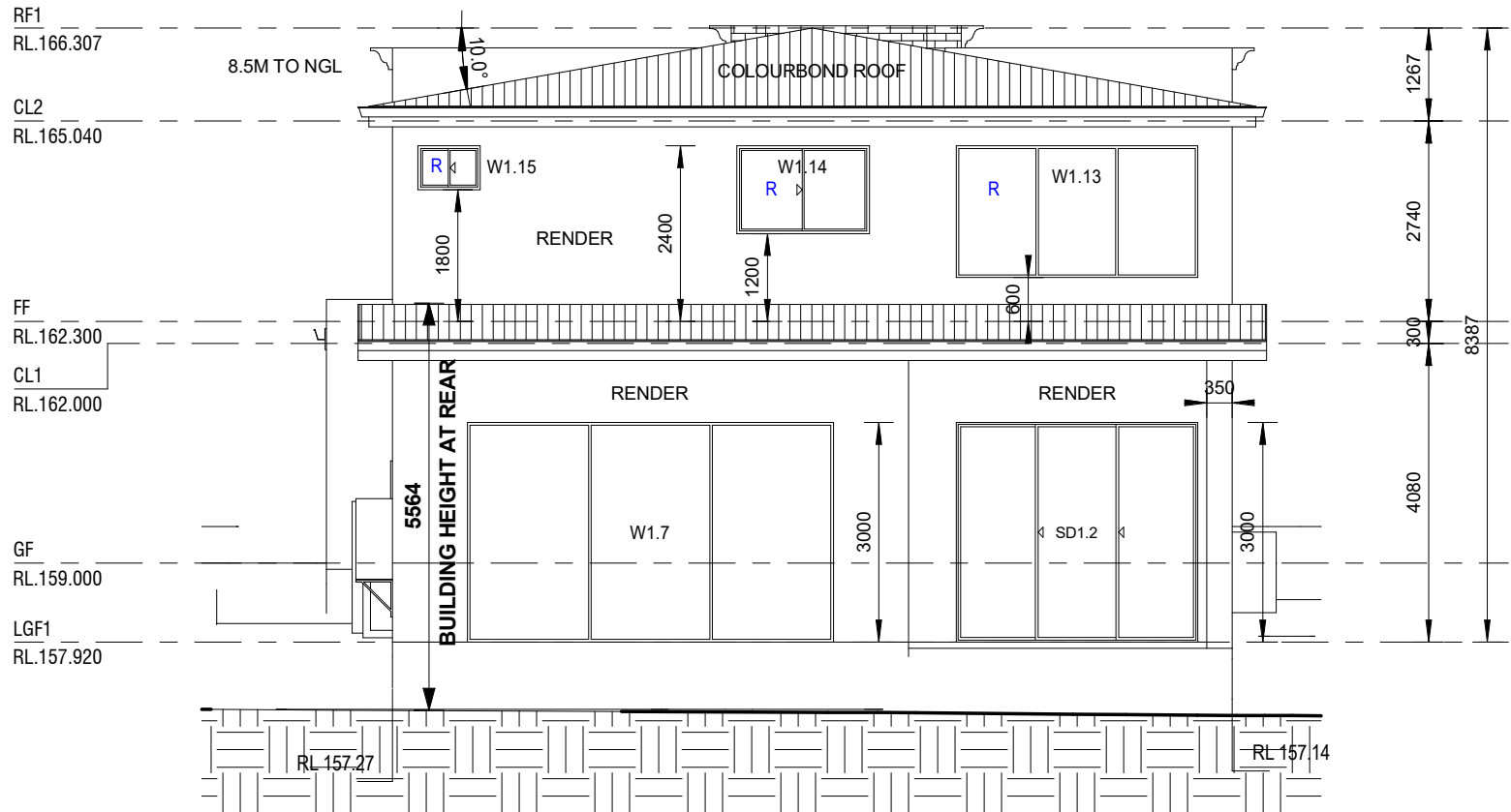
2 SOUTH EAST ELEVATION A04 1 : 100
