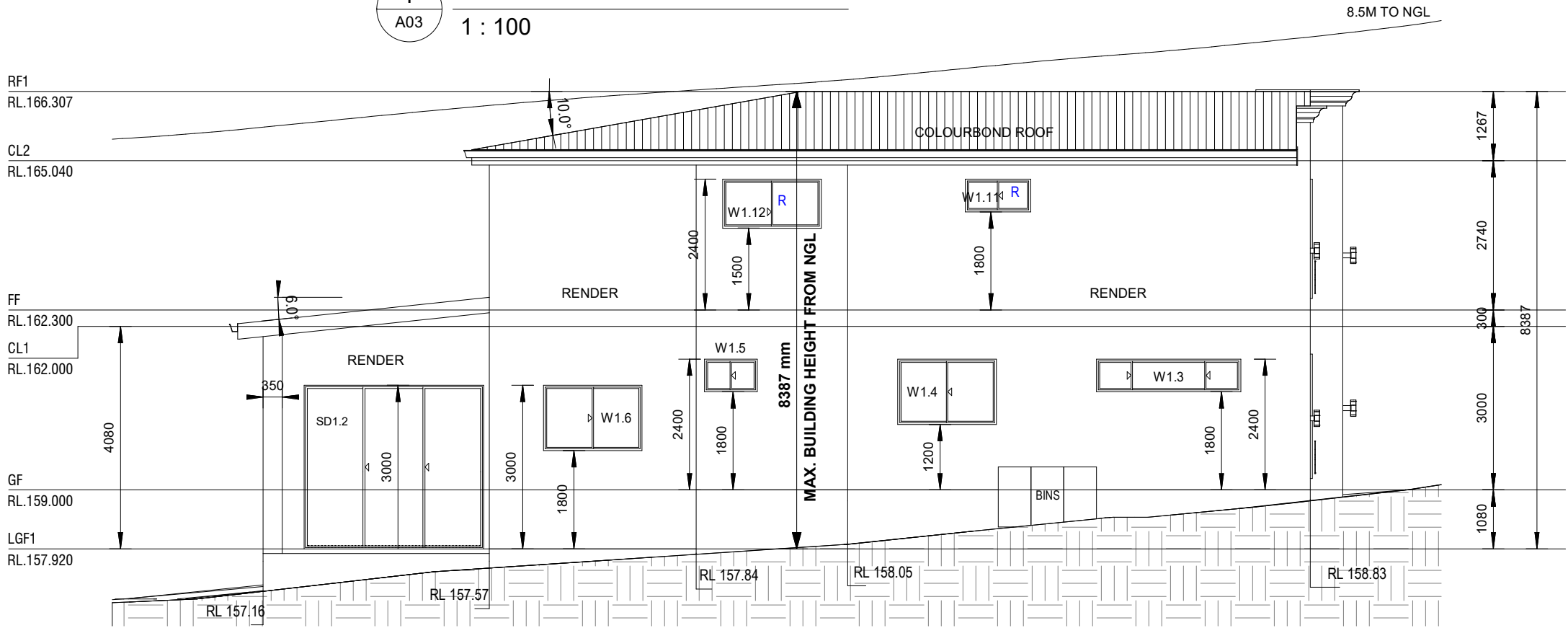
2 NORTH EAST ELEVATION A03 1 : 100
