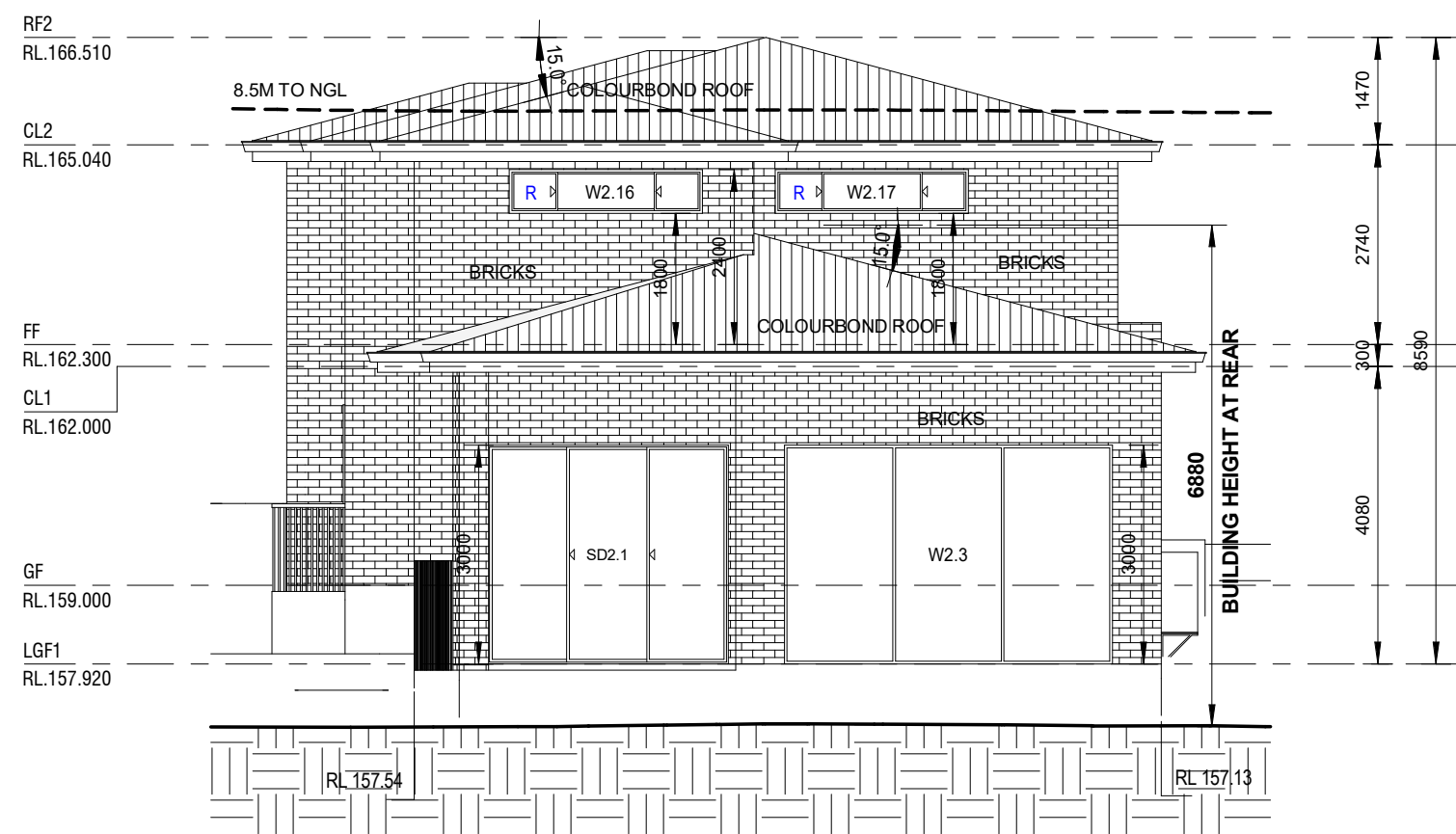
1 SOUTH EAST ELEVATION A04 1 : 100
