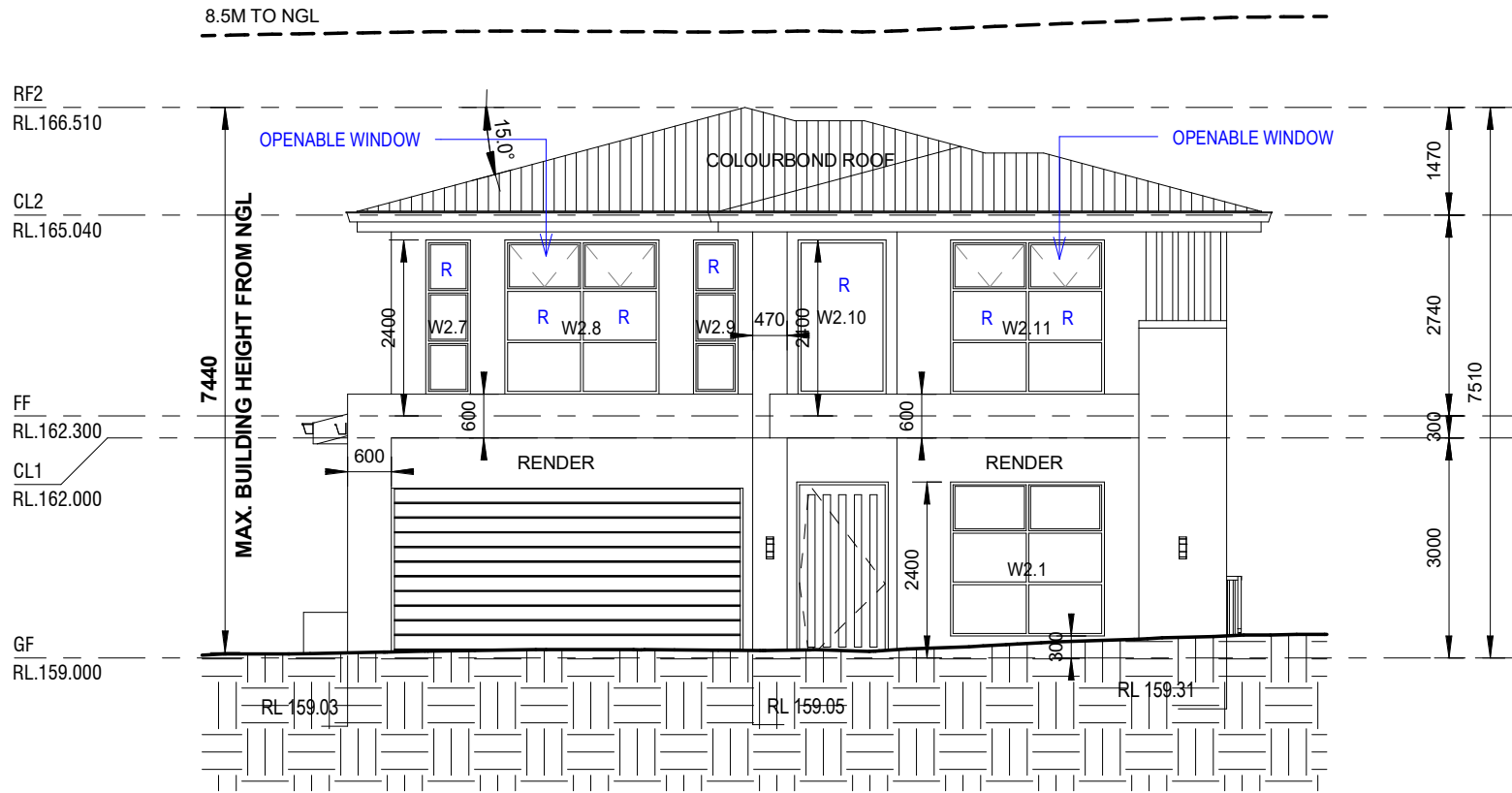
1 NORTH WEST ELEVATION A03 1 : 100
