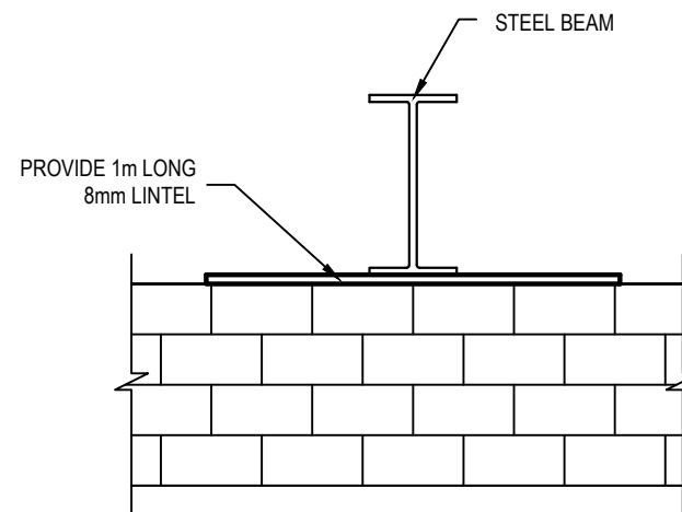
TYPICAL BEAM BEARING DETAIL
