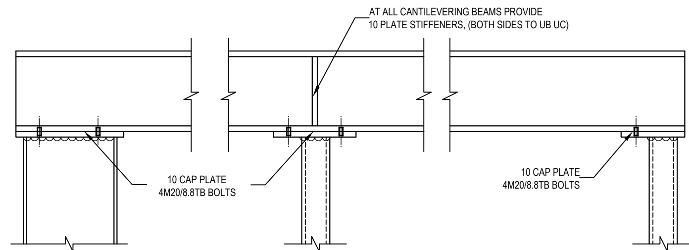
TYPICAL BEAM TO COLUMN CONNECTIONS
