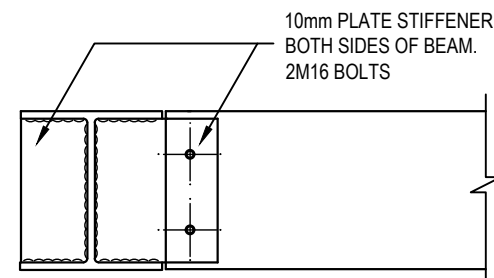
BEAM TO BEAM CONNECTION
