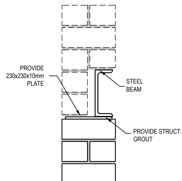
TYPICAL BEAM BEARING DETAIL
