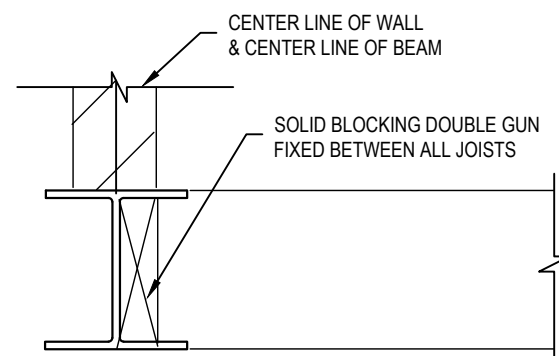
RAFTERS & JOISTS AT BEAMS
