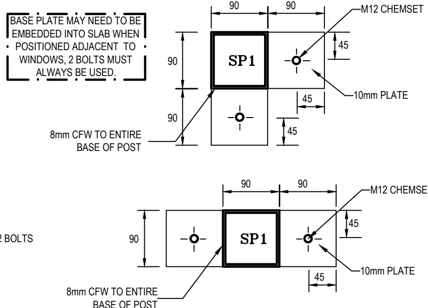
BASE PLATE DETAIL OPTIONS
