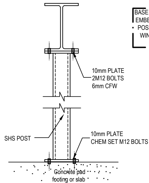
SHS POST WITH BEAM DETAIL
