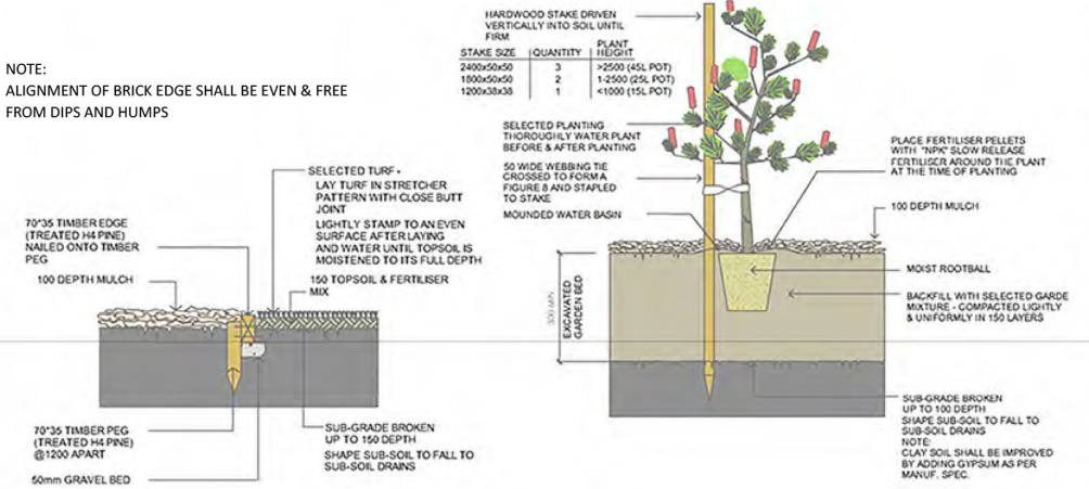
TURF & GARDEN EDGE DETAIL
