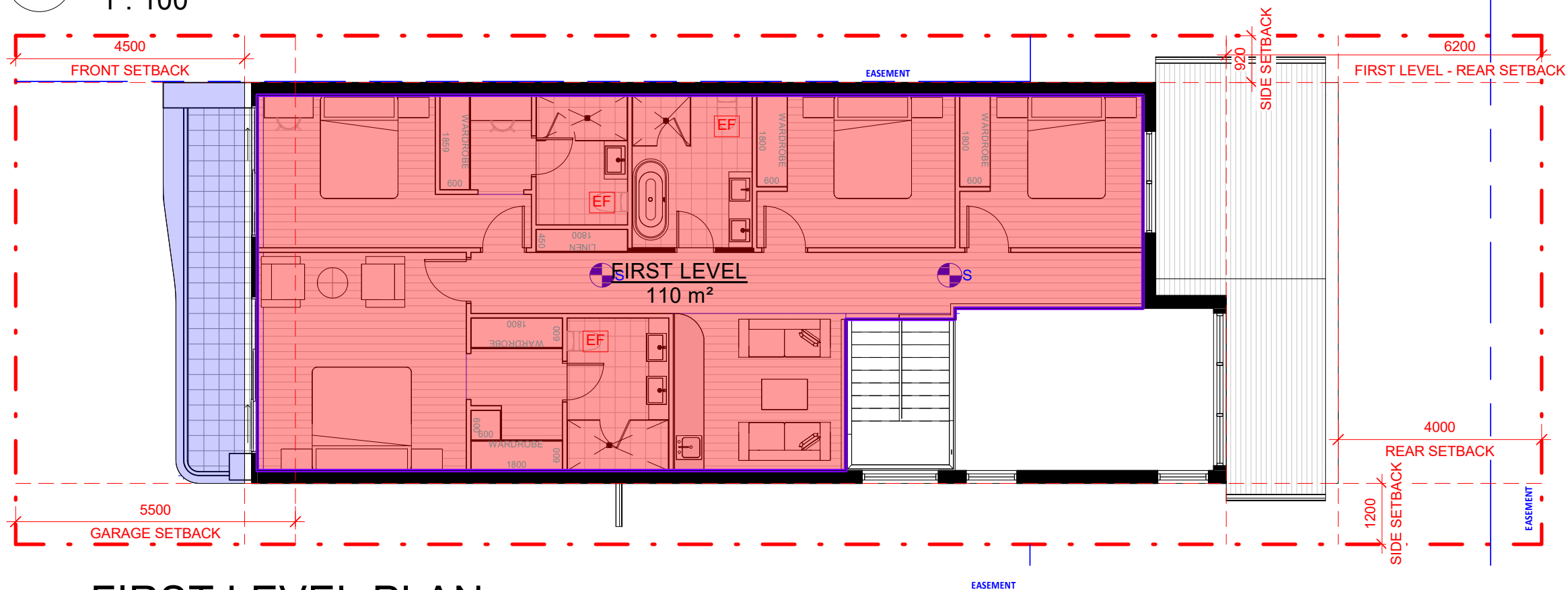
2 FIRST LEVEL PLAN 1 : 100
