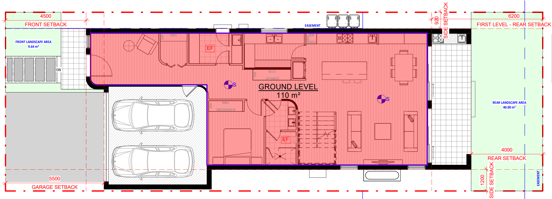
1 GROUND LEVEL PLAN 1 : 100
