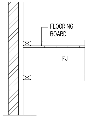
SECTION 1 SCALE 1:20
