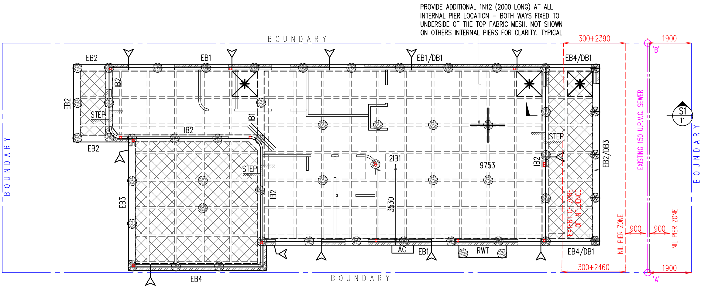
GROUND FLOOR WAFFLE SLAB LAYOUT PLAN SCALE 1:100
