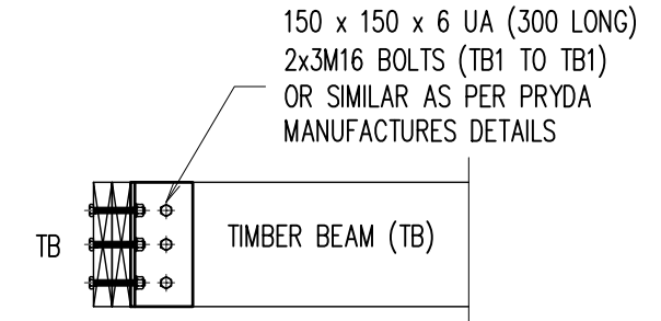
TYPICAL TIMBER BEAM (TB) TO TB DETAIL
