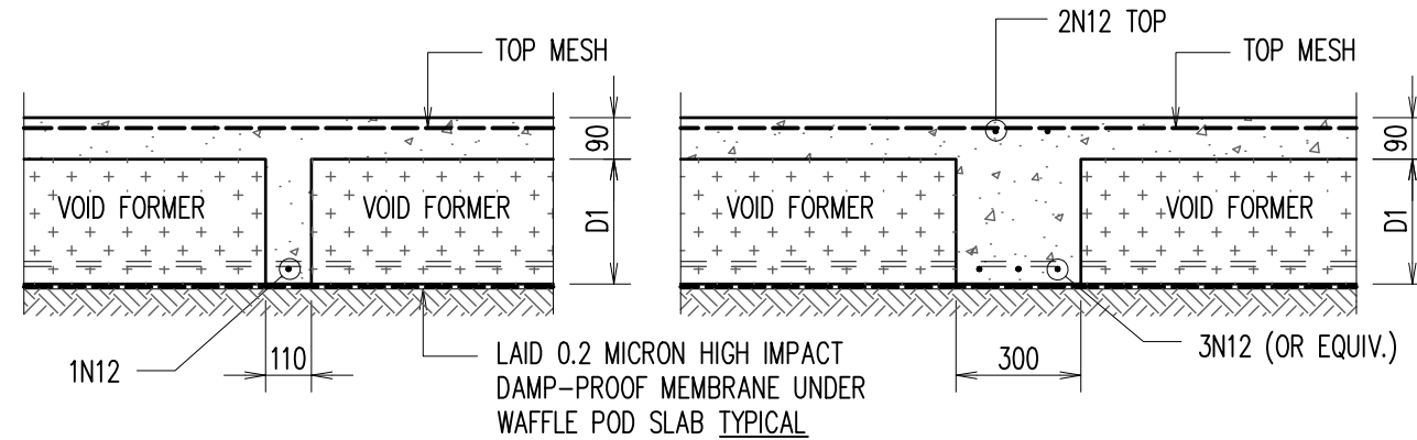
INTERNAL RIB
