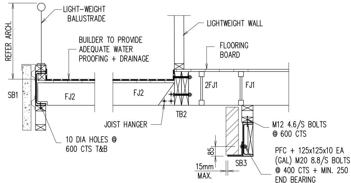
SECTION 5 SCALE 1:20
