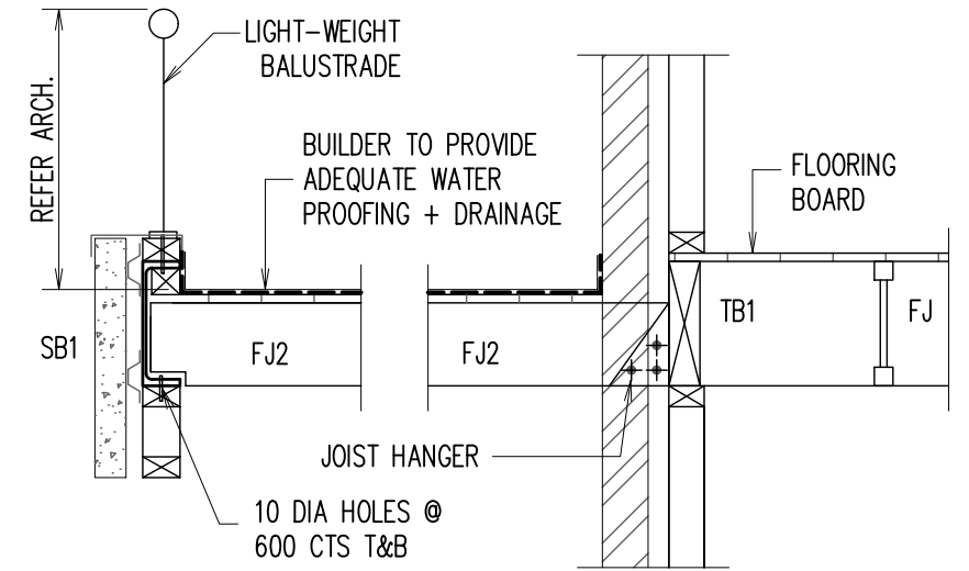
SECTION 4 SCALE 1:20
