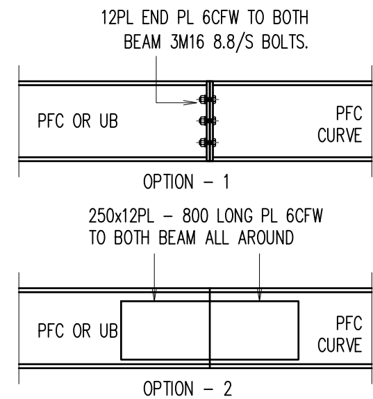
TYPICAL CURVE STEEL BEAM DETAIL
