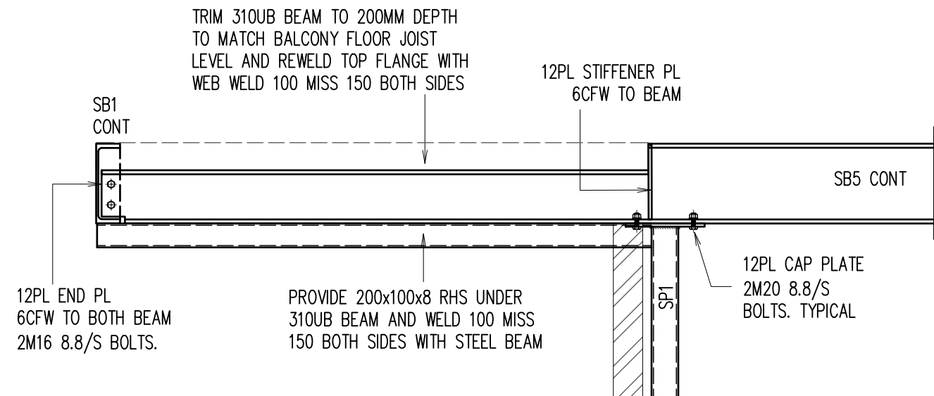
DETAIL - F SCALE 1:20
