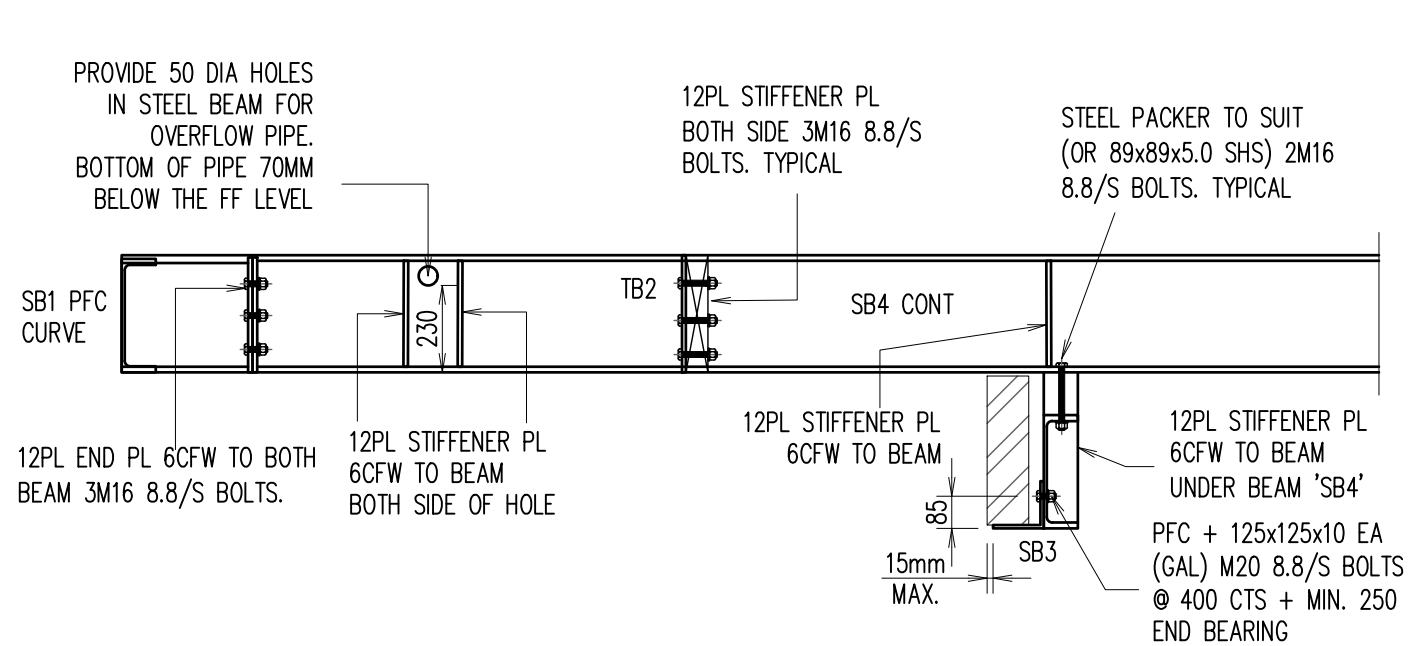
DETAIL - G SCALE 1:20
