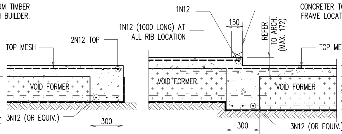
EDGE BEAM – 'EB2' ALTERNATIVELY REFER TO 'DB3' FOR DETAILS
