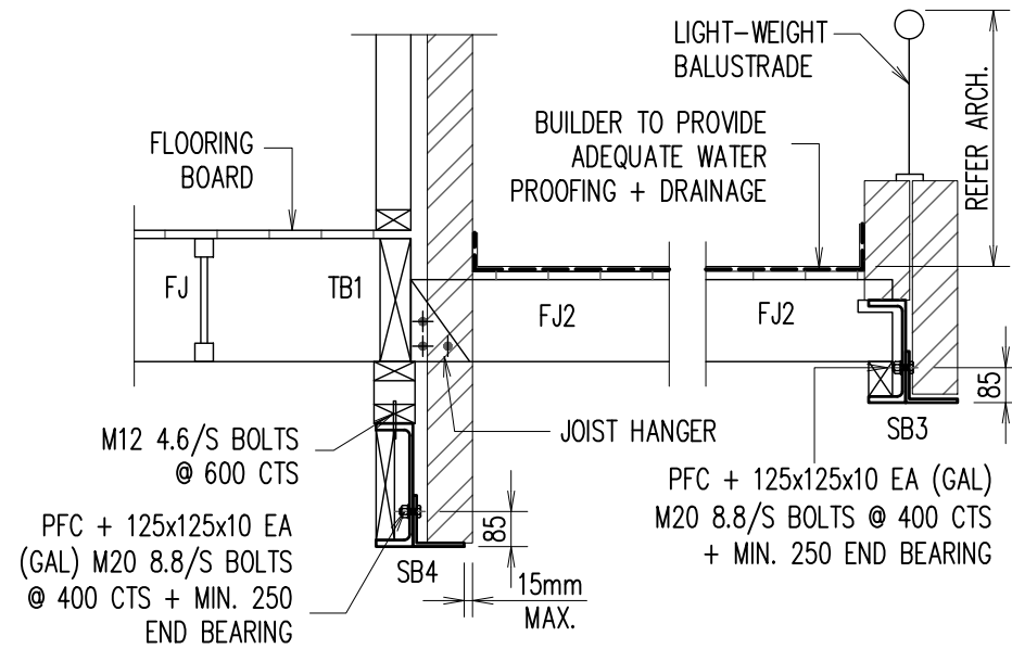
SECTION 3 SCALE 1:20
