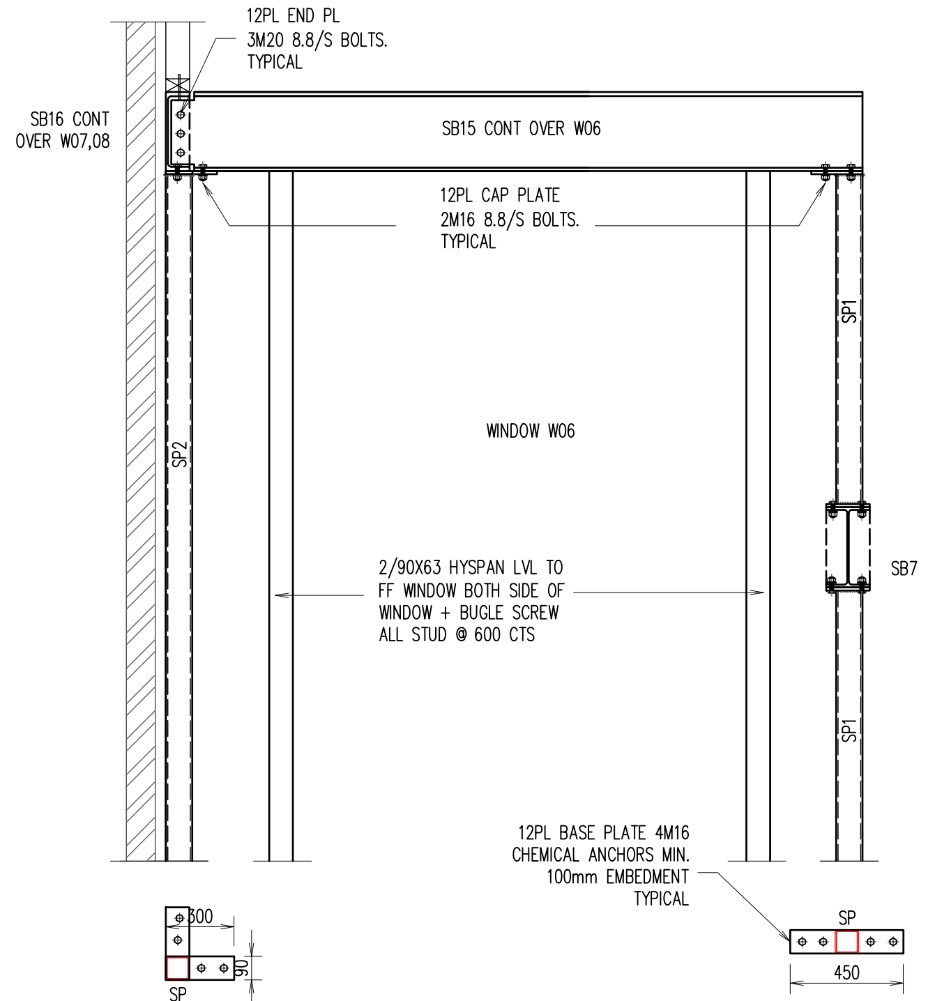
BASE PLATE DETAILS
