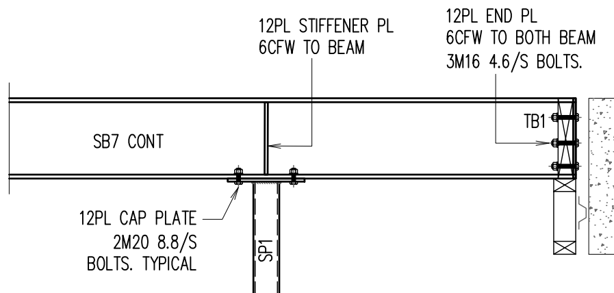
DETAIL - F SCALE 1:20
