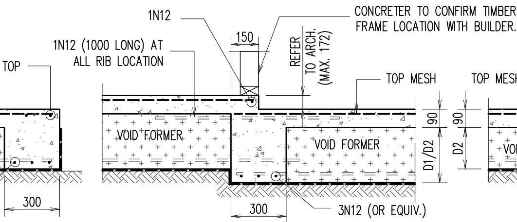
INTERNAL STEPDOWN BEAM – 'IB3'
