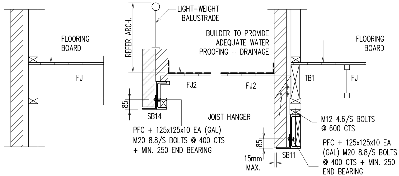
SECTION 1 SCALE 1:20
