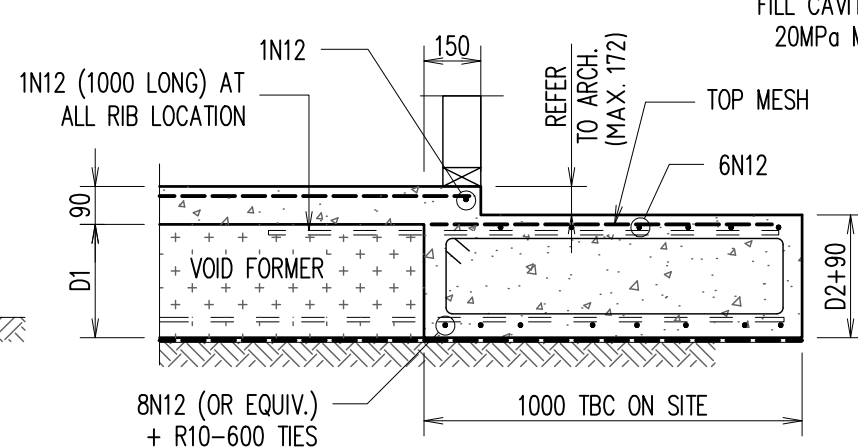
INTERNAL STEPDOWN BEAM – 'IB3'
