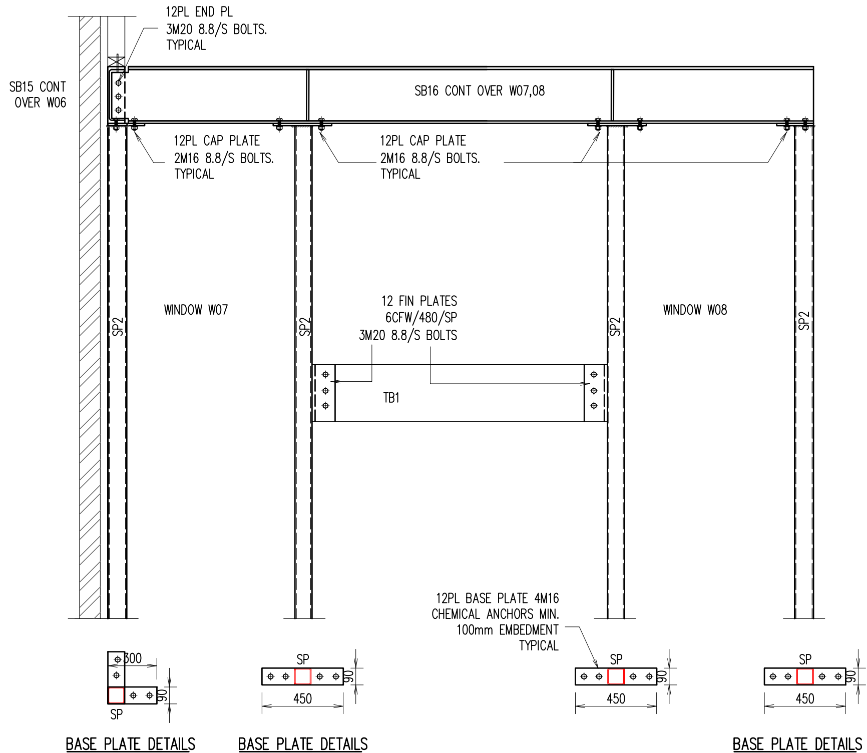
DETAIL – H SCALE 1: 20
