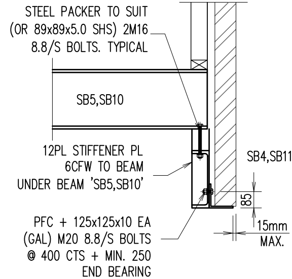
DETAIL - E SCALE 1:20
