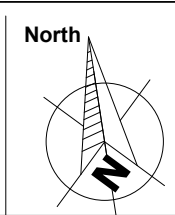
Shadow @ 10AM
