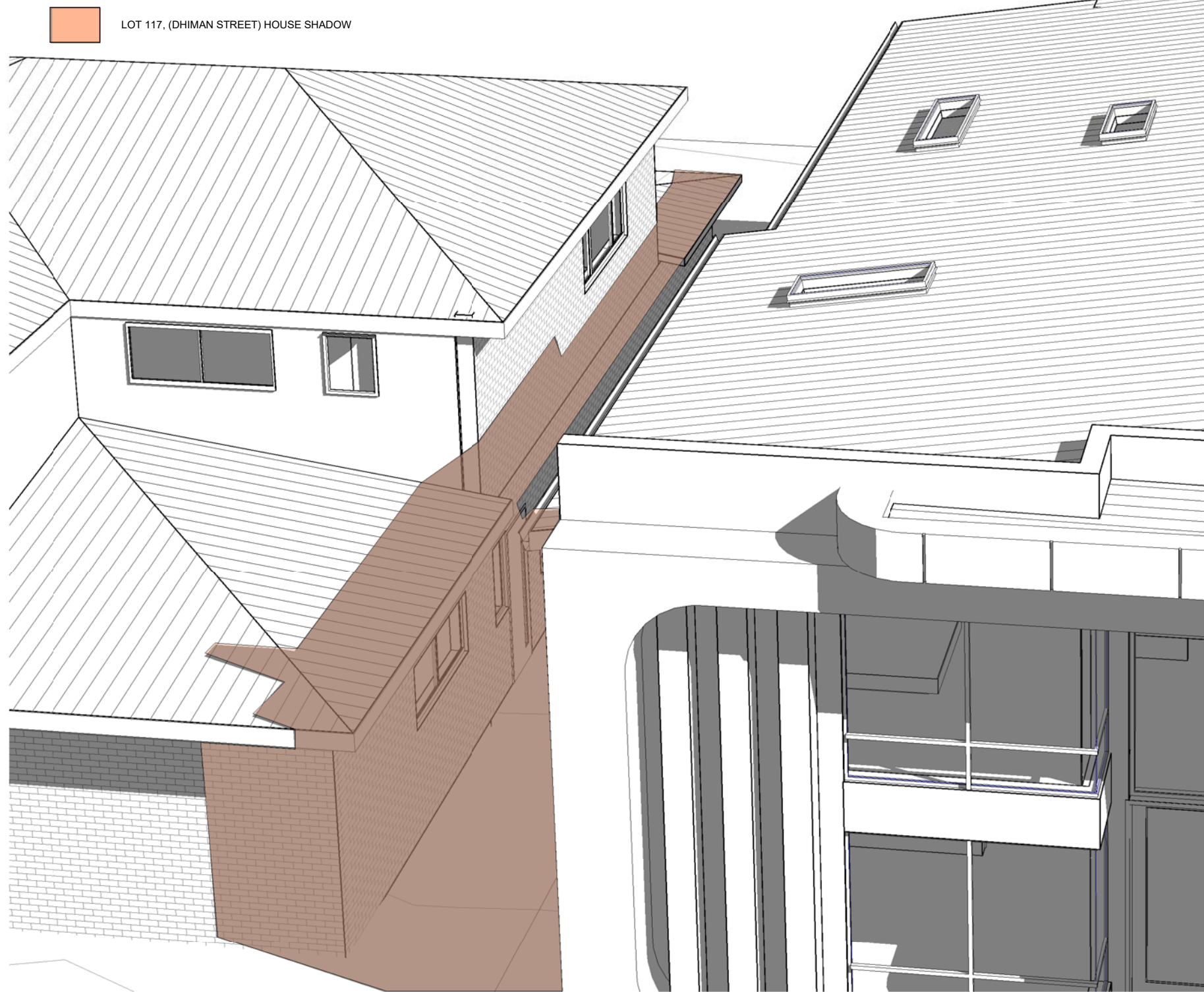
Shadow @ 11AM
