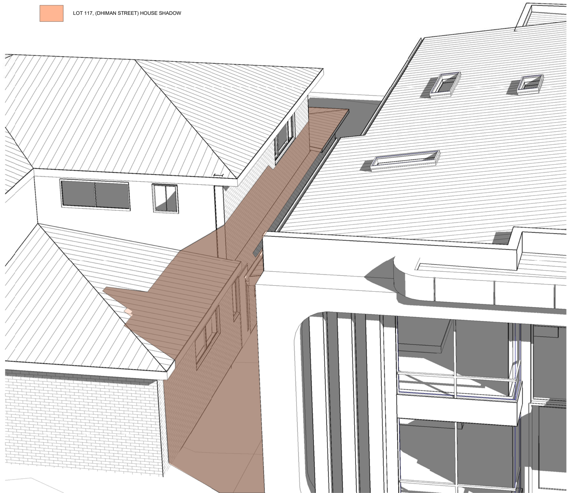
Shadow @ 10AM
