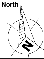
Shadow @ 2PM
