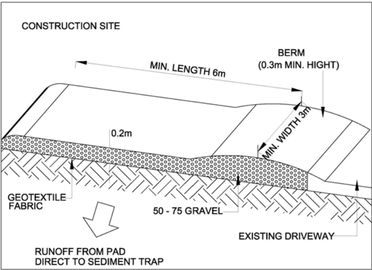
Temporary Construction Driveway (Not to scale)
