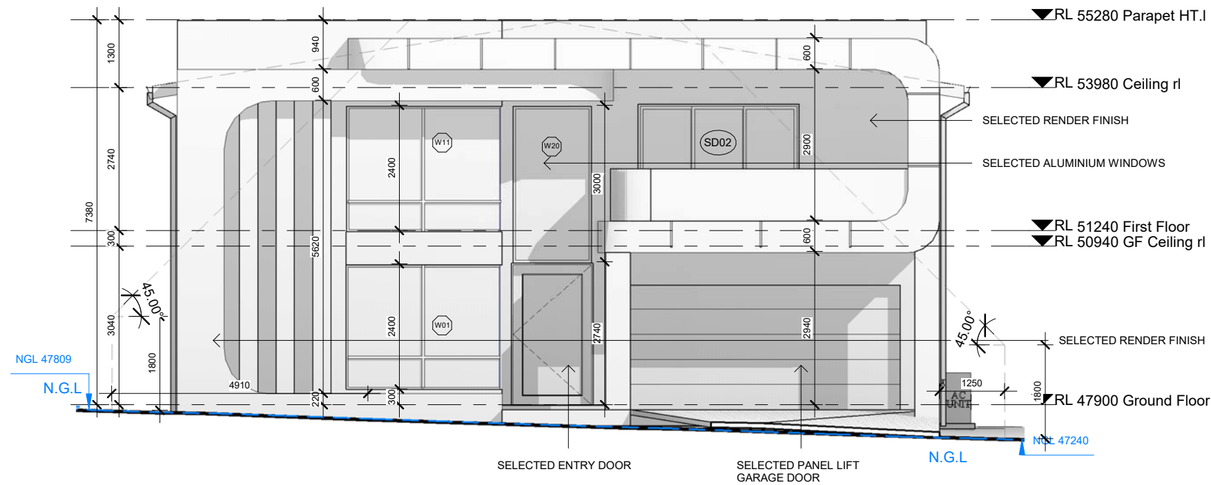
EAST ELEVATION 1 : 100
