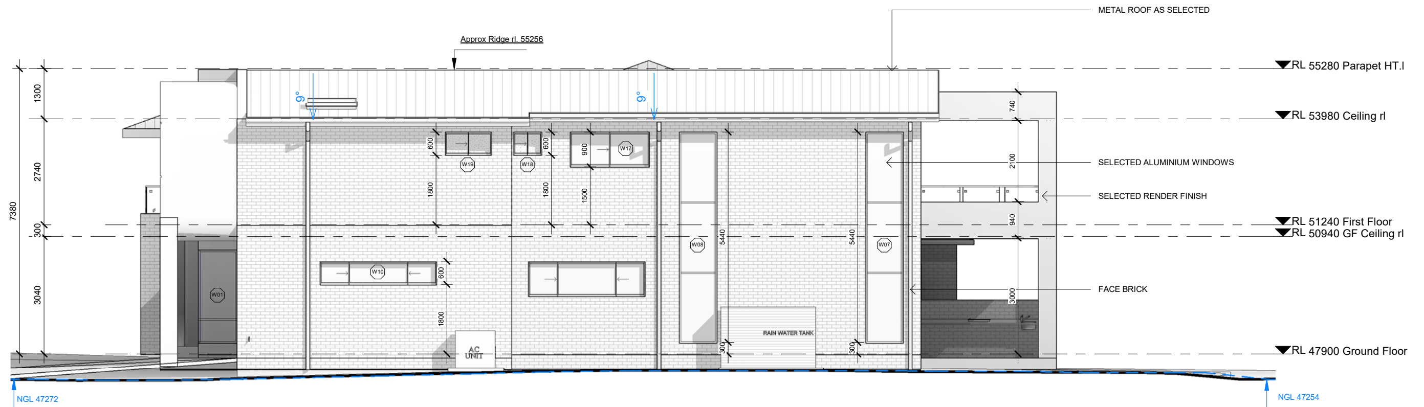
EAST ELEVATION 1 : 100
