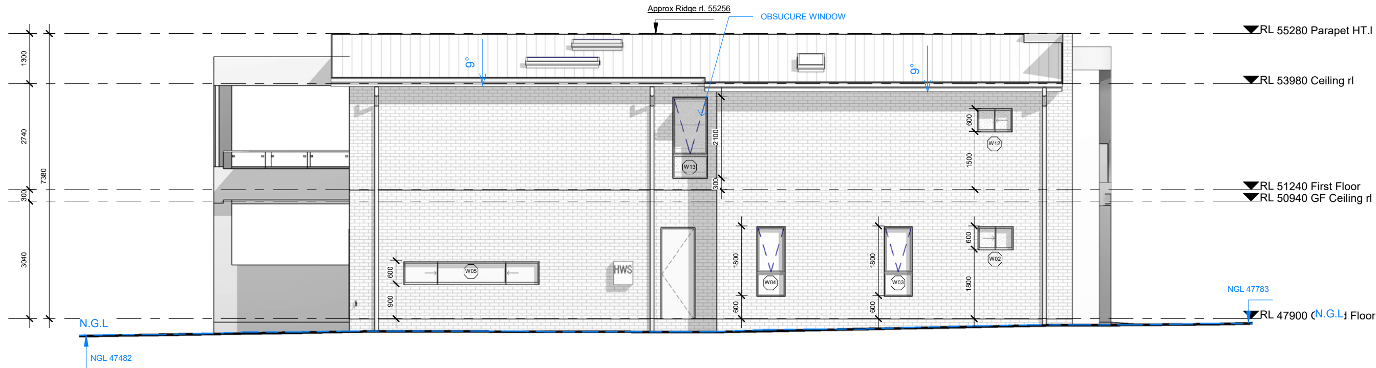
SOUTH ELEVATION 1 : 100
