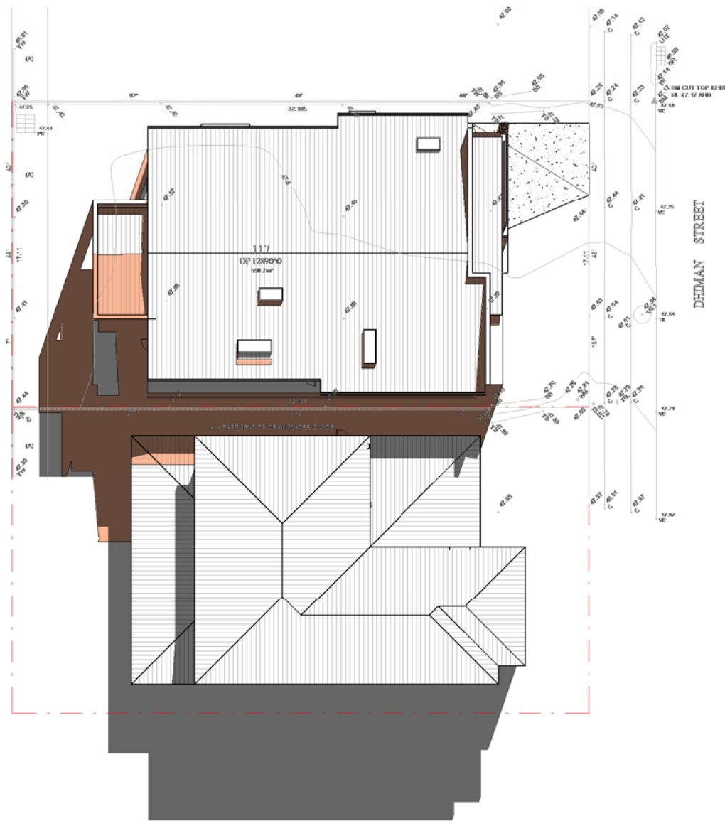
SHADOW AT 11AM 1 : 300
