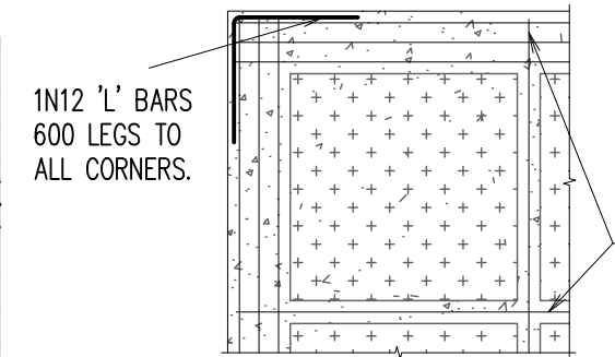
TYPICAL CORNER DETAILS
