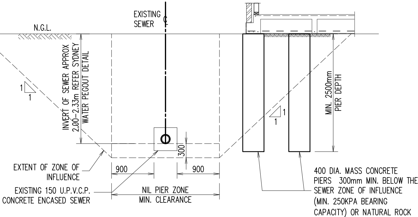
SECTION SCALE 1:50 S1 3
