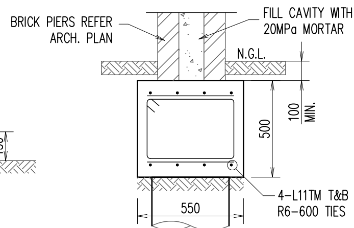
STRIP FOOTING (SF1) DETAILS
