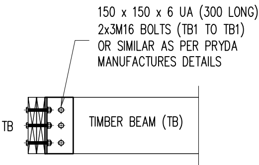
TYPICAL TIMBER BEAM (TB) TO TB DETAIL
