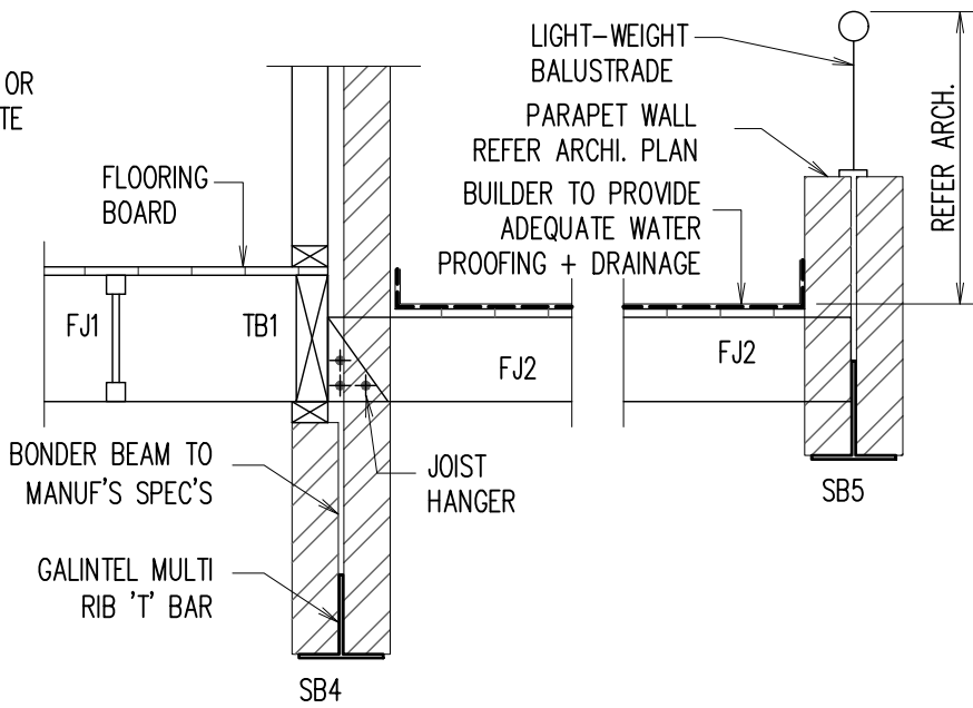
SECTION 4 SCALE 1:20
