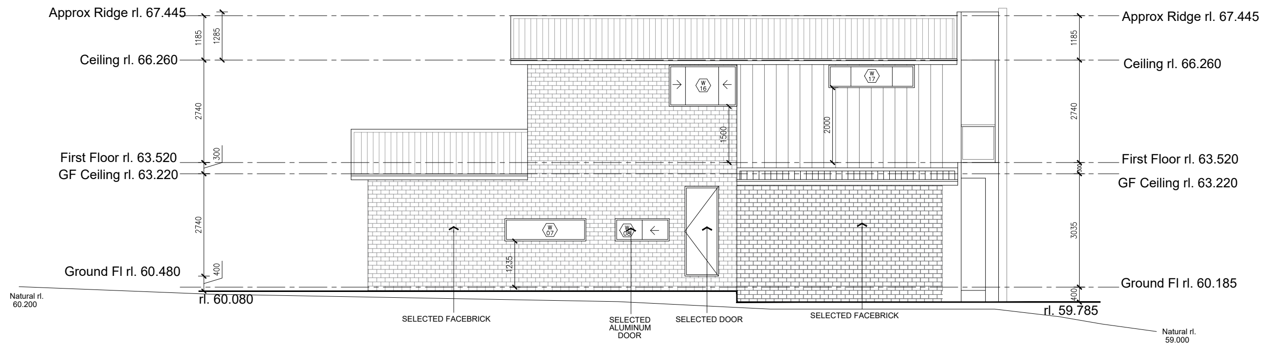
North-West Elevation
