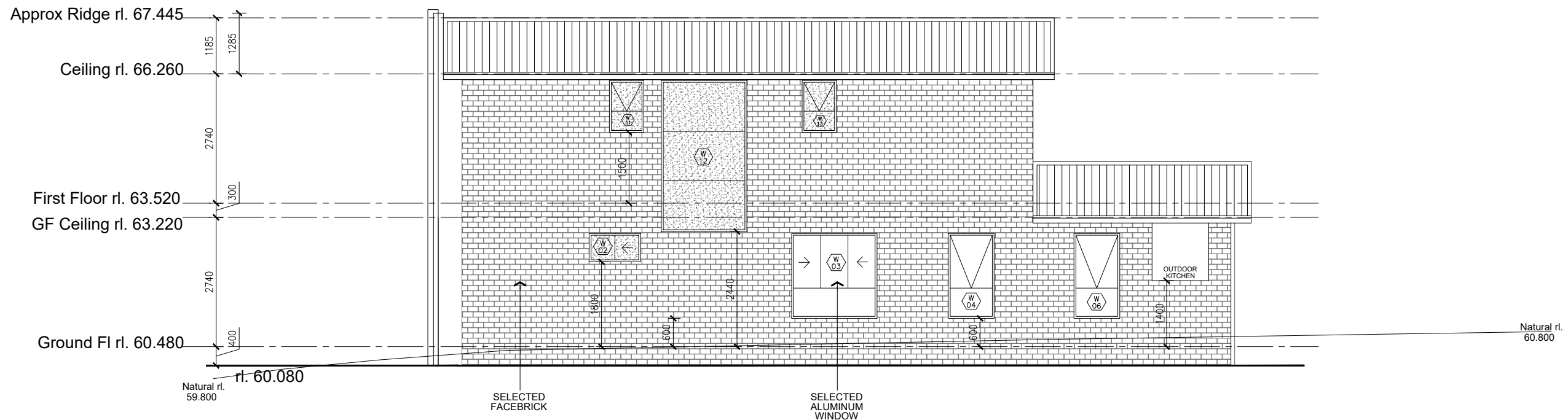
South-East Elevation
