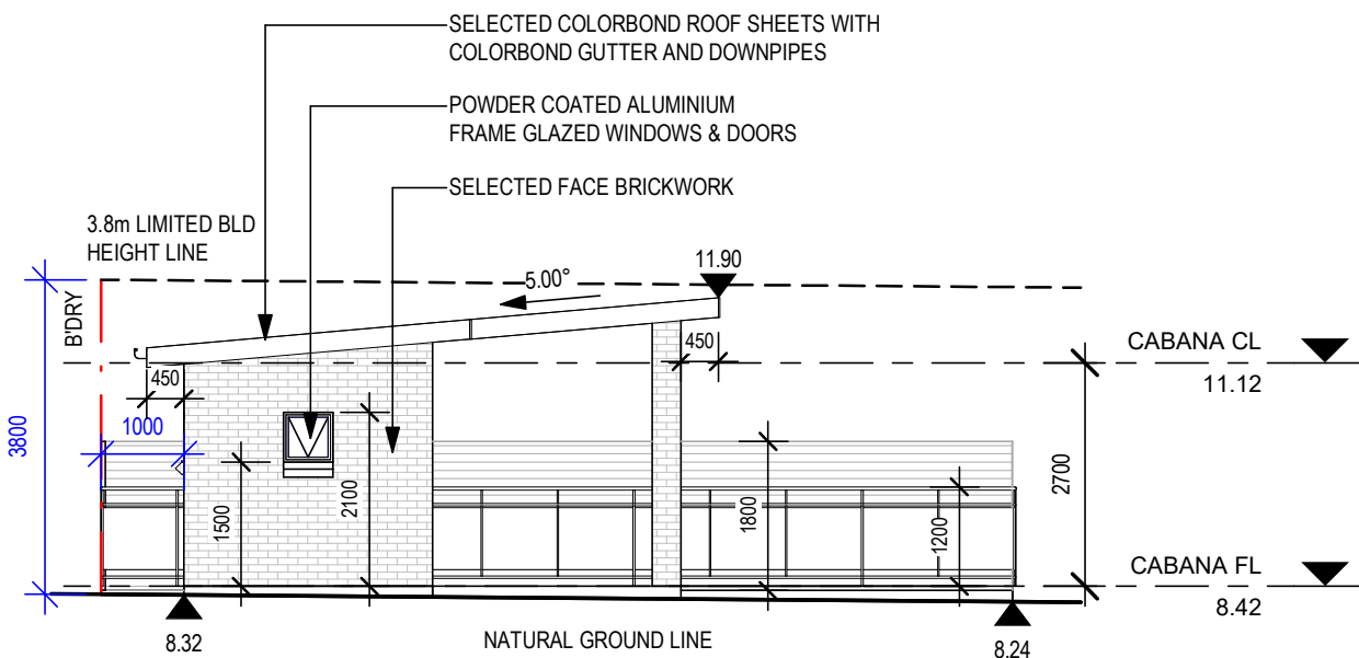
4 CABANA SOUTH ELEVATION 1 : 100
