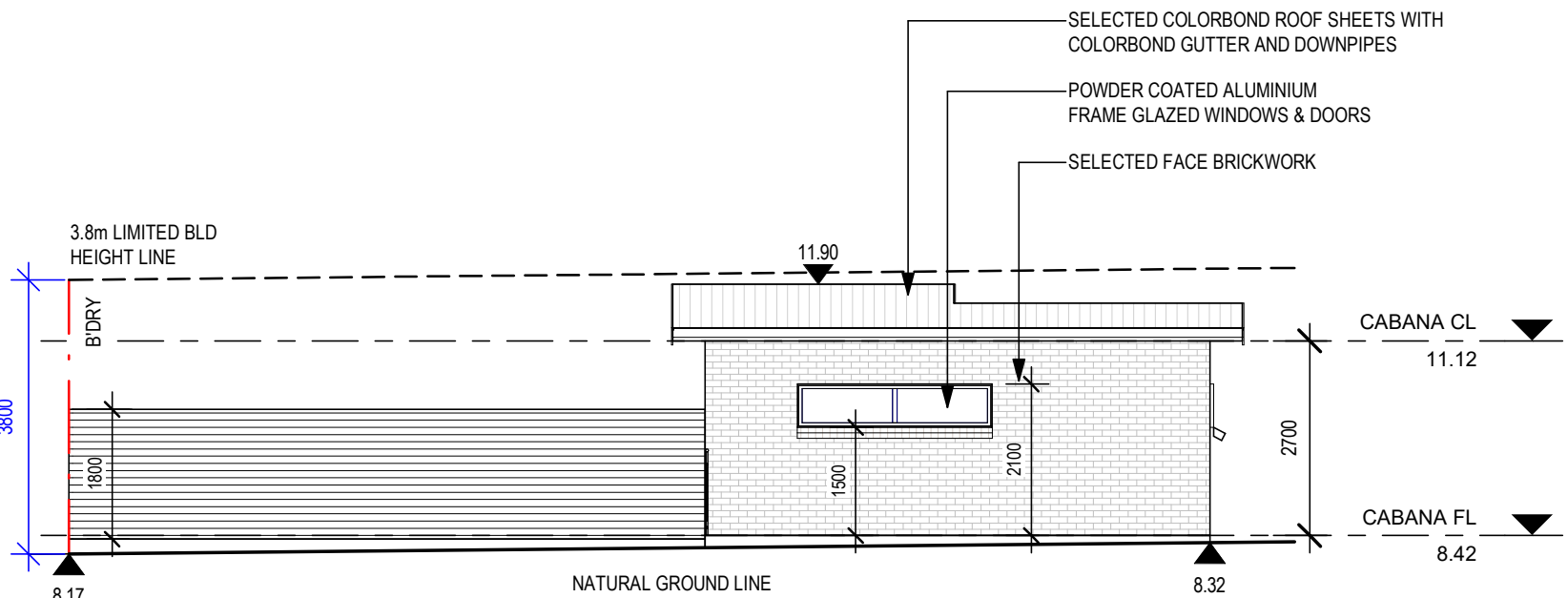
5 CABANA WEST ELEVATION 1 : 100
