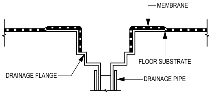
C02 TYPICAL MEMBRANE TERMINATION AT DRAINAGE OUTLET NOT TO SCALE
