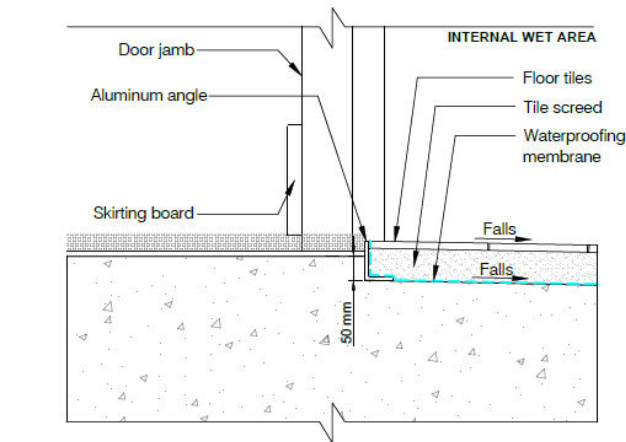
INTERNAL WET AREA DOOR THRESHOLD
