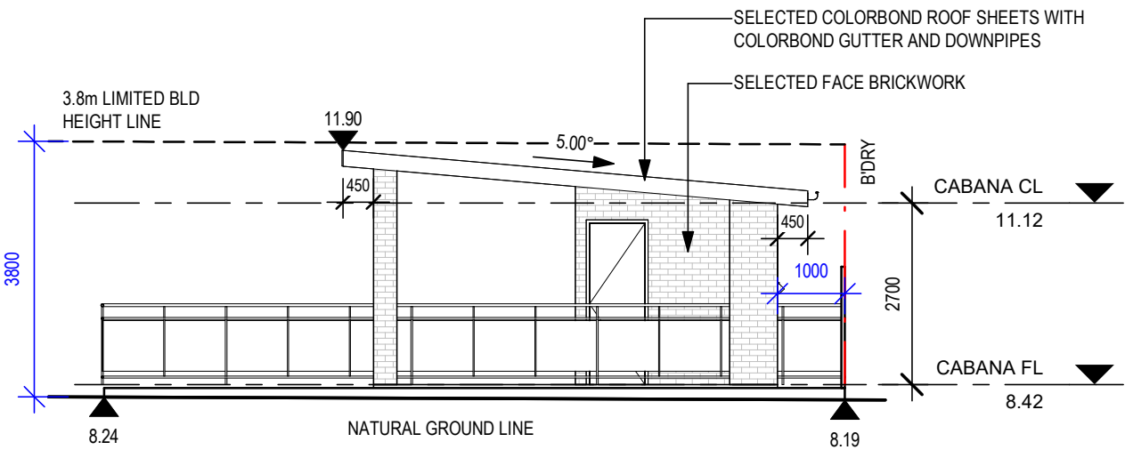
2 CABANA NORTH ELEVATION 1 : 100
