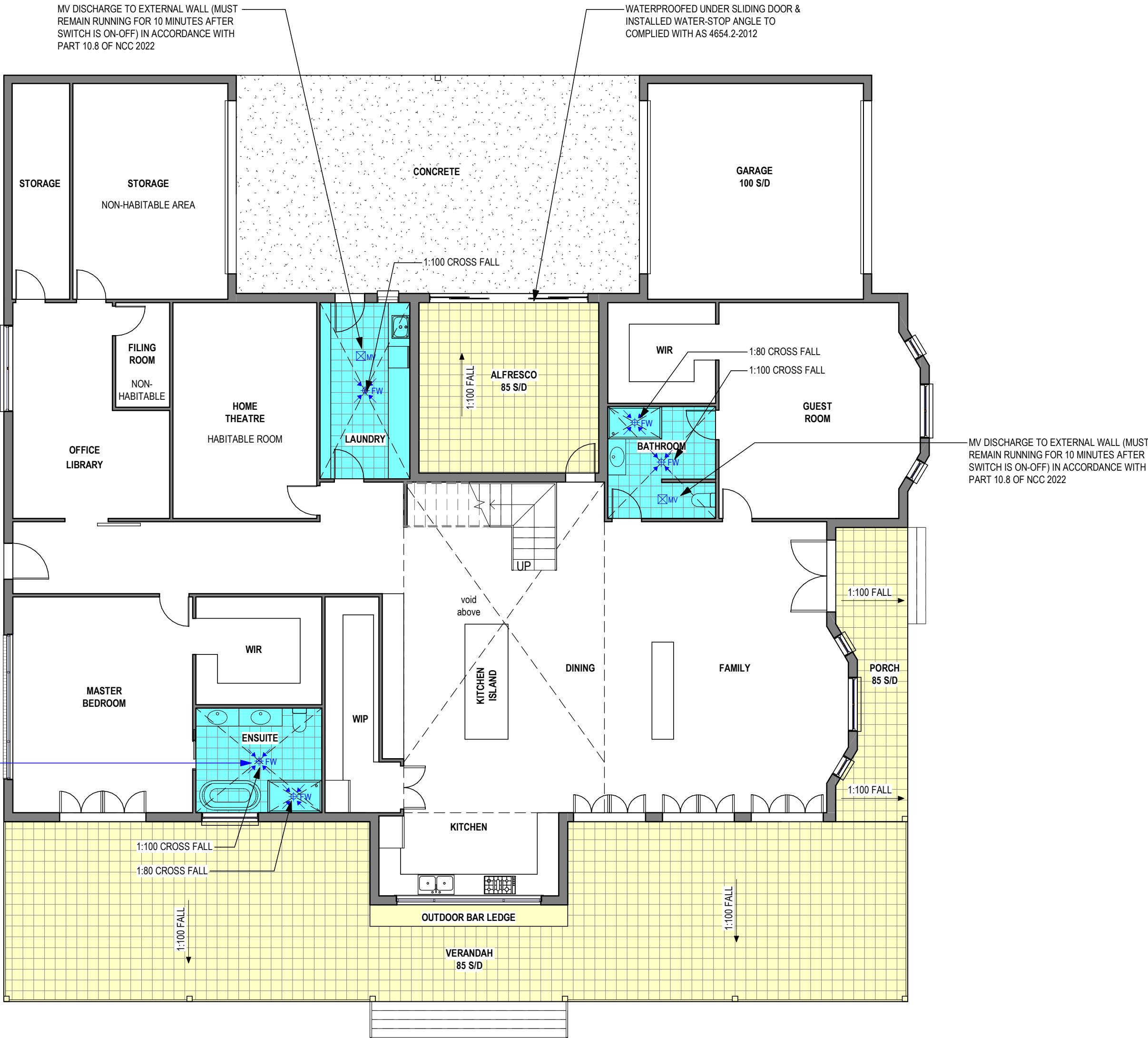
1 WET AREAS PLAN - GROUND FLOOR 1 : 100
