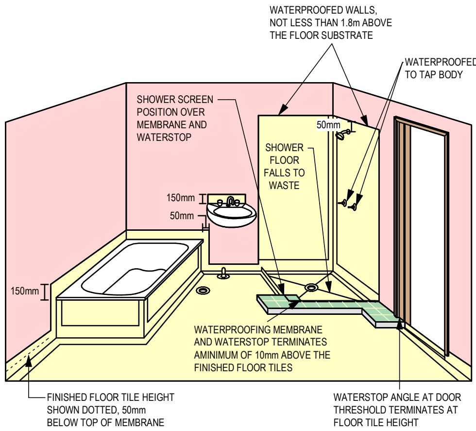
C03 WATERPROOFING DETAILS AROUND BATHROOM
