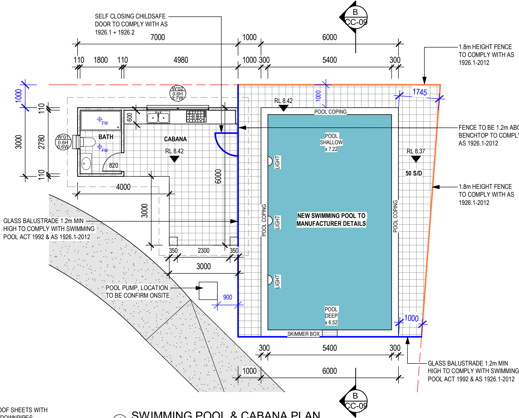
1 SWIMMING POOL & CABANA PLAN 1 : 100
