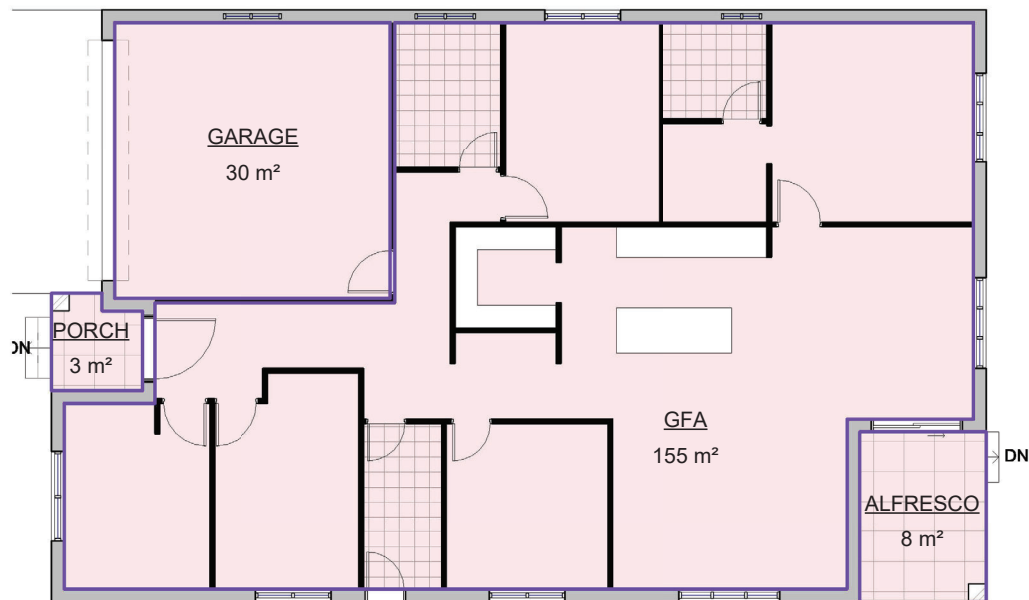
1 Ground Floor 1 : 100
