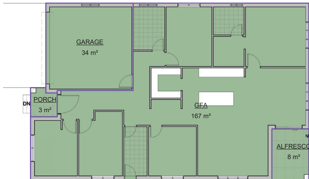
1 Ground Floor 1 : 100
