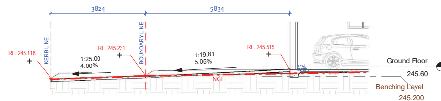
2 DRIVEWAY SECTION
