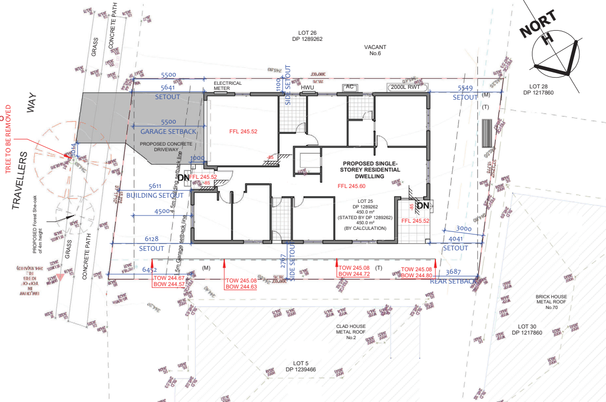
CC - SITE PLAN
