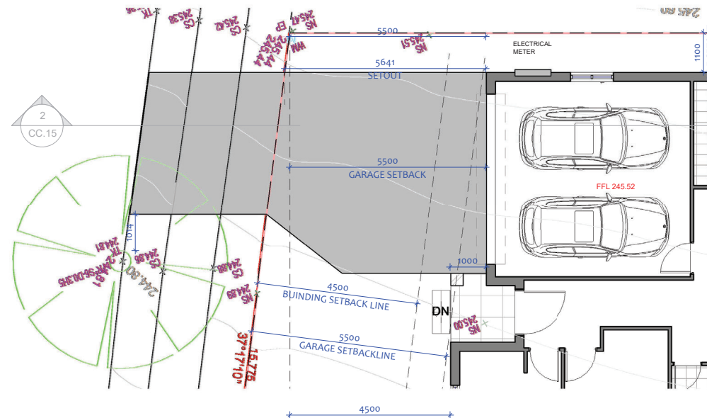
1 CC - DRIVEWAY PLAN 1 : 100
