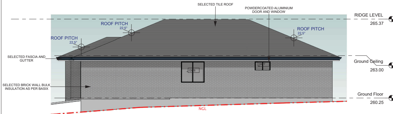
1 South-East Elevation 1 : 100
