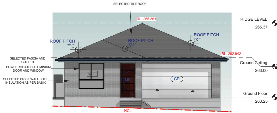
1 South-West Elevation 1 : 100
