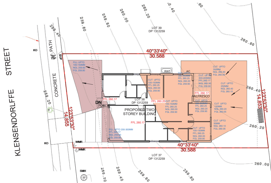
DA - CUT AND FILL PLAN 1 : 200
