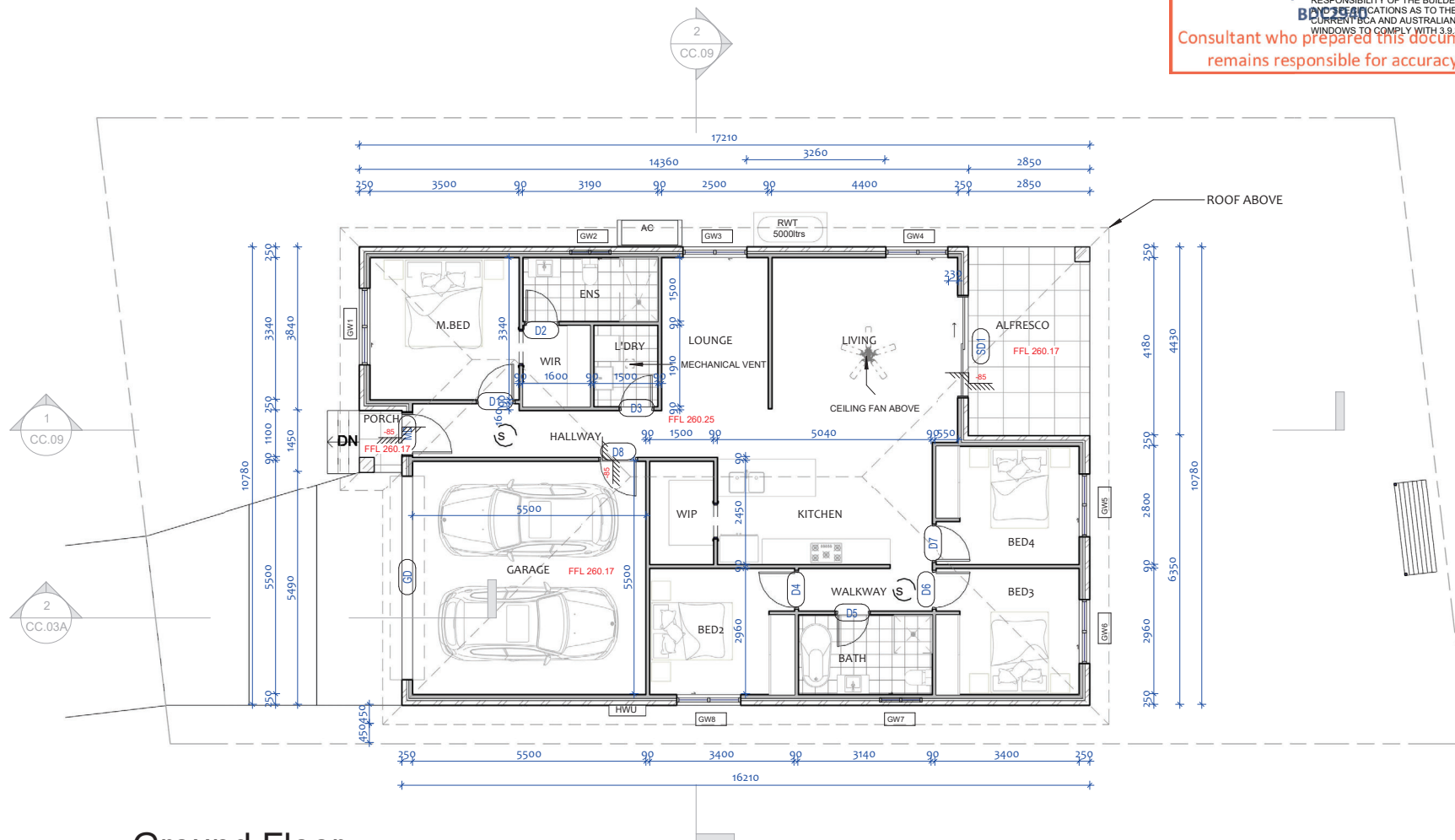
1 Ground Floor 1 : 100
