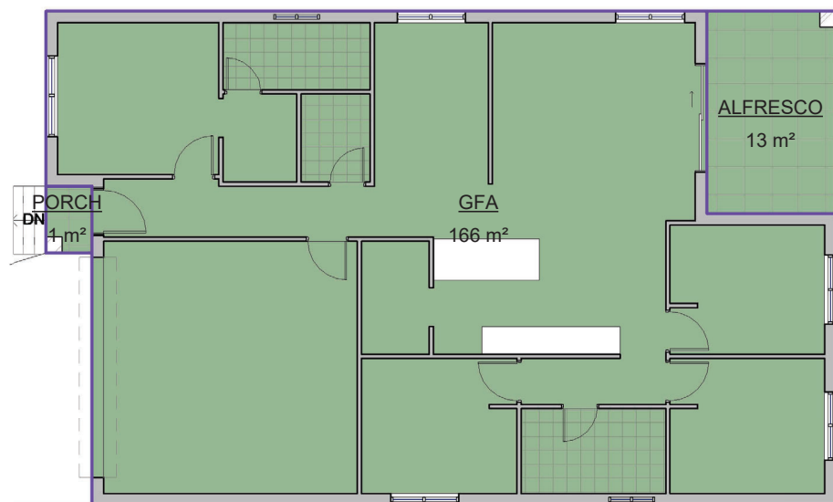
1 Ground Floor 1 : 100
