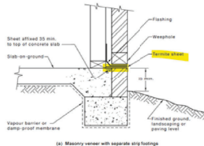
FIGURE 5.5 (in part) TYPICAL SHEET INSTALLATION TO EXTERNAL WALL WITH CONCRETE FLOORSLAB
