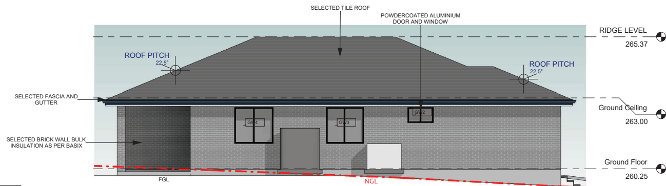
2 North-West Elevation 1 : 100
