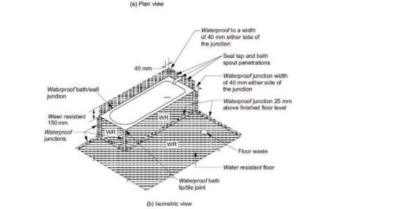
Figure 10.2.4b: Areas adjacent to baths and spas without showers for timber floors including particle-board, plywood and other floor materials
