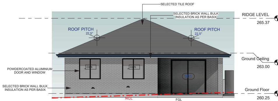
2 North-East Elevation 1 : 100
