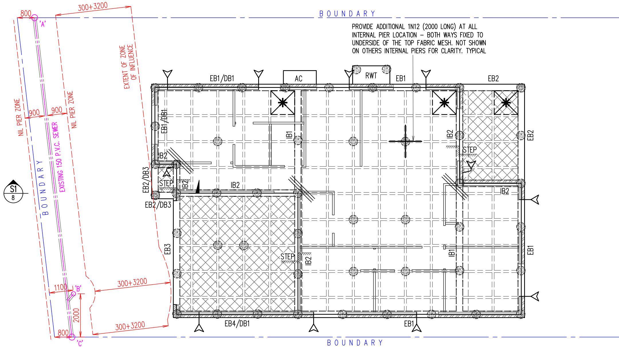
GROUND FLOOR WAFFLE SLAB LAYOUT PLAN SCALE 1:100
