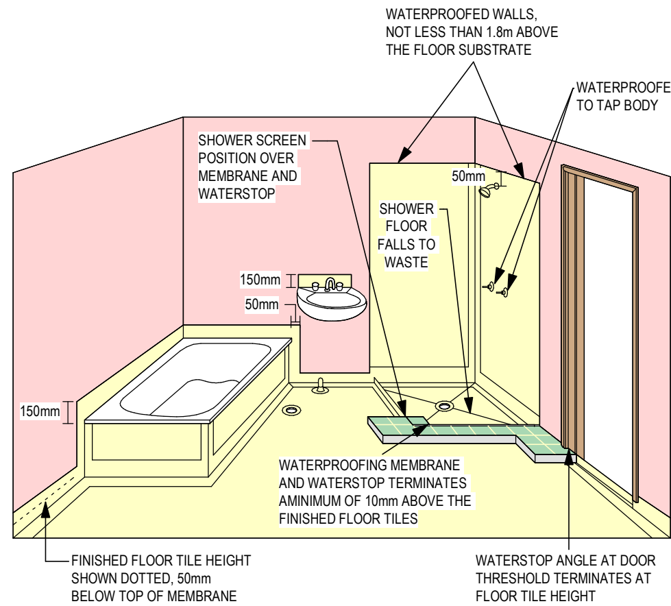
C03 WATERPROOFING DETAILS AROUND BATHROOM
