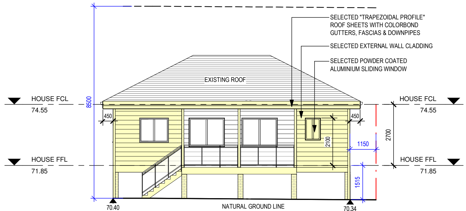
3 SOUTH ELEVATION 1 : 100
