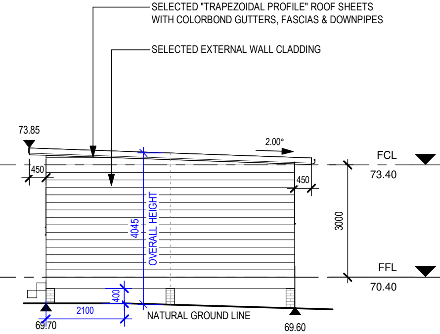
2 WEST ELEVATION 1 : 100
