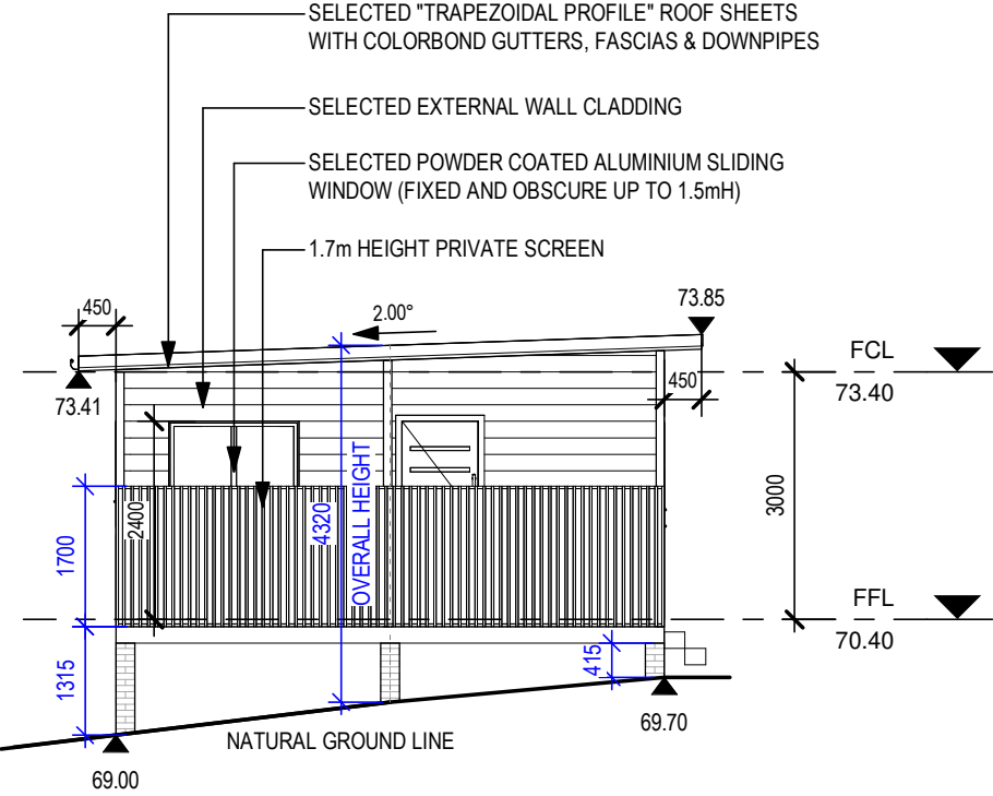
1 EAST ELEVATION 1 : 100
