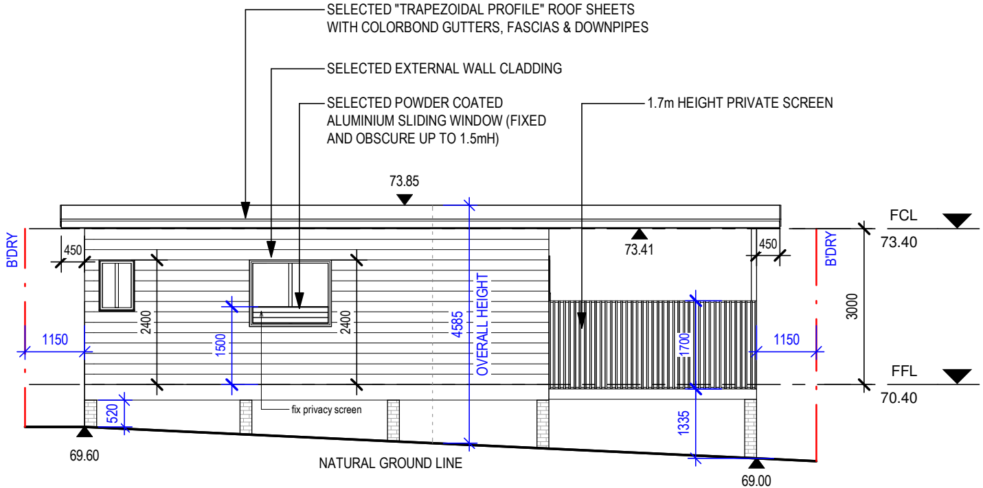
4 SOUTH ELEVATION 1 : 100
