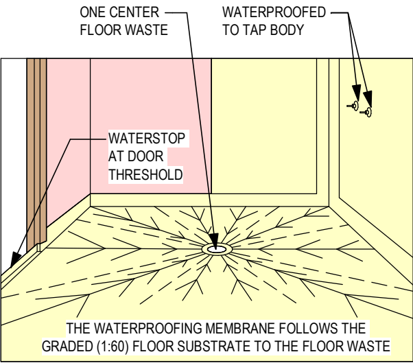
C01 CROSS FALL TO FLOOR WASTE
