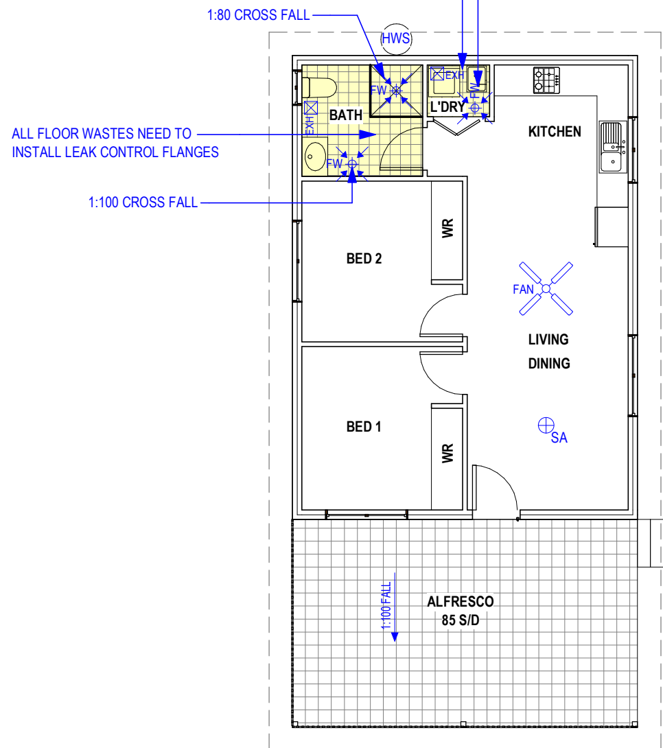
1 WET AREAS PLAN 1 : 100
