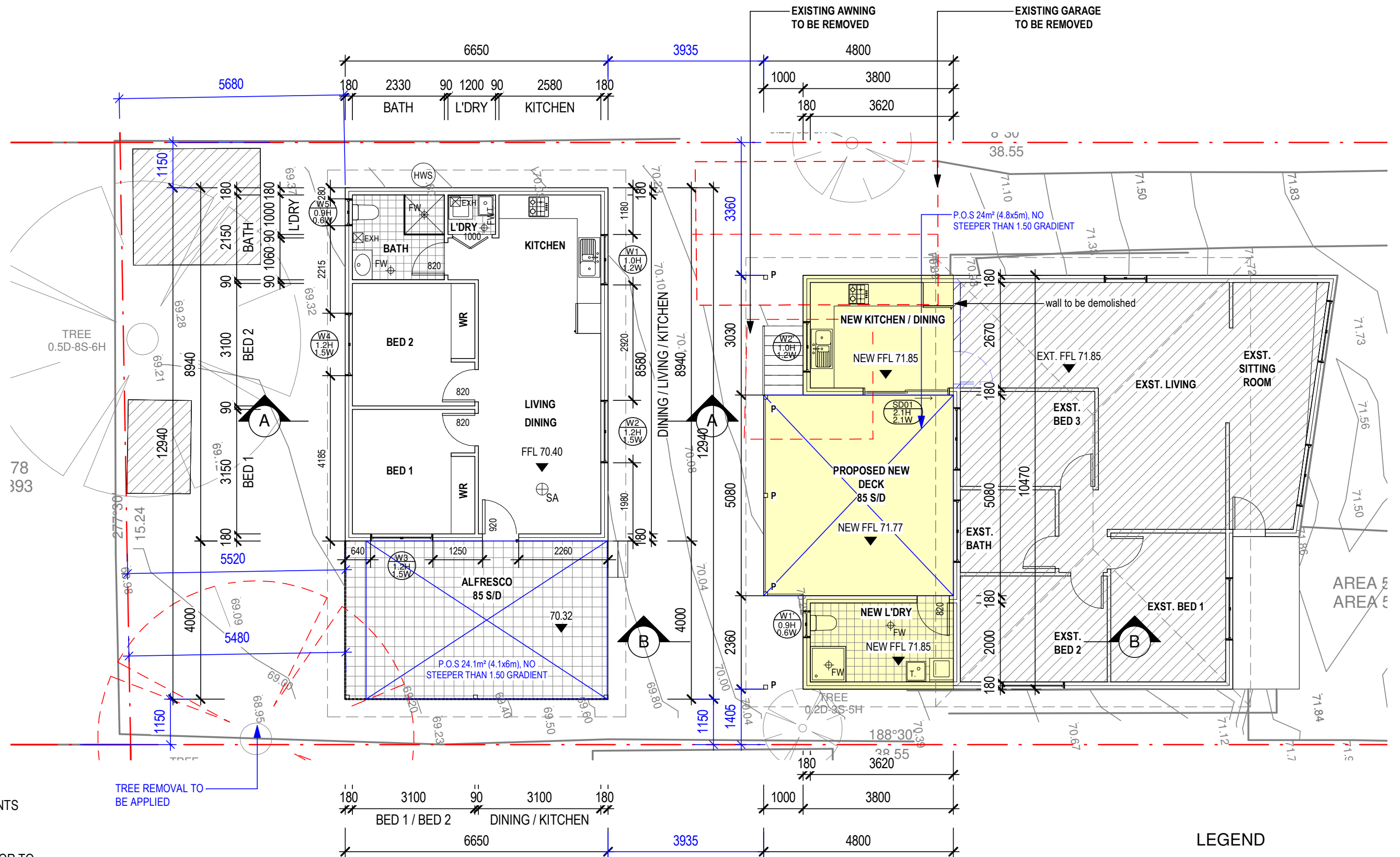
1 PROPOSED GROUND FLOOR PLAN 1 : 100
