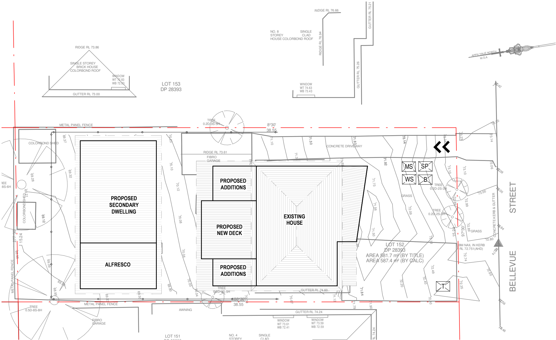
1 EROSION AND SEDIMENT CONTROL PLAN 1 : 200
