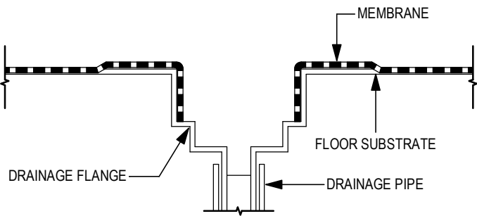
TYPICAL MEMBRANE TERMINATION AT DRAINAGE OUTLET NOT TO SCALE
