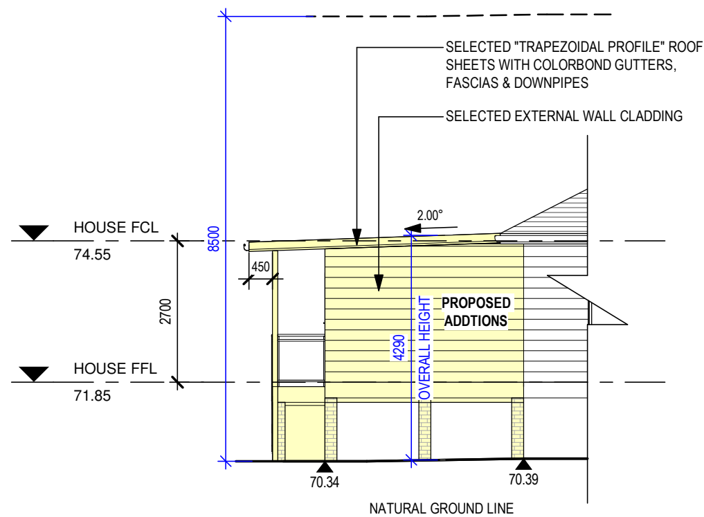
1 EAST ELEVATION 1 : 100
