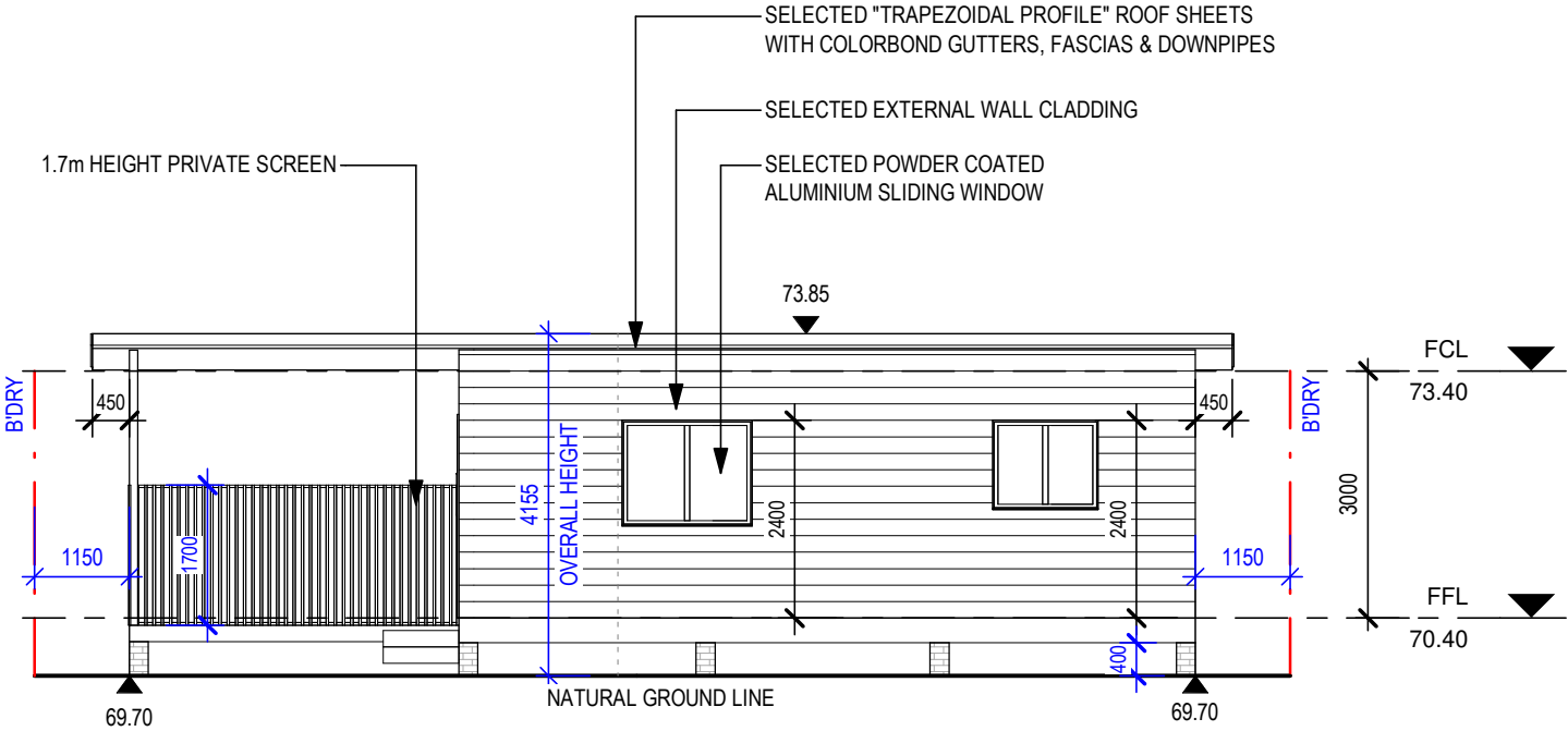
3 NORTH ELEVATION 1 : 100
