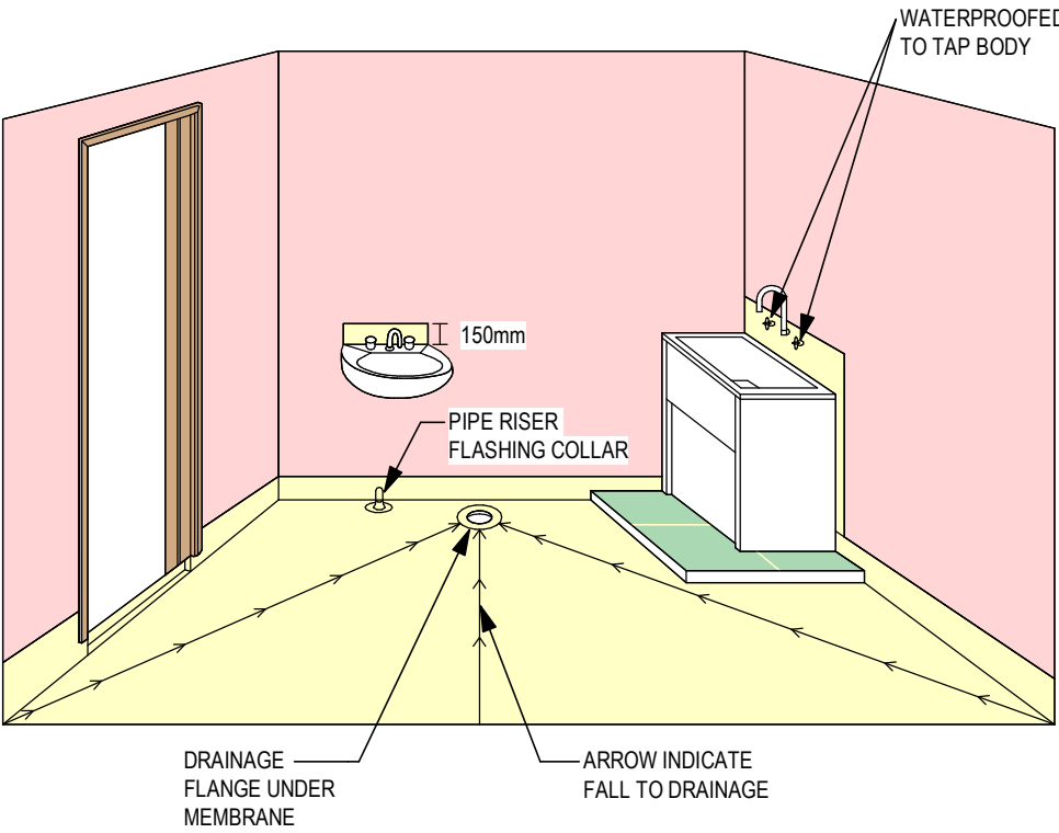
C04 WATERPROOFING DETAILS AROUND LAUNDRY
