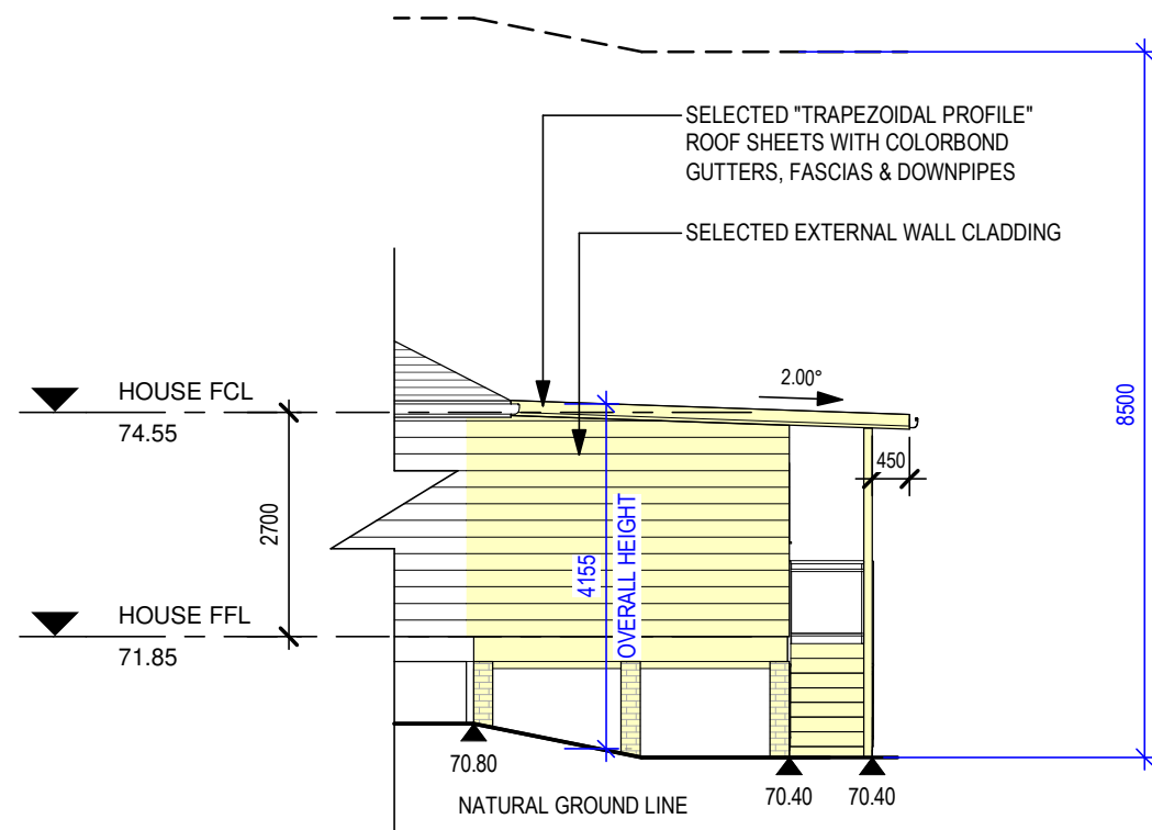
2 WEST ELEVATION 1 : 100
