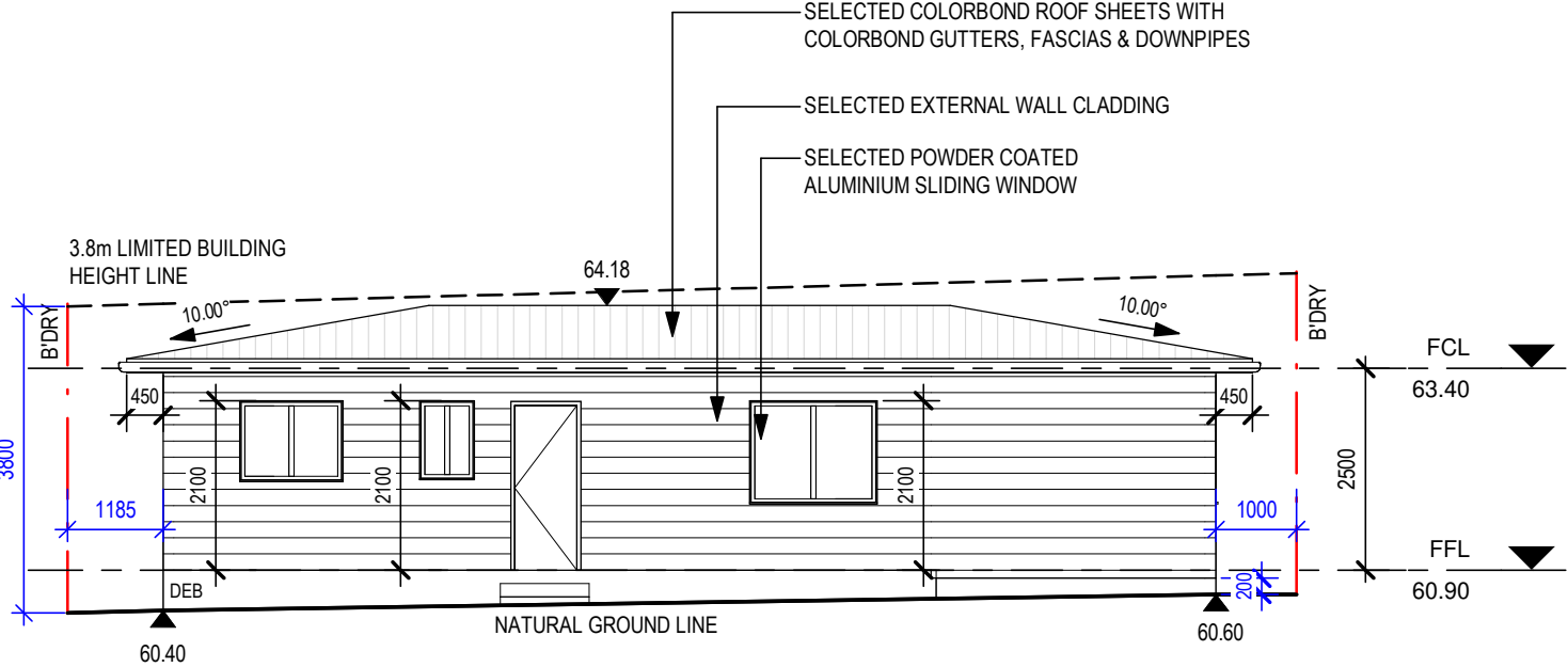
2 SOUTH ELEVATION 1 : 100
