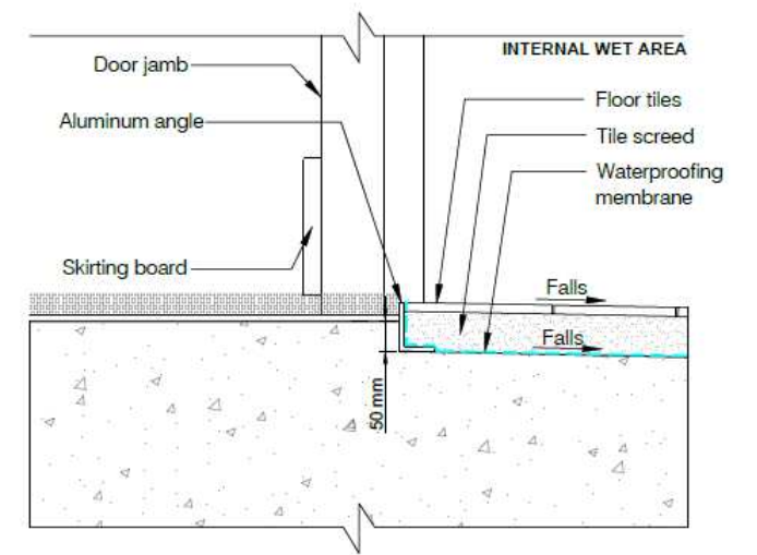
INTERNAL WET AREA DOOR THRESHOLD
