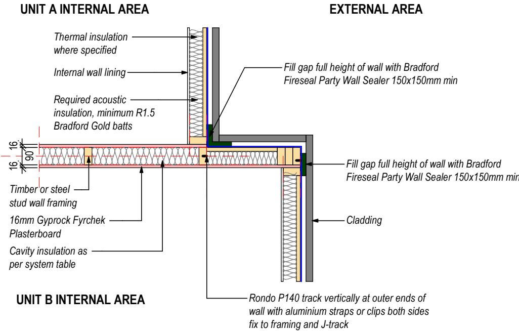
C03 JUNCTION OF PARTY WALL AND EXTERNAL WALL WITH CLADDING AT WALL RETURN - PLAN VIEW
