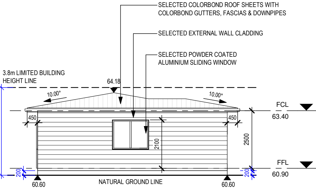
3 EAST ELEVATION 1 : 100
