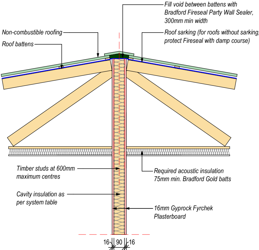
C01 PARTY WALL PERPENDICULAR TO TRUSS/RAFTER (SIDE ELEVATION)
