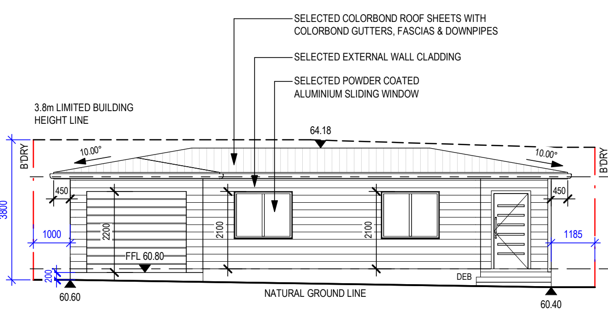
1 NORTH ELEVATION 1 : 100
