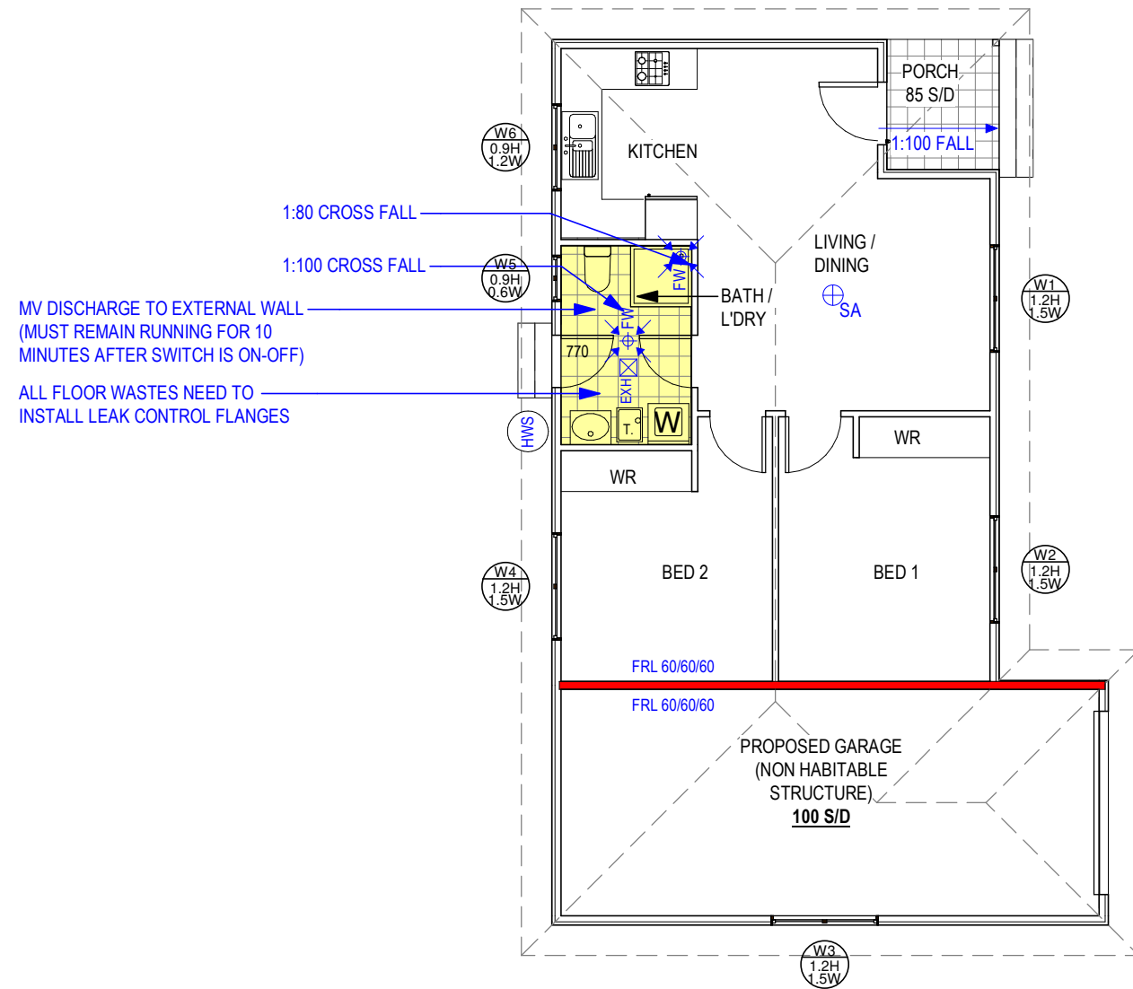
1 WET AREAS PLAN 1 : 100
