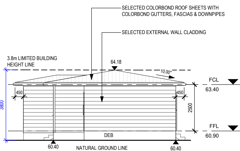
4 WEST ELEVATION 1 : 100
