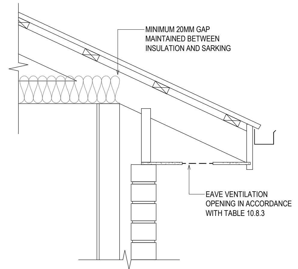
CONDENSATION MANAGEMENT DETAILS
