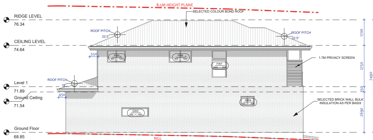
1 WEST ELEVATION 1 : 100
