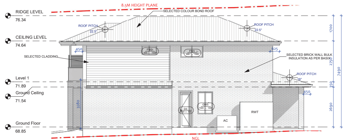
2 EAST ELEVATION 1 : 100
