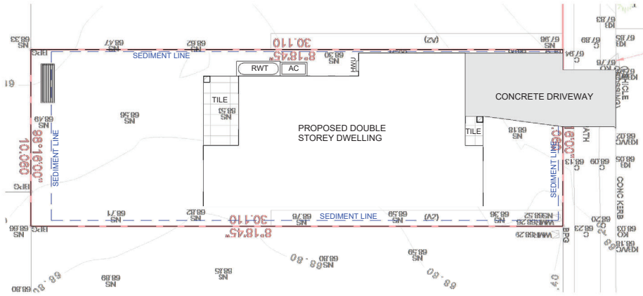
CDC - SITE ANALYSIS AND SEDIMENT CONTROL PLAN
