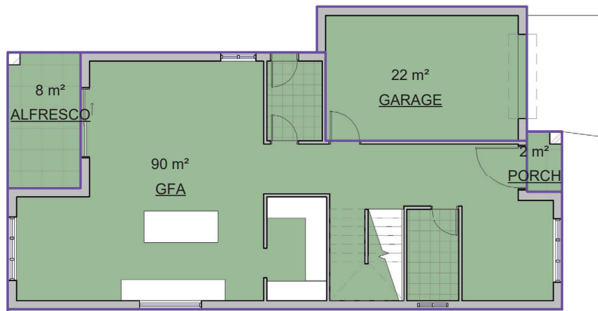
1 Ground Floor 1 : 100
