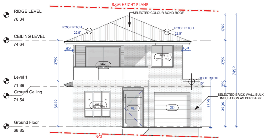
1 SOUTH ELEVATION 1 : 100
