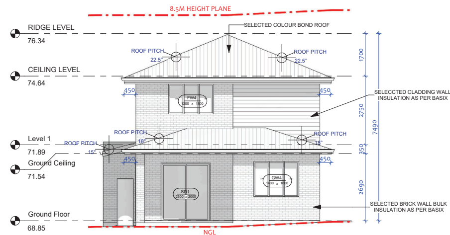
2 NORTH ELEVATION 1 : 100
