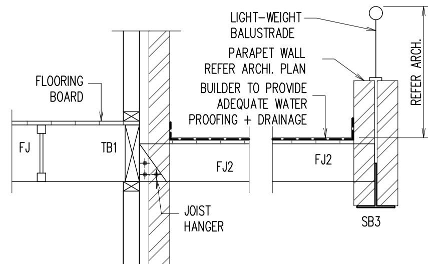
SECTION 5 SCALE 1:20
