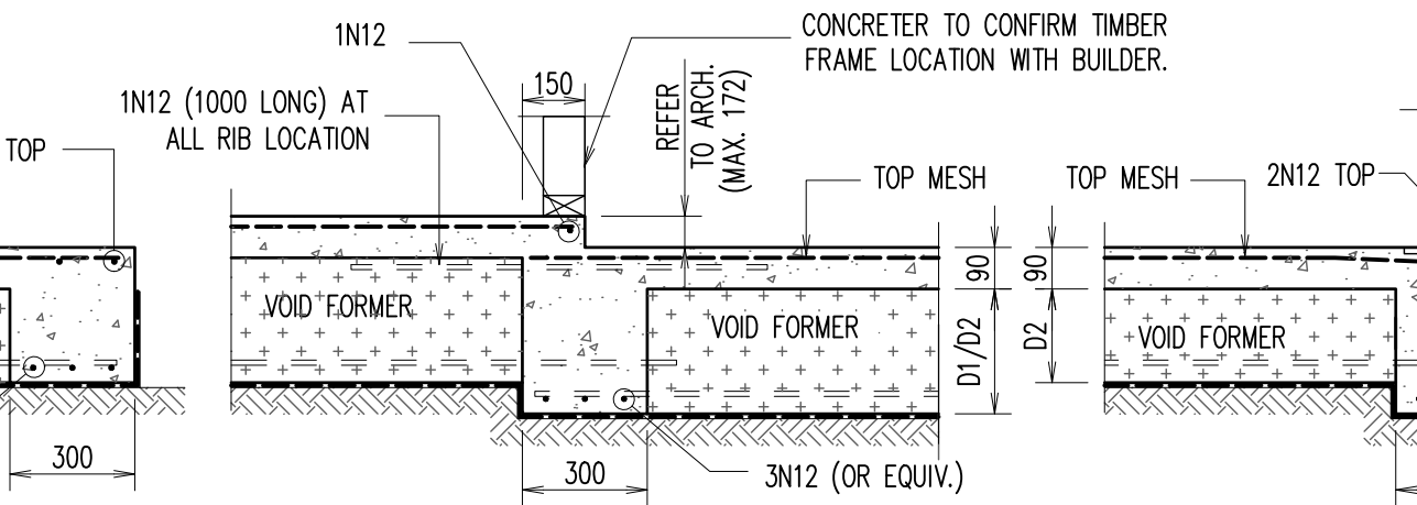
INTERNAL STEPDOWN BEAM - 'IB3' ALTERNATIVELY REFER TO 'DB2' FOR DETAILS
