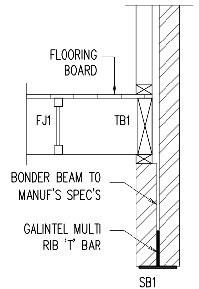
SECTION 4 SCALE 1:20
