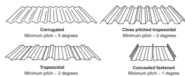
Figure 7.2.3: Minimum pitch requirements for metal roofing profiles
