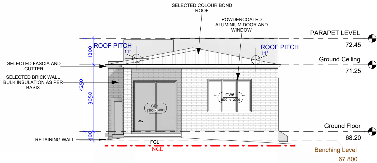
NORTH Elevation
