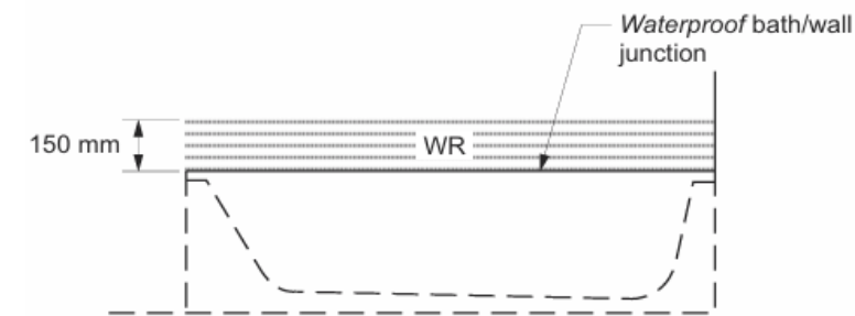
(b) Wall/bath junction
