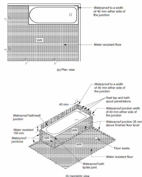
Figure 10.2.4b: Areas adjacent to baths and spas without showers for timber floors including particle-board, plywood and other floor materials
