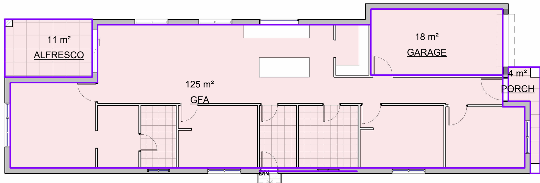
1 Ground Floor 1 : 100
