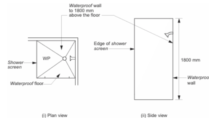
(a) Enclosed shower
