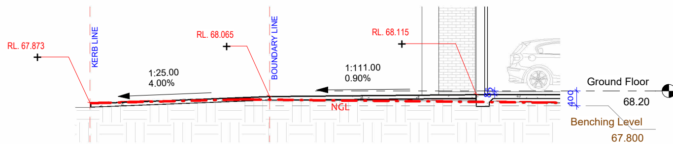
DRIVEWAY SECTION
