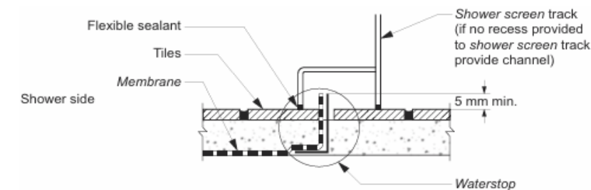
Figure 10.2.17: Typical hobless construction
