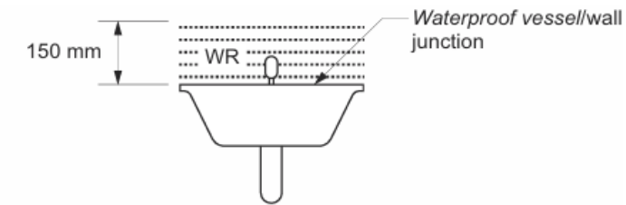
(a) Vessel abutting wall
