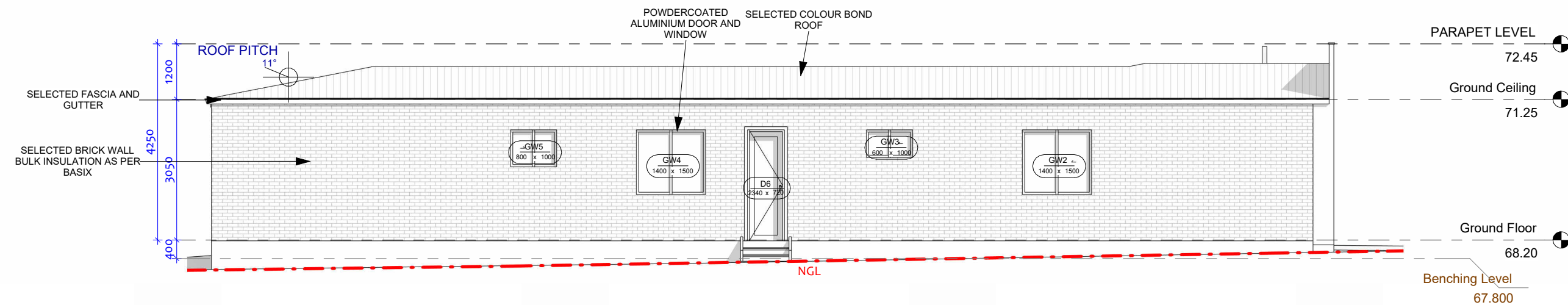
2 WEST Elevation 1 : 100
