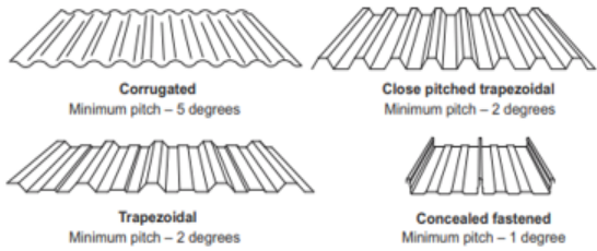
Figure 7.2.3: Minimum pitch requirements for metal roofing profiles
