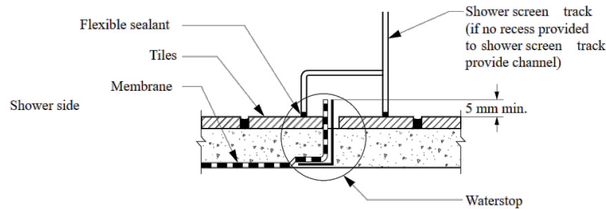
Figure 10.2.16: Typical hob construction — internal membrane
