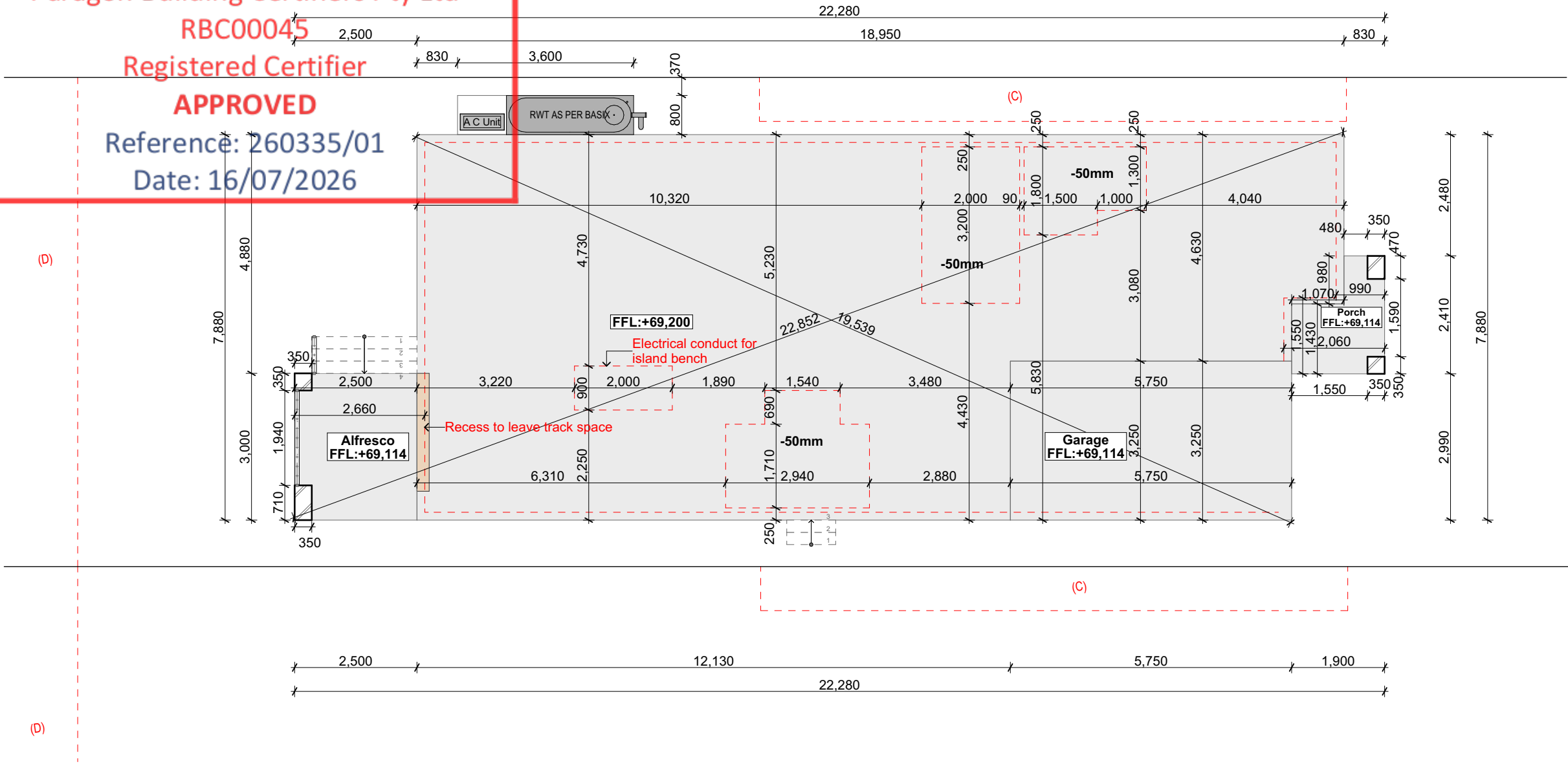
Slab Plan 1:100
