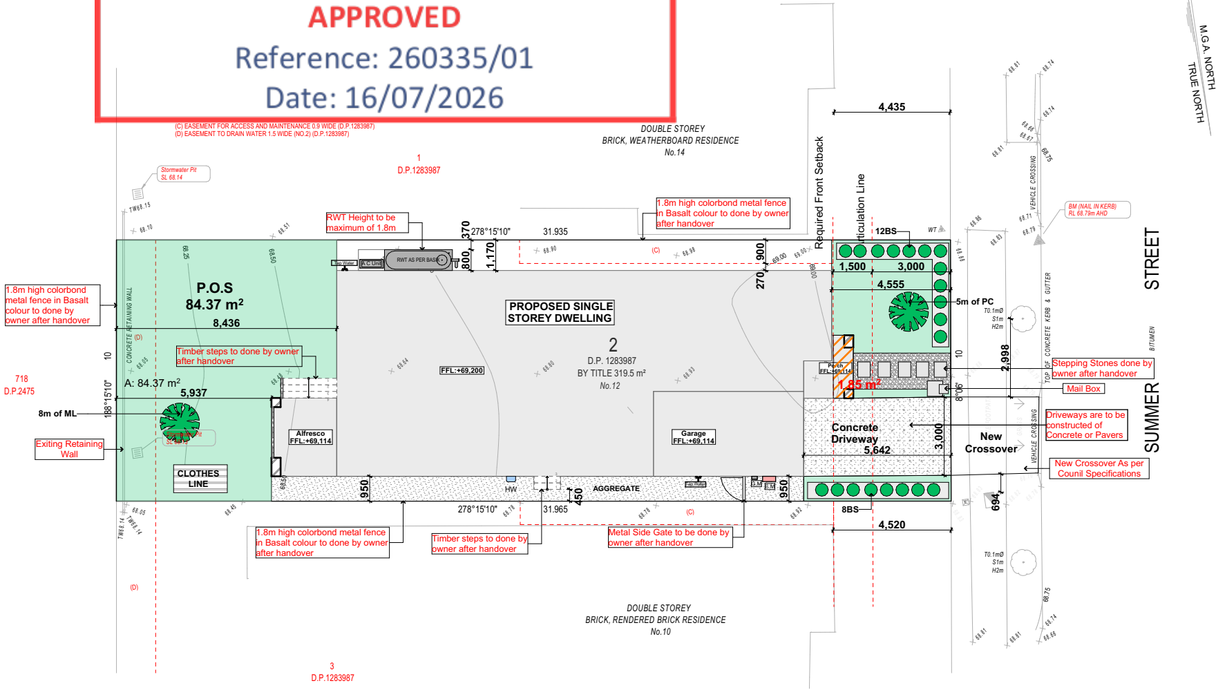
Landscape Plan 1:200
