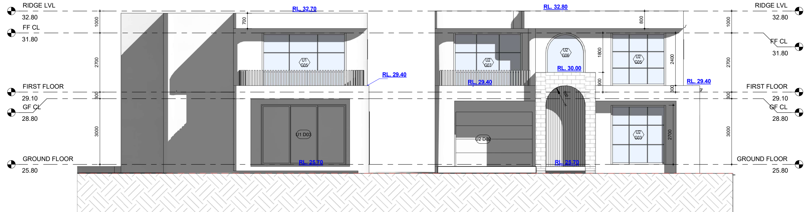
EAST ELEVATION
