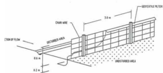
SEDIMENT FENCE NTS
