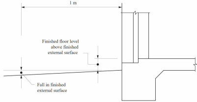
Figure 1.3.3a for surface drainage
