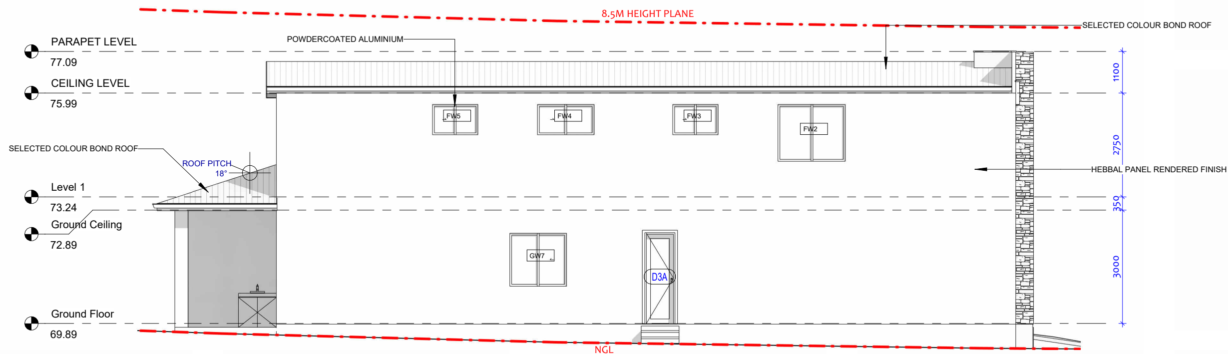
2 North Elevation 1 : 100
