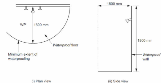
(b) Unenclosed shower
