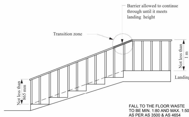
Figure 11.3.4b Measuring heights for barriers and handrails and where transition zones are allowed
