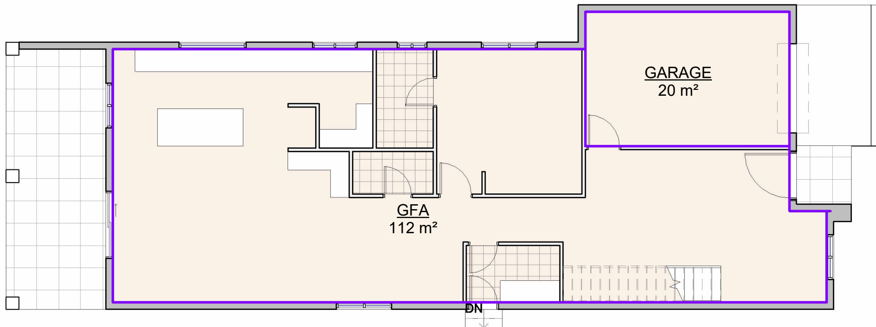
1 Ground Floor 1 : 100
