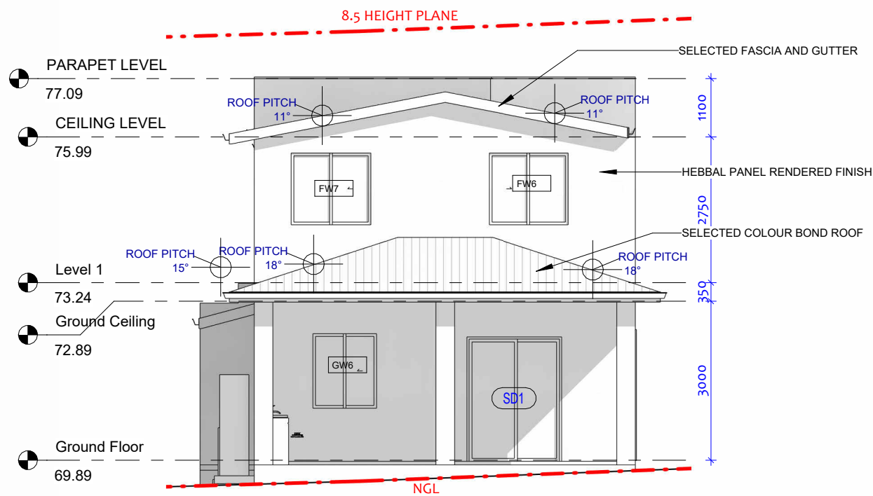
2 West Elevation 1 : 100
