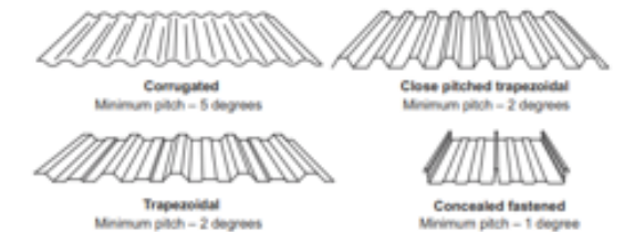
Figure 7.2.3: Minimum pitch requirements for metal roofing profiles
