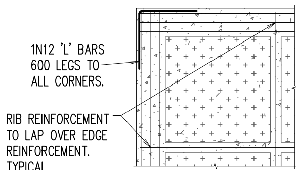
TYPICAL CORNER DETAILS
