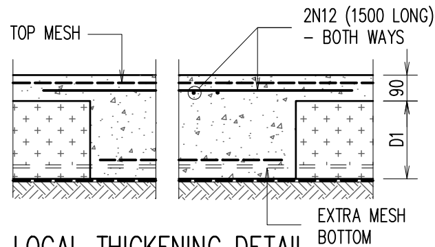
LOCAL THICKENING DETAIL
