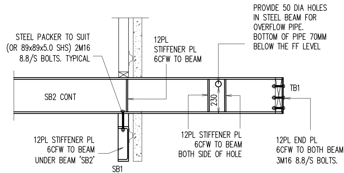
DETAIL - A
