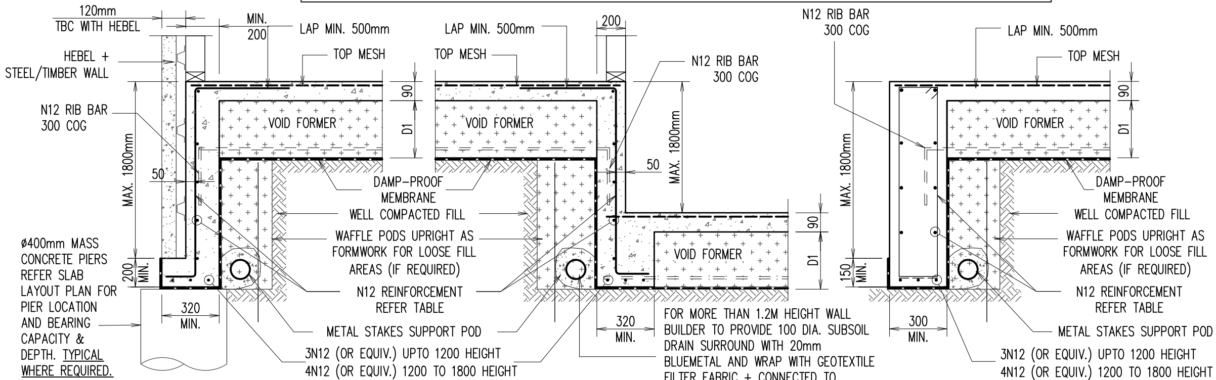
'EXTERNAL' DROP BEAM - 'DB1'
