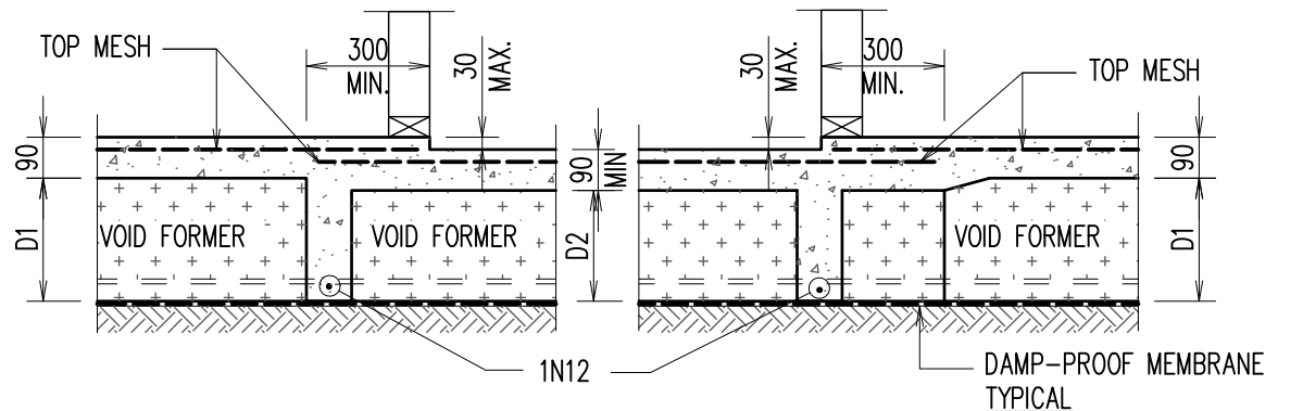
TYPICAL WET AREA STEP DETAIL
