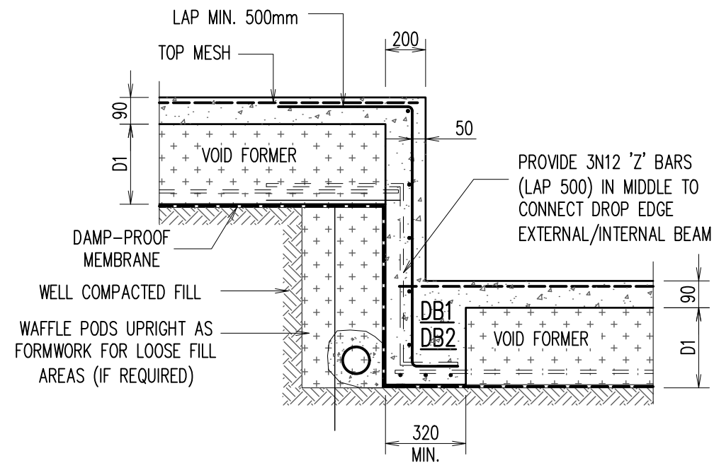
DROP EDGE BEAM TRANSITION DETAIL
