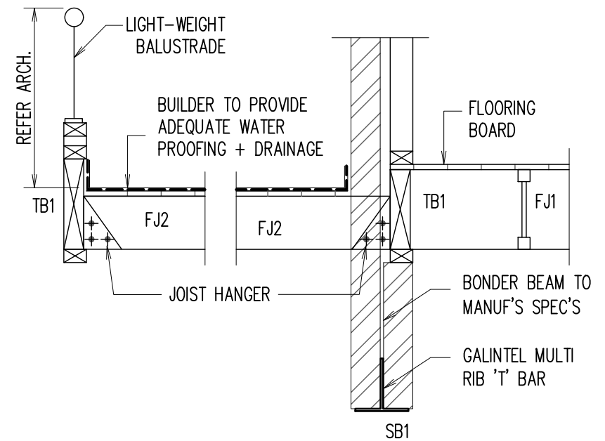
SECTION 3 SCALE 1:20
