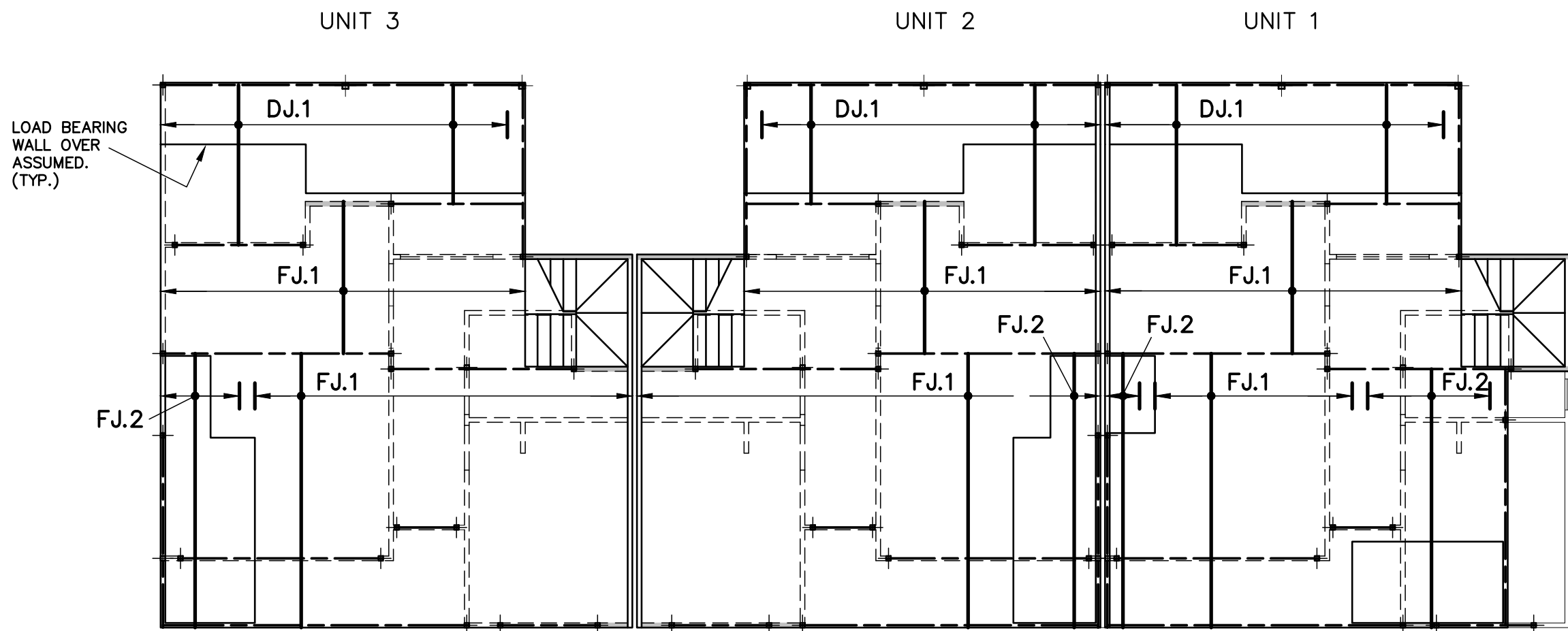
FIRST FLOOR JOIST LAYOUT FOR UNITS 1 – 3 (1:100)
