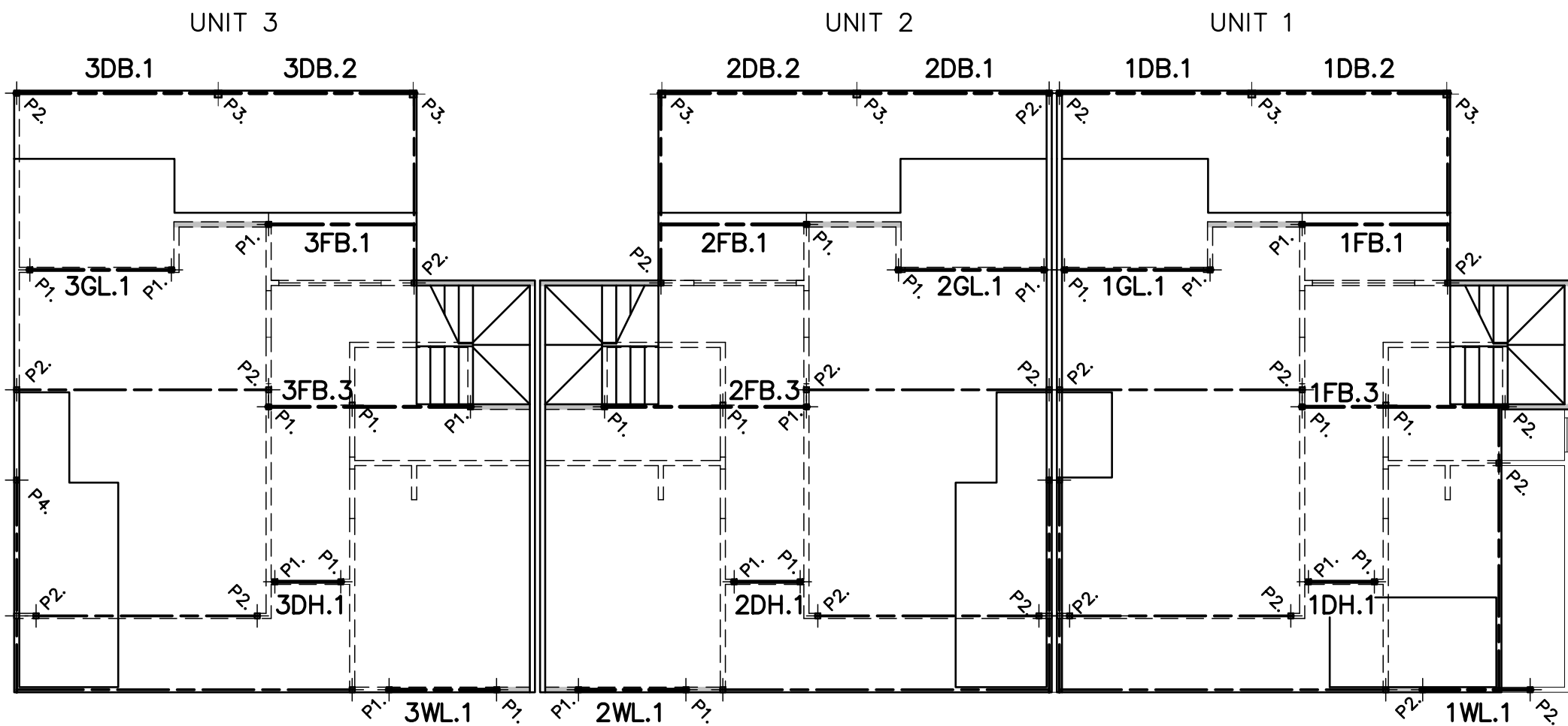
FIRST FLOOR BEAM LAYOUT FOR UNITS 1 – 3 (1:100)
