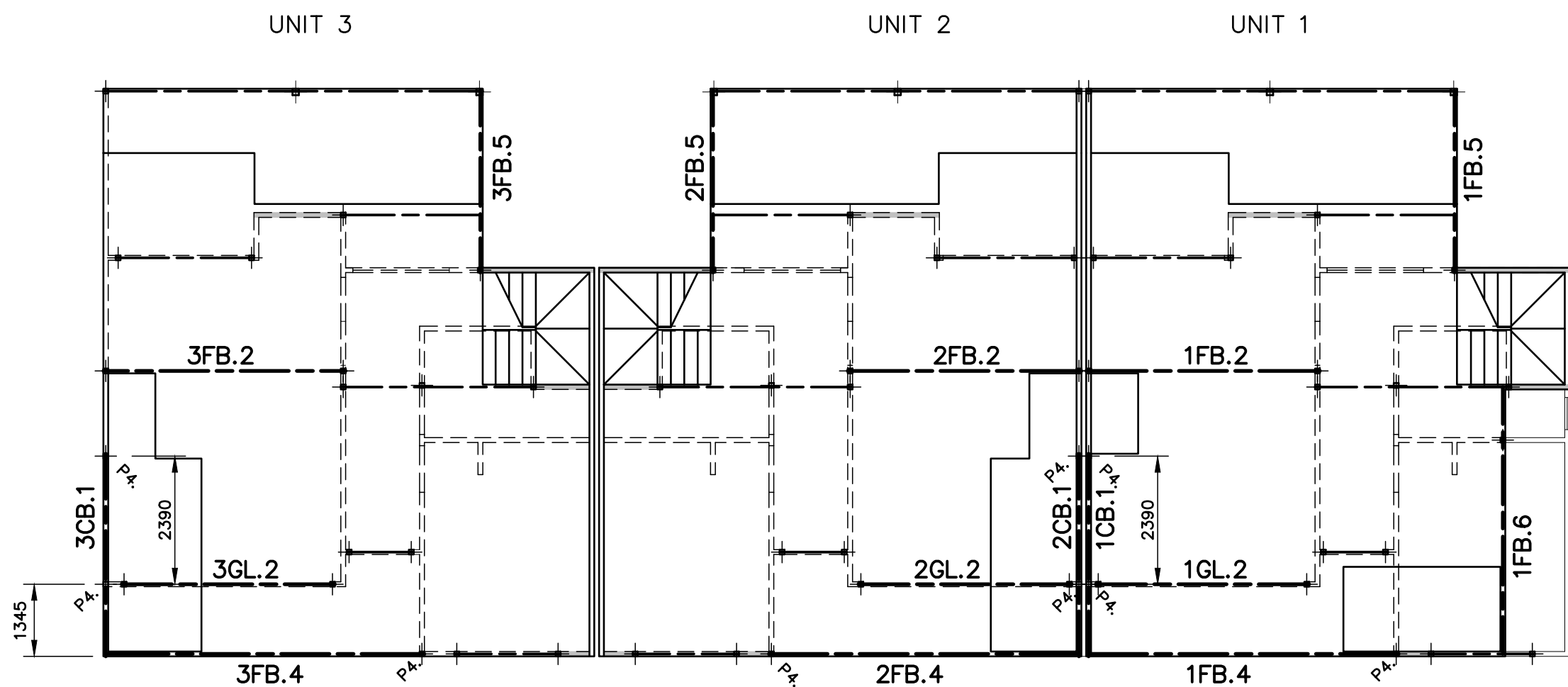
FIRST FLOOR BEAM LAYOUT FOR UNITS 1 – 3 (1:100)
