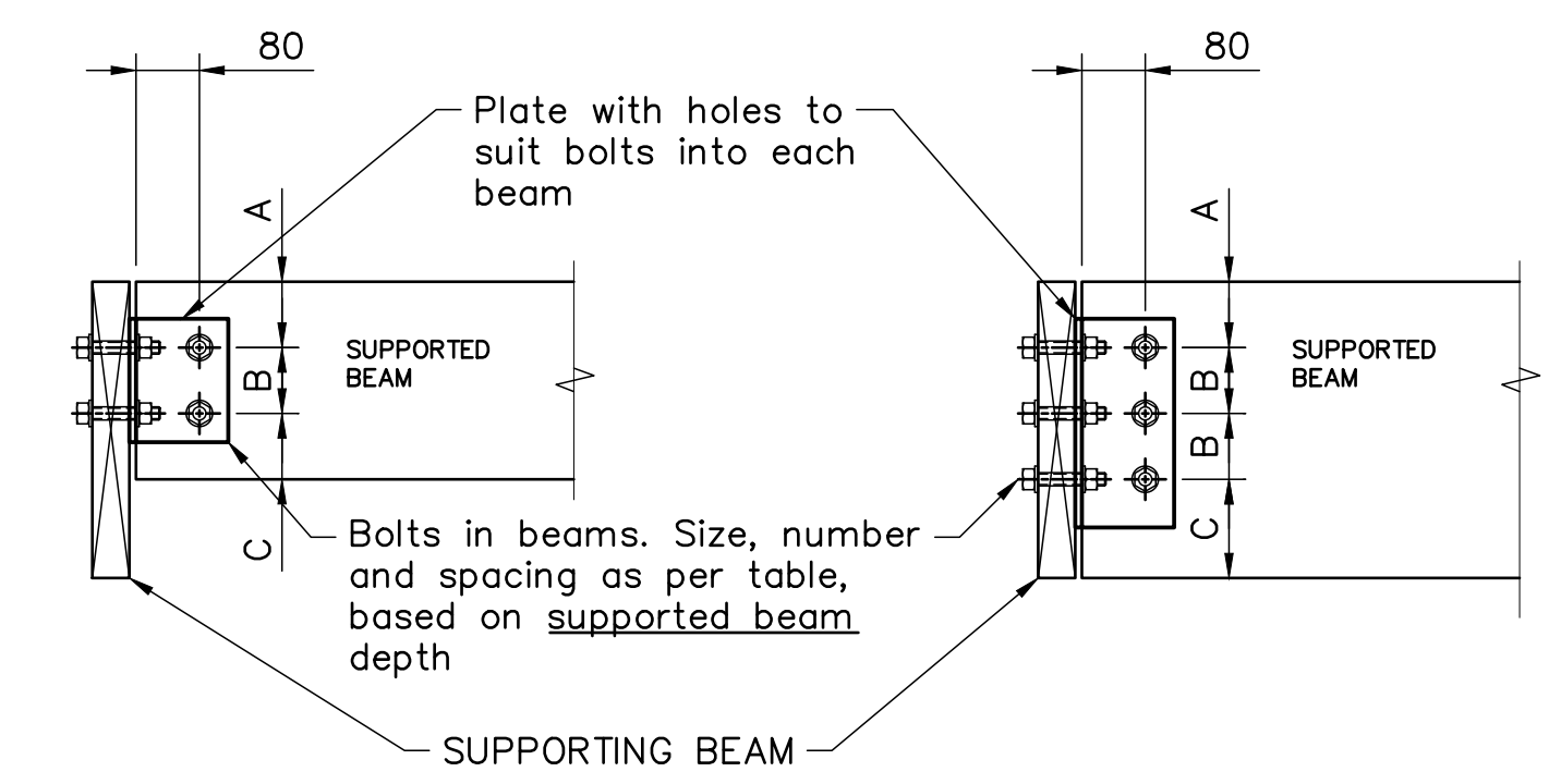
TIMBER BEAM CONNECTION (1:10)
