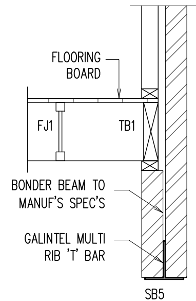
SECTION 5 SCALE 1:20
