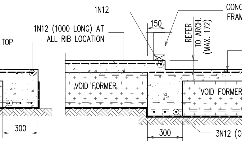
INTERNAL STEPDOWN BEAM – 'IB3'
