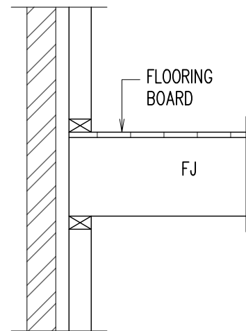
SECTION 1 SCALE 1:20
