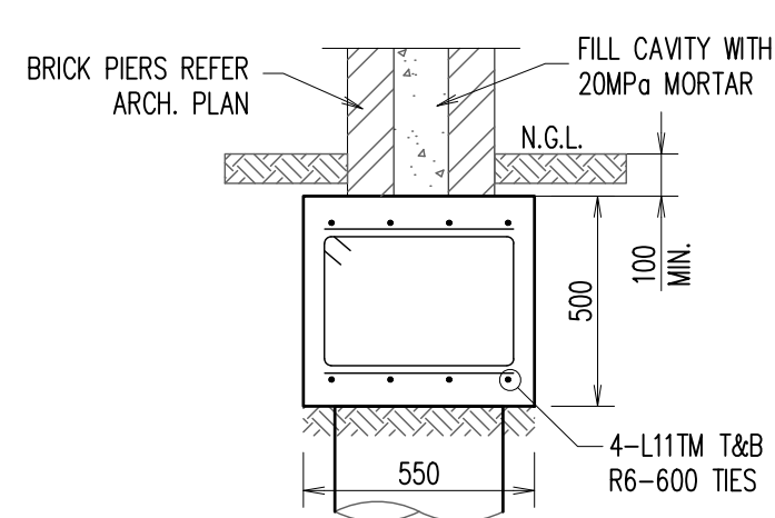
STRIP FOOTING (SF1) DETAILS
