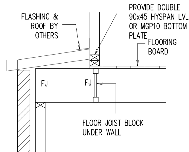
SECTION 3 SCALE 1:20
