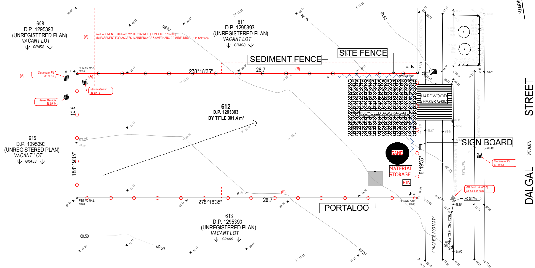
Sediment Control Plan 1:200
