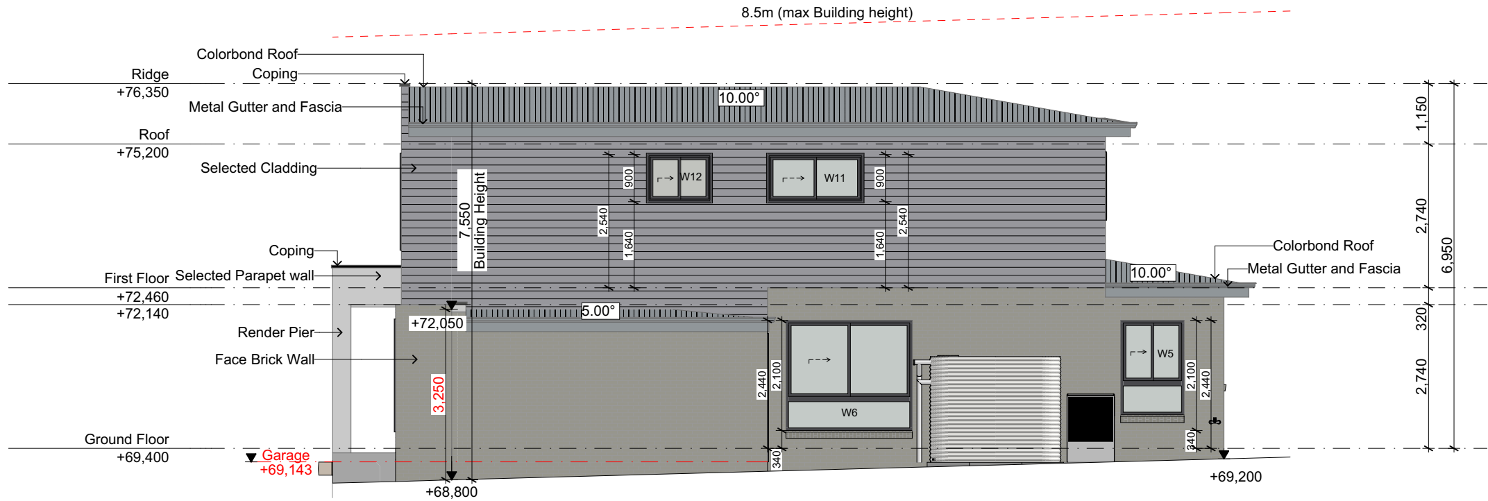
4 North Elevation (Right Side) 1:100
