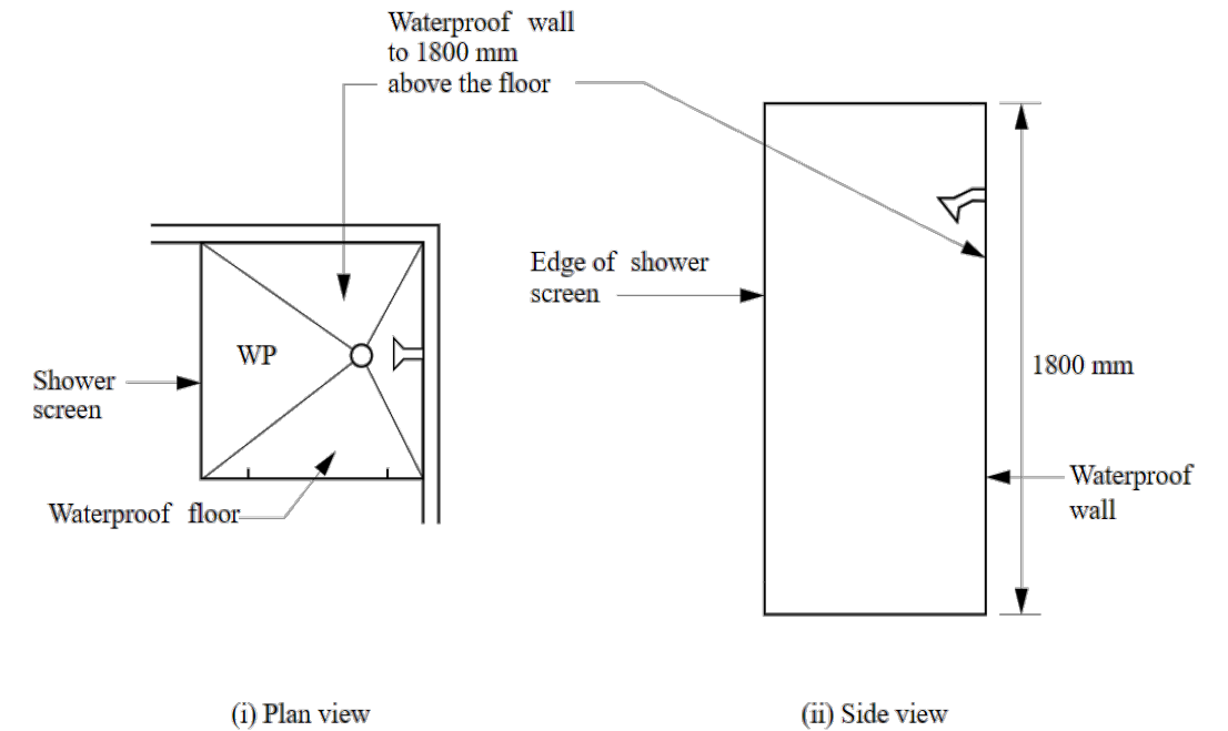
(a) Enclosed shower
