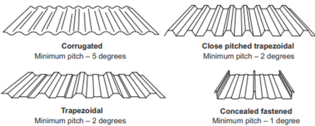
Figure 7.2.3: Minimum pitch requirements for metal roofing profiles
