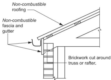
(b) Gutter on face of wall
